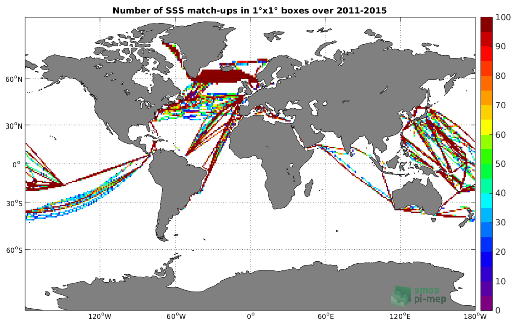
Figure 4: Number of SSS match-ups between TSG-LEGOS-DM SSS and the Aquarius-L3-OR-V5-MONTHLY-1DEG SSS product for the Global Ocean Pi-MEP region over 1^\circ \times 1^\circ boxes and for the full satellite product period.
