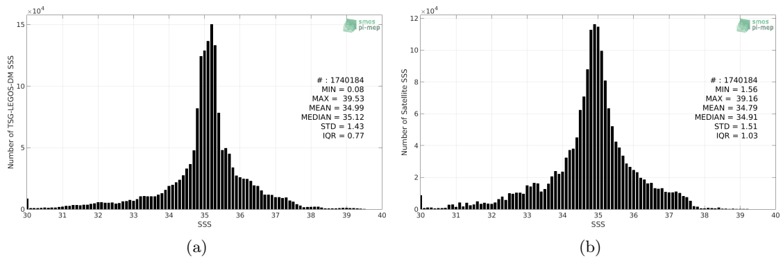
Figure 2: Histograms of SSS from TSG-LEGOS-DM (a) and Aquarius-L3-OR-V5-MONTHLY-1DEG (b) considering all match-up pairs per bins of 0.1 over the Global Ocean Pi-MEP region and for the full satellite product period.
