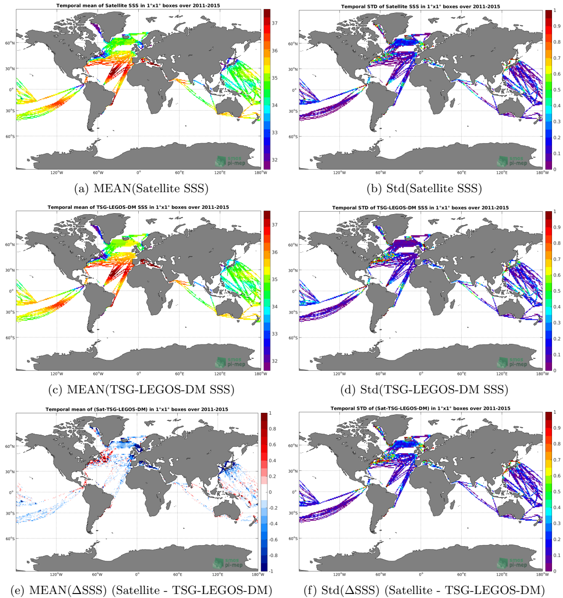
Figure 6: Temporal mean (left) and Std (right) of SSS from Aquarius-L3-OR-V5-MONTHLY-1DEG (top), TSG-LEGOS-DM (middle), and of \Delta SSS (Satellite - TSG-LEGOS-DM). Only match-up pairs are used to generate these maps.
