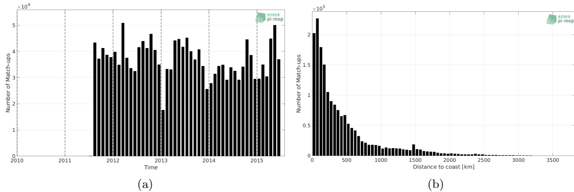
Figure 1: Number of match-ups between TSG-LEGOS-DM and Aquarius-L3-OR-V5-MONTHLY-1DEG SSS as a function of time (a) and as function of the distance to coast (b) over the Global Ocean Pi-MEP region and for the full satellite product period.
