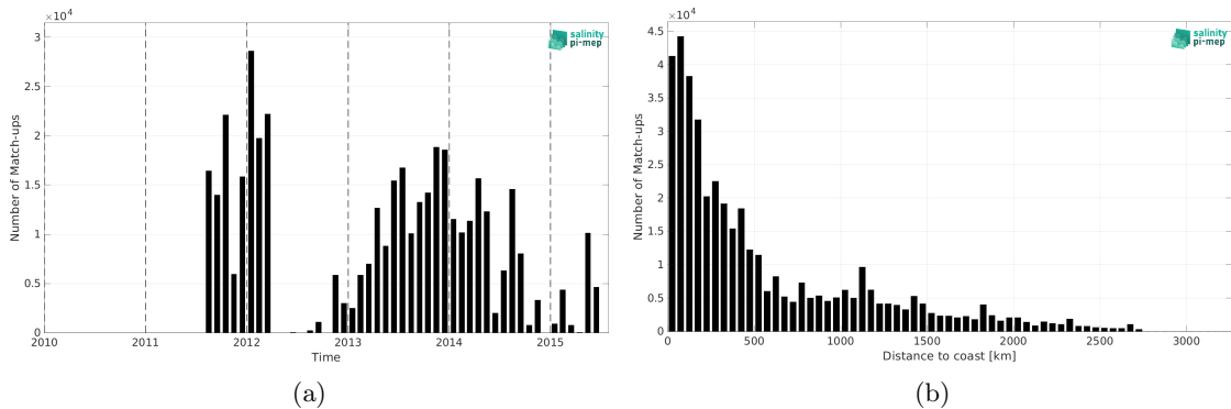
Figure 2: Number of match-ups between TSG (GOSUD-Sailing-ship) and Aquarius SSS L3 OR v5 - Monthly (NASA-GSFC) SSS as a function of time (a) and as function of the distance to coast (b) over the Global Ocean Pi-MEP region and for the full satellite product period.
