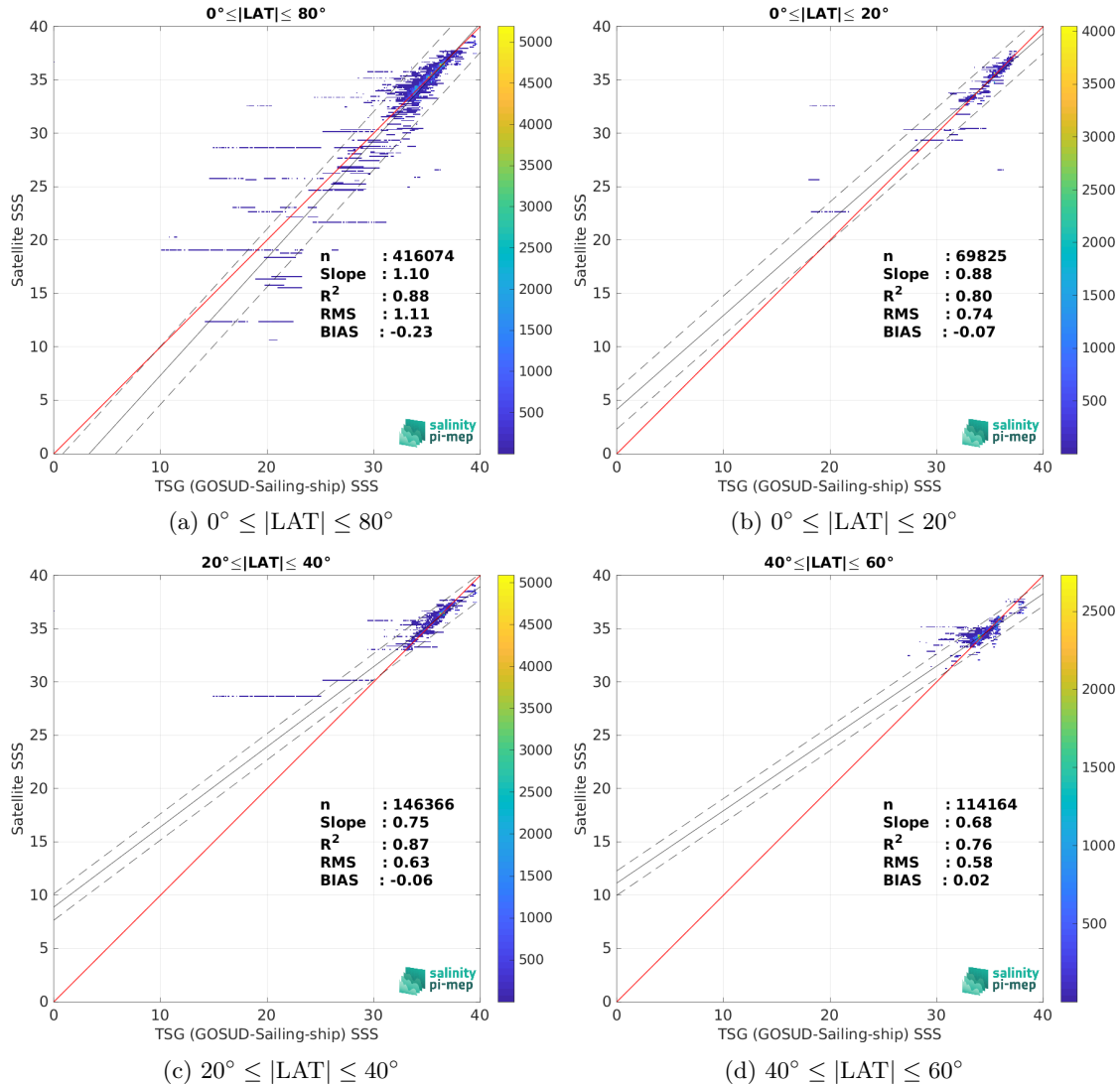
Figure 10: Contour maps of the concentration of Aquarius SSS L3 OR v5 - Monthly (NASA-GSFC) SSS (y-axis) versus TSG (GOSUD-Sailing-ship) SSS (x-axis) at match-up pairs for different latitude bands. For each plot, the red line shows x=y . The black thin and dashed lines indicate a linear fit through the data cloud and the \pm 95\% confidence levels, respectively. The number match-up pairs n , the slope and R^2 coefficient of the linear fit, the root mean square (RMS) and the mean bias between satellite and in situ data are indicated for each latitude band in each plots.
