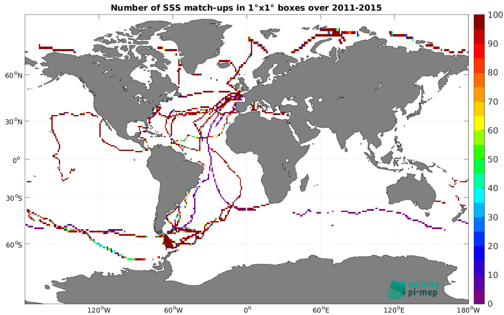
Figure 5: Number of SSS match-ups between TSG (GOSUD-Sailing-ship) SSS and the Aquarius SSS L3 OR v5 - Monthly (NASA-GSFC) SSS product for the Global Ocean Pi-MEP region over 1^\circ \times 1^\circ boxes and for the full satellite product period.
