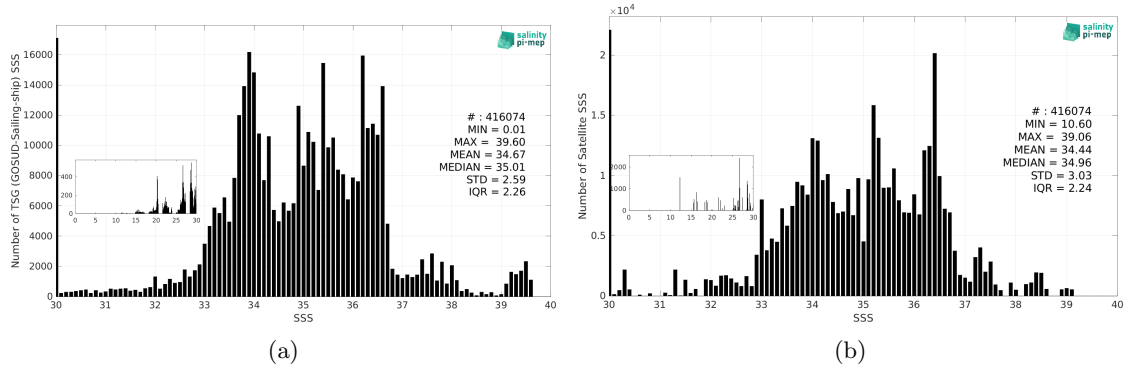
Figure 3: Histograms of SSS from TSG (GOSUD-Sailing-ship) (a) and Aquarius SSS L3 OR v5 - Monthly (NASA-GSFC) (b) considering all match-up pairs per bins of 0.1 over the Global Ocean Pi-MEP region and for the full satellite product period.
