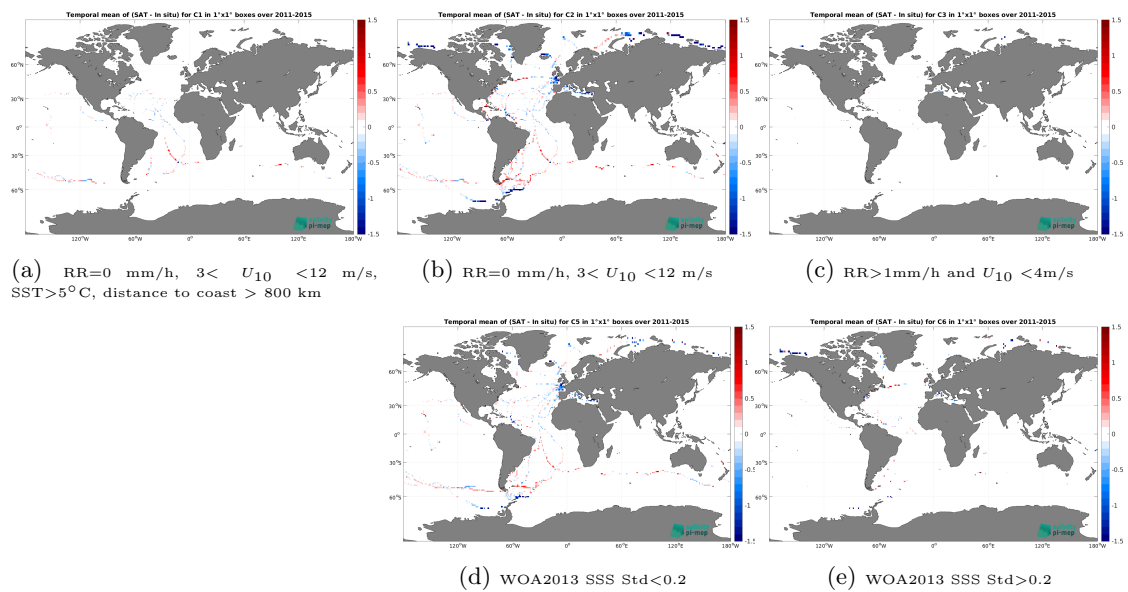
Figure 14: Temporal mean gridded over spatial boxes of size 1^\circ \times 1^\circ of \Delta SSS (Aquarius SSS L3 OR v5 - Monthly (NASA-GSFC) - TSG (GOSUD-Sailing-ship)) for 5 different subdatasets corresponding to:RR=0 mm/h, 3 < U_{10} < 12 m/s, SST > 5^\circ\text{C} , distance to coast > 800 km (a), RR=0 mm/h, 3 < U_{10} < 12 m/s (b), RR > 1 mm/h and U_{10} < 4 m/s (c), WOA2013 SSS Std < 0.2 (d), WOA2013 SSS Std > 0.2 (e).
