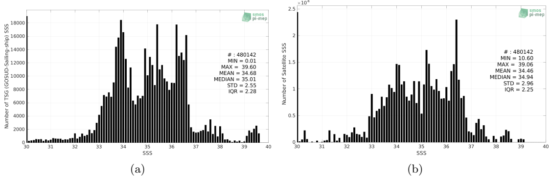
Figure 2: Histograms of SSS from TSG (GOSUD-Sailing-ship) (a) and Aquarius SSS L3 OR v5 - Monthly (NASA-GSFC) (b) considering all match-up pairs per bins of 0.1 over the Global Ocean Pi-MEP region and for the full satellite product period.
