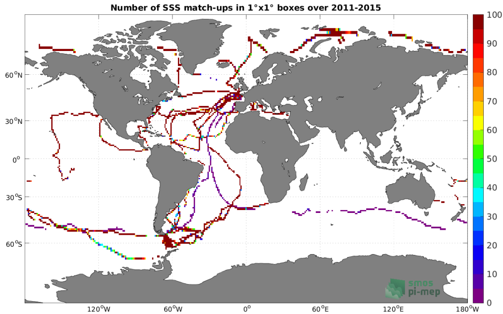
Figure 4: Number of SSS match-ups between TSG (GOSUD-Sailing-ship) SSS and the Aquarius SSS L3 OR v5 - Monthly (NASA-GSFC) SSS product for the Global Ocean Pi-MEP region over 1^\circ \times 1^\circ boxes and for the full satellite product period.
