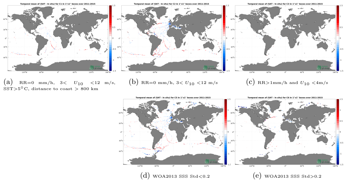
Figure 12: Temporal mean gridded over spatial boxes of size 1^\circ \times 1^\circ of \Delta SSS (Aquarius SSS L3 OR v5 - Monthly (NASA-GSFC) - TSG (GOSUD-Sailing-ship)) for 5 different subdatasets corresponding to: RR=0 mm/h, 3 < U_{10} < 12 m/s, SST > 5°C, distance to coast > 800 km (a), RR=0 mm/h, 3 < U_{10} < 12 m/s (b), RR > 1mm/h and U_{10} < 4 m/s (c), WOA2013 SSS Std < 0.2 (d), WOA2013 SSS Std > 0.2 (e).
