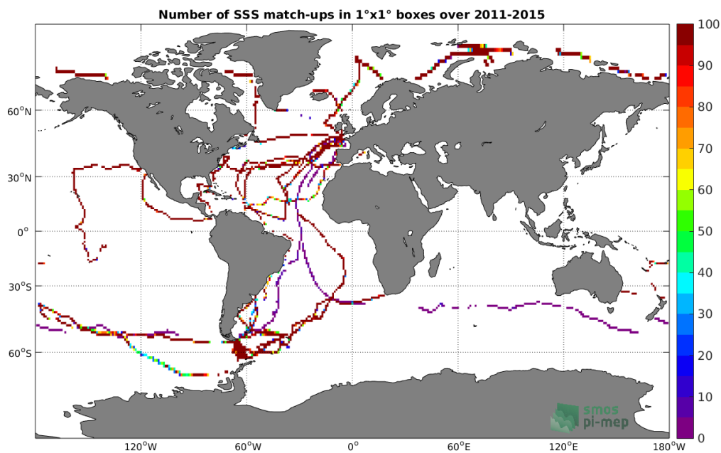
Figure 4: Number of SSS match-ups between TSG-GOSUD-Sailing-ship SSS and the Aquarius-L3-OR-V5-MONTHLY-1DEG SSS product for the Global Ocean Pi-MEP region over 1^\circ \times 1^\circ boxes and for the full satellite product period.
