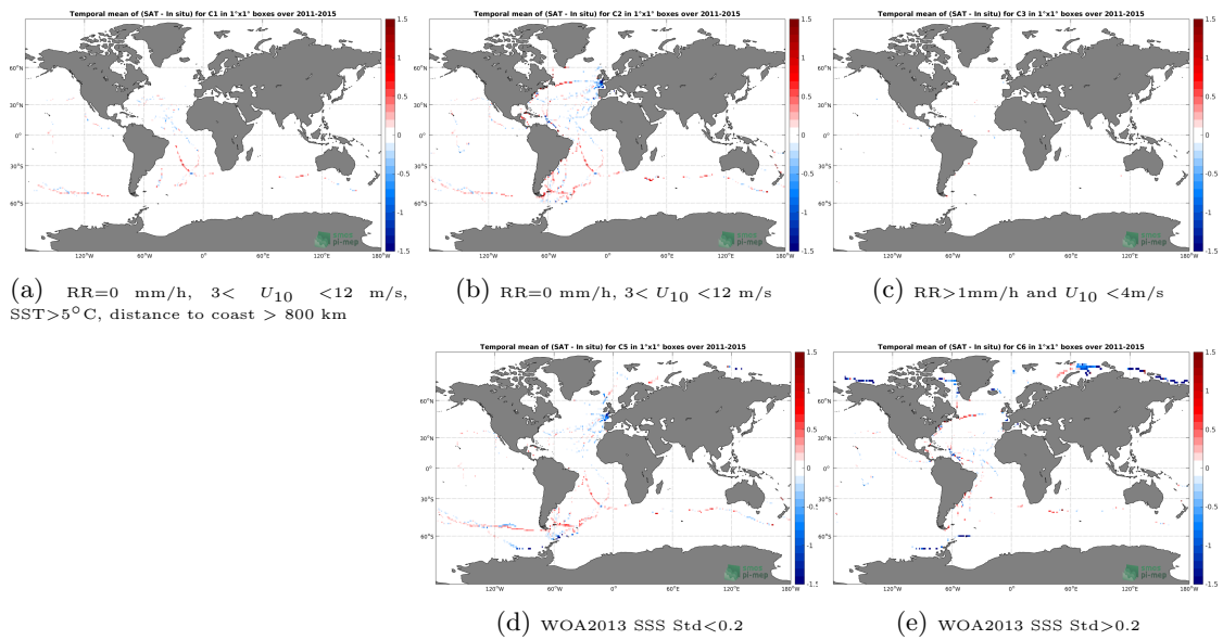
Figure 12: Temporal mean gridded over spatial boxes of size 1^\circ \times 1^\circ of \Delta SSS (Aquarius-L3-OR-V5-MONTHLY-1DEG - TSG-GOSUD-Sailing-ship) for 5 different subdatasets corresponding to: RR=0 mm/h, 3 < U_{10} < 12 m/s, SST > 5°C, distance to coast > 800 km (a), RR=0 mm/h, 3 < U_{10} < 12 m/s (b), RR > 1mm/h and U_{10} < 4 m/s (c), WOA2013 SSS Std < 0.2 (d), WOA2013 SSS Std > 0.2 (e).
