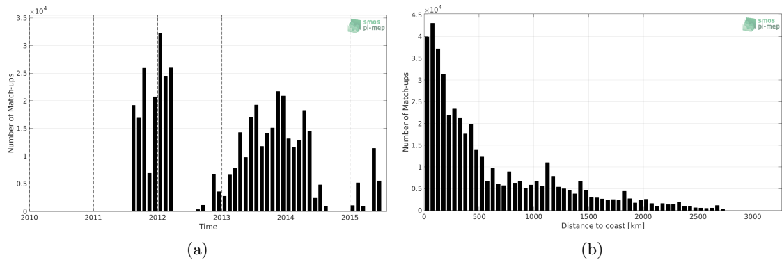
Figure 1: Number of match-ups between TSG-GOSUD-Sailing-ship and Aquarius-L3-OR-V5-MONTHLY-1DEG SSS as a function of time (a) and as function of the distance to coast (b) over the Global Ocean Pi-MEP region and for the full satellite product period.
