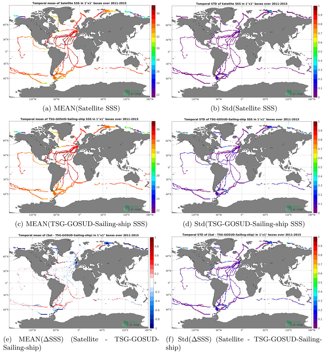
Figure 6: Temporal mean (left) and Std (right) of SSS from Aquarius-L3-OR-V5-MONTHLY-1DEG (top), TSG-GOSUD-Sailing-ship (middle), and of \Delta SSS (Satellite - TSG-GOSUD-Sailing-ship). Only match-up pairs are used to generate these maps.
