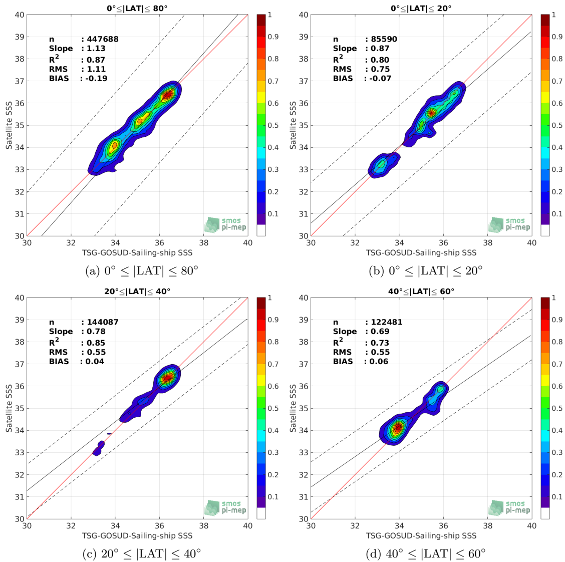
Figure 9: Contour maps of the concentration of Aquarius-L3-OR-V5-MONTHLY-1DEG SSS (y-axis) versus TSG-GOSUD-Sailing-ship SSS (x-axis) at match-up pairs for different latitude bands. For each plot, the red line shows x=y . The black thin and dashed lines indicate a linear fit through the data cloud and the \pm 95\% confidence levels, respectively. The number match-up pairs n , the slope and R^2 coefficient of the linear fit, the root mean square (RMS) and the mean bias between satellite and in situ data are indicated for each latitude band in each plots.
