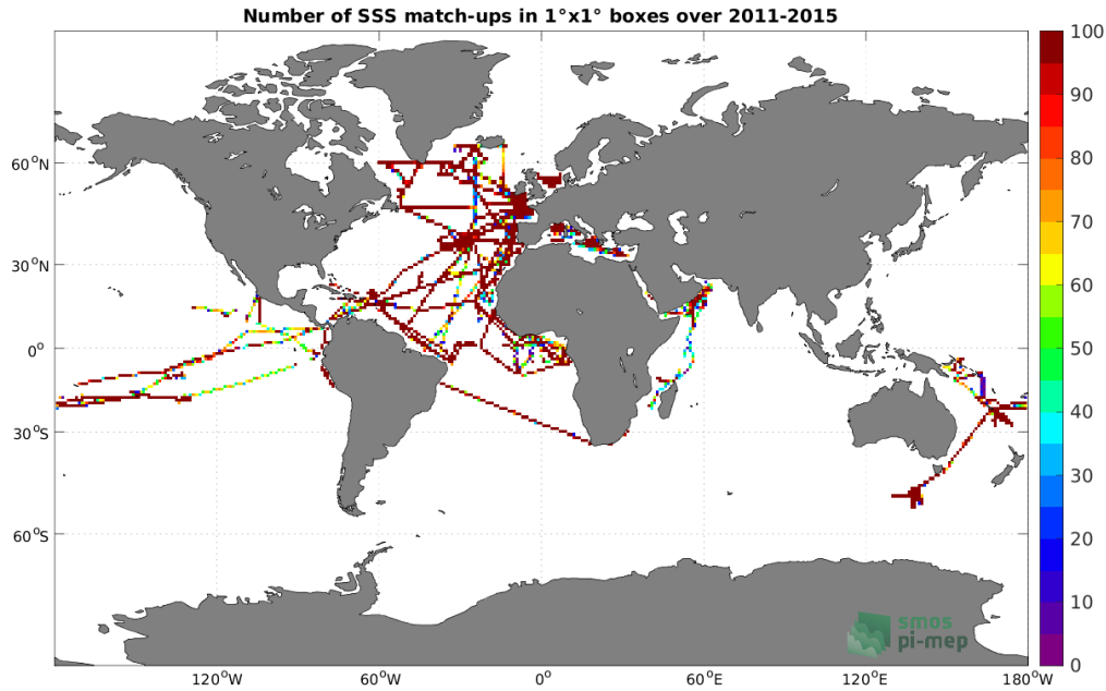
Figure 4: Number of SSS match-ups between TSG (GOSUD-Research-vessel) SSS and the Aquarius SSS L3 OR v5 - Monthly (NASA-GSFC) SSS product for the Global Ocean Pi-MEP region over 1^\circ \times 1^\circ boxes and for the full satellite product period.
