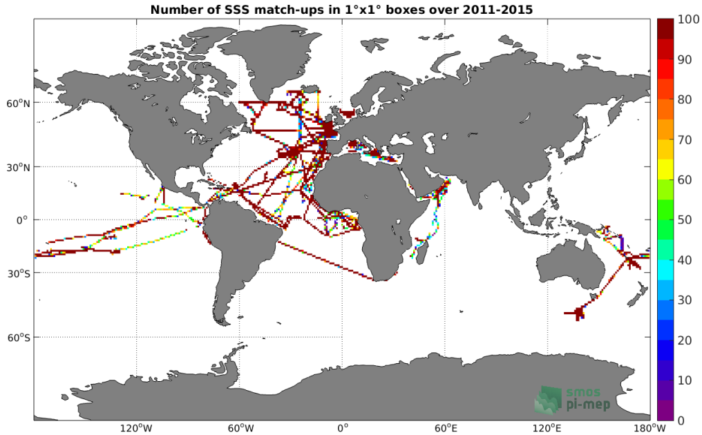
Figure 4: Number of SSS match-ups between TSG (GOSUD-Research-vessel) SSS and the Aquarius SSS L3 OR v5 - Monthly (NASA-GSFC) SSS product for the Global Ocean Pi-MEP region over 1^\circ \times 1^\circ boxes and for the full satellite product period.
