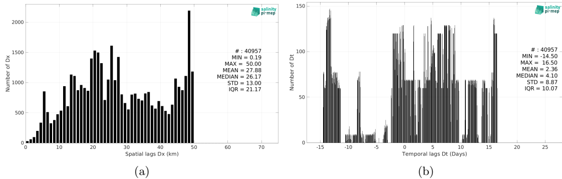
Figure 6: Histograms of the spatial (a) and temporal (b) lags between the location/time of the TSG (Amundsen) measurement and the date of the corresponding Aquarius SSS L3 OR v5 - Monthly (NASA-GSFC) SSS pixel.
