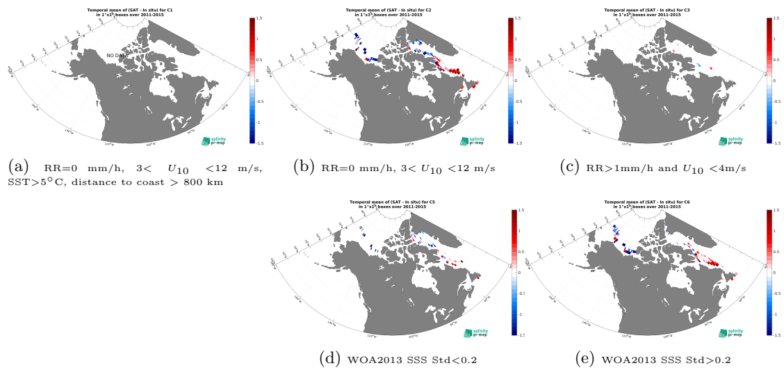
Figure 14: Temporal mean gridded over spatial boxes of size 1^\circ \times 1^\circ of \Delta SSS (Aquarius SSS L3 OR v5 - Monthly (NASA-GSFC) - TSG (Amundsen)) for 5 different subdatasets corresponding to: RR=0 mm/h, 3 < U_{10} < 12 m/s, SST > 5^\circ C , distance to coast > 800 km (a), RR=0 mm/h, 3 < U_{10} < 12 m/s (b), RR > 1 mm/h and U_{10} < 4 m/s (c), WOA2013 SSS Std < 0.2 (d), WOA2013 SSS Std > 0.2 (e).
