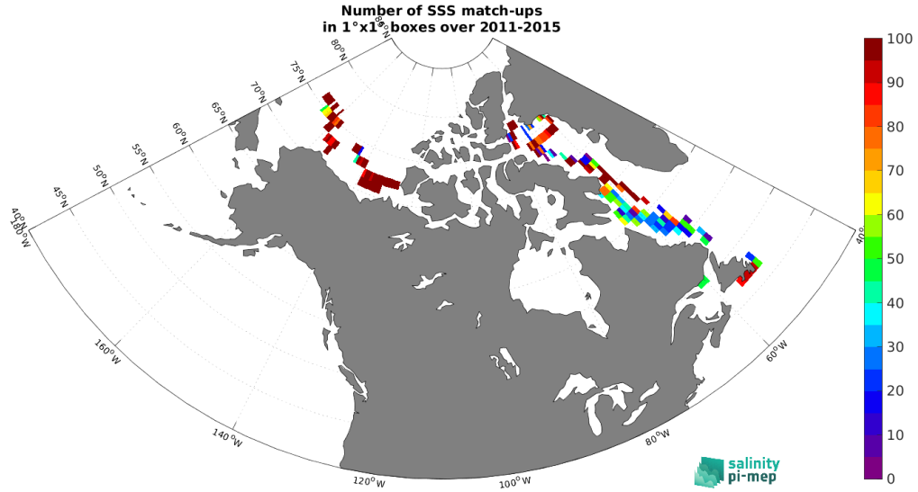
Figure 5: Number of SSS match-ups between TSG (Amundsen) SSS and the Aquarius SSS L3 OR v5 - Monthly (NASA-GSFC) SSS product for the Global Ocean Pi-MEP region over 1^\circ \times 1^\circ boxes and for the full satellite product period.
