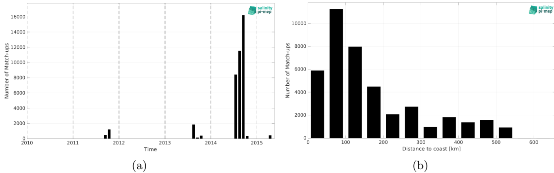
Figure 2: Number of match-ups between TSG (Amundsen) and Aquarius SSS L3 OR v5 - Monthly (NASA-GSFC) SSS as a function of time (a) and as function of the distance to coast (b) over the Global Ocean Pi-MEP region and for the full satellite product period.
