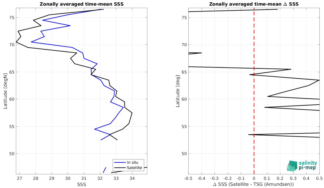
Figure 9: Left panel: Zonal mean SSS from Aquarius SSS L3 OR v5 - Monthly (NASA-GSFC) satellite product (black) and from TSG (Amundsen) (blue). Right panel: Zonal mean of \Delta SSS (Satellite - TSG (Amundsen)) for all the collected Pi-MEP match-up pairs estimated over the full satellite product period.
