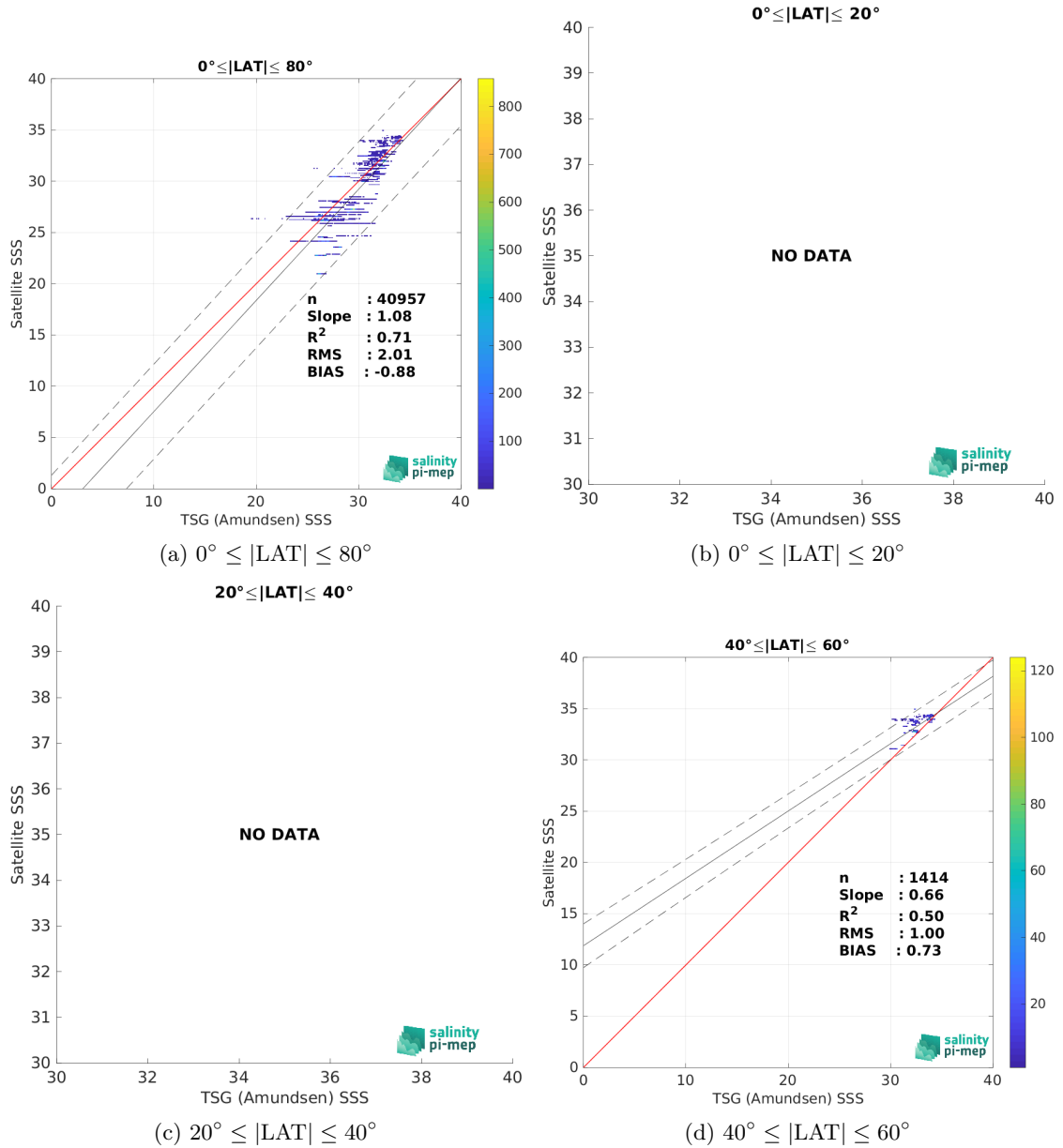
Figure 10: Contour maps of the concentration of Aquarius SSS L3 OR v5 - Monthly (NASA-GSFC) SSS (y-axis) versus TSG (Amundsen) SSS (x-axis) at match-up pairs for different latitude bands. For each plot, the red line shows x=y . The black thin and dashed lines indicate a linear fit through the data cloud and the \pm 95\% confidence levels, respectively. The number match-up pairs n , the slope and R^2 coefficient of the linear fit, the root mean square (RMS) and the mean bias between satellite and in situ data are indicated for each latitude band in each plots.
