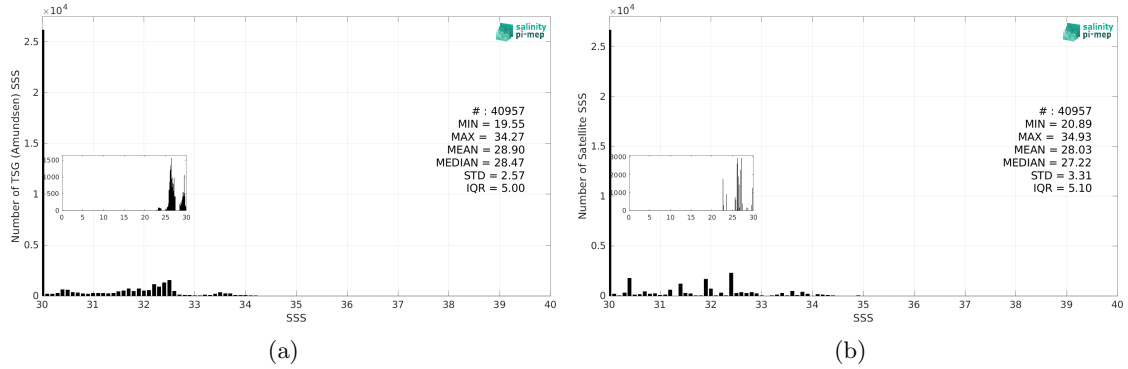
Figure 3: Histograms of SSS from TSG (Amundsen) (a) and Aquarius SSS L3 OR v5 - Monthly (NASA-GSFC) (b) considering all match-up pairs per bins of 0.1 over the Global Ocean Pi-MEP region and for the full satellite product period.
