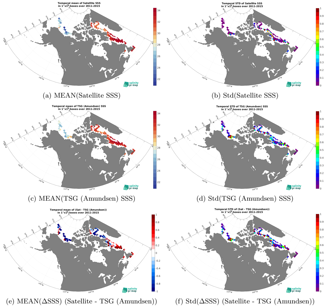
Figure 7: Temporal mean (left) and Std (right) of SSS from Aquarius SSS L3 OR v5 - Monthly (NASA-GSFC) (top), TSG (Amundsen) (middle), and of \Delta SSS (Satellite - TSG (Amundsen)). Only match-up pairs are used to generate these maps.
