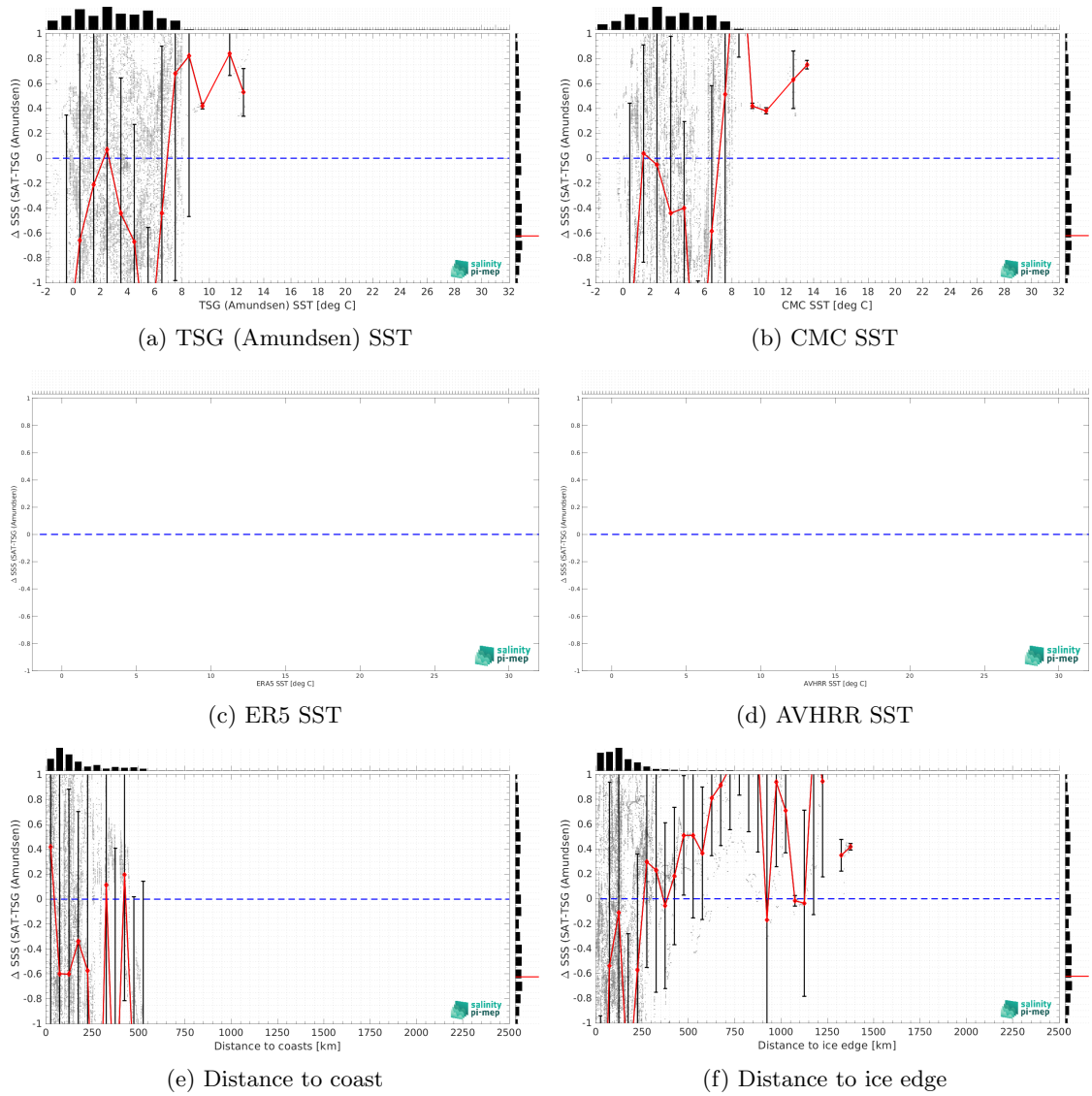
Figure 13: \Delta\text{SSS} (Satellite - TSG (Amundsen)) sorted as function of TSG (Amundsen) SST values (a), CMC SST (b), ERA5 SST (c), AVHRR SST (d), distance to coast (e) and distance to ice edge (f). In all plots the median and Std of \Delta\text{SSS} for each bin is indicated by the red curves and black vertical thick bars ( \pm 1 Std). Links to similar figures sorted as function of Sea ice fraction and in situ measurement depth .
