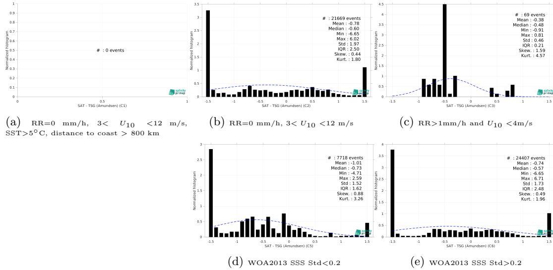
Figure 15: Normalized histogram of \Delta SSS (Aquarius SSS L3 OR v5 - Monthly (NASA-GSFC) - TSG (Amundsen)) for 5 different subdatasets corresponding to: RR=0 mm/h, 3 < U_{10} < 12 m/s, SST>5°C, distance to coast > 800 km (a), RR=0 mm/h, 3 < U_{10} < 12 m/s (b), RR>1mm/h and U_{10} < 4 m/s (c), WOA2013 SSS Std<0.2 (d), WOA2013 SSS Std>0.2 (e).
