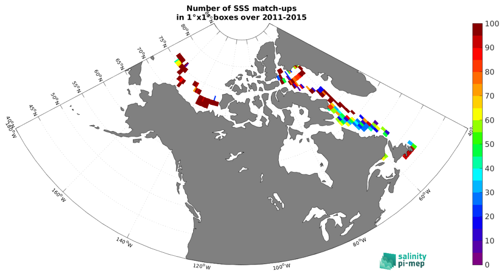
Figure 4: Number of SSS match-ups between TSG (Amundsen) SSS and the Aquarius SSS L3 OR v5 - Monthly (NASA-GSFC) SSS product for the Global Ocean Pi-MEP region over 1°x1° boxes and for the full satellite product period.
