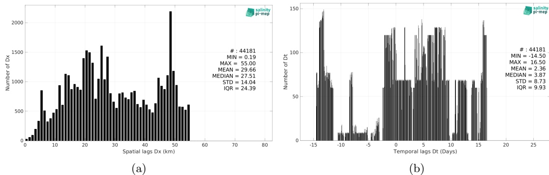
Figure 5: Histograms of the spatial (a) and temporal (b) lags between the location/time of the TSG (Amundsen) measurement and the date of the corresponding Aquarius SSS L3 OR v5 - Monthly (NASA-GSFC) SSS pixel.
