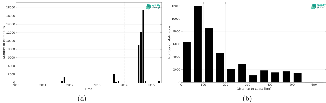
Figure 1: Number of match-ups between TSG (Amundsen) and Aquarius SSS L3 OR v5 - Monthly (NASA-GSFC) SSS as a function of time (a) and as function of the distance to coast (b) over the Global Ocean Pi-MEP region and for the full satellite product period.
