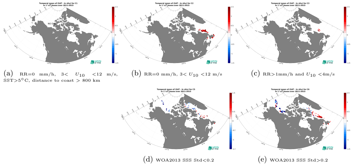
Figure 12: Temporal mean gridded over spatial boxes of size 1^{\circ}\times 1^{\circ} of \Delta\text{SSS} (Aquarius SSS L3 OR v5 - Monthly (NASA-GSFC) - TSG (Amundsen)) for 5 different subdatasets corresponding to:RR=0 mm/h, 3 < U_{10} < 12 m/s, SST >5^{\circ}\text{C} , distance to coast > 800 km (a), RR=0 mm/h, 3 < U_{10} < 12 m/s (b), RR >1 mm/h and U_{10} < 4 m/s (c), WOA2013 SSS Std <0.2 (d), WOA2013 SSS Std >0.2 (e).
