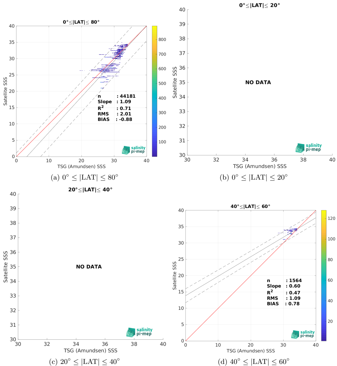
Figure 9: Contour maps of the concentration of Aquarius SSS L3 OR v5 - Monthly (NASA-GSFC) SSS (y-axis) versus TSG (Amundsen) SSS (x-axis) at match-up pairs for different latitude bands. For each plot, the red line shows x=y . The black thin and dashed lines indicate a linear fit through the data cloud and the \pm 95\% confidence levels, respectively. The number match-up pairs n , the slope and R^2 coefficient of the linear fit, the root mean square (RMS) and the mean bias between satellite and in situ data are indicated for each latitude band in each plots.
