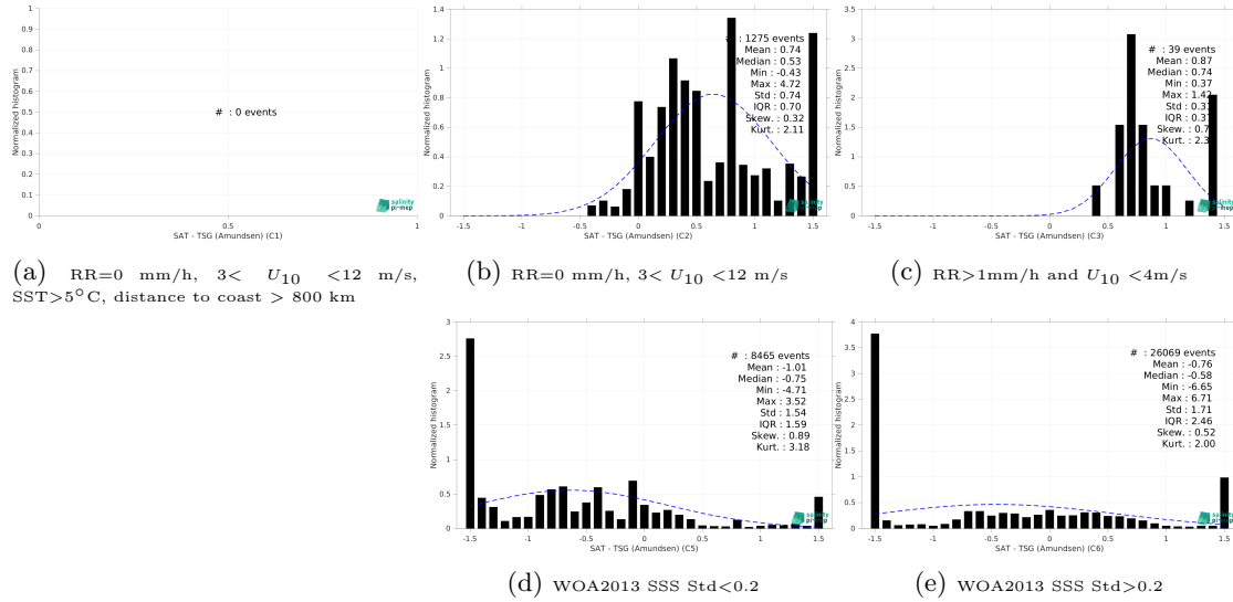
Figure 13: Normalized histogram of \Delta SSS (Aquarius SSS L3 OR v5 - Monthly (NASA-GSFC) - TSG (Amundsen)) for 5 different subdatasets corresponding to: RR=0 mm/h, 3 < U_{10} < 12 m/s, SST > 5°C, distance to coast > 800 km (a), RR=0 mm/h, 3 < U_{10} < 12 m/s (b), RR > 1mm/h and U_{10} < 4 m/s (c), WOA2013 SSS Std < 0.2 (d), WOA2013 SSS Std > 0.2 (e).
