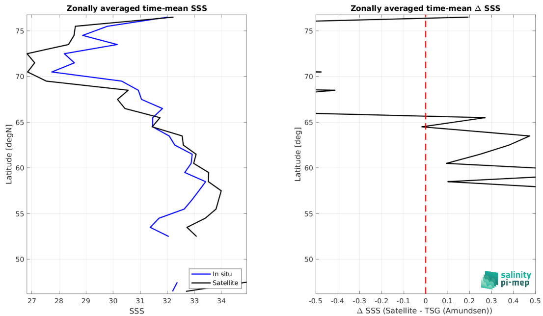
Figure 8: Left panel: Zonal mean SSS from Aquarius SSS L3 OR v5 - Monthly (NASA-GSFC) satellite product (black) and from TSG (Amundsen) (blue). Right panel: Zonal mean of \Delta SSS (Satellite - TSG (Amundsen)) for all the collected Pi-MEP match-up pairs estimated over the full satellite product period.
