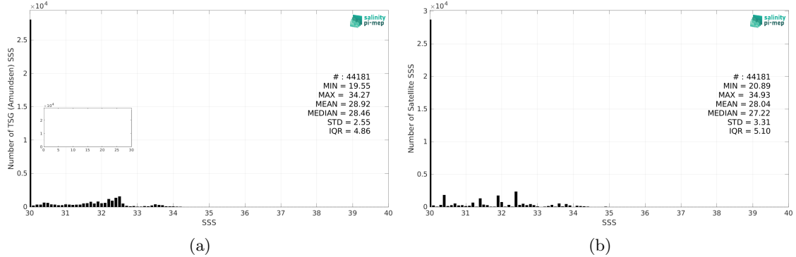
Figure 2: Histograms of SSS from TSG (Amundsen) (a) and Aquarius SSS L3 OR v5 - Monthly (NASA-GSFC) (b) considering all match-up pairs per bins of 0.1 over the Global Ocean Pi-MEP region and for the full satellite product period.
