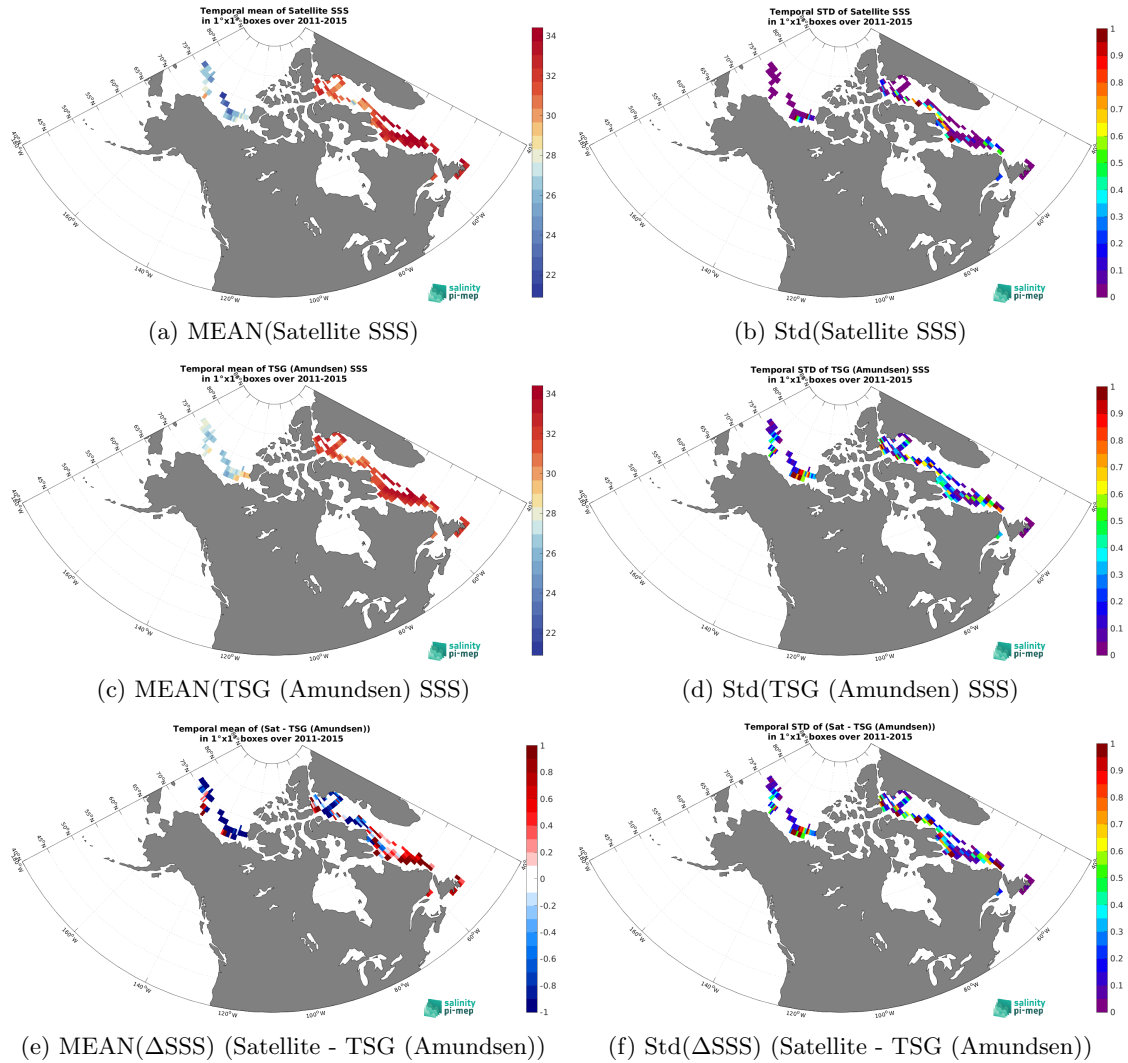
Figure 6: Temporal mean (left) and Std (right) of SSS from Aquarius SSS L3 OR v5 - Monthly (NASA-GSFC) (top), TSG (Amundsen) (middle), and of \Delta SSS (Satellite - TSG (Amundsen)). Only match-up pairs are used to generate these maps.
