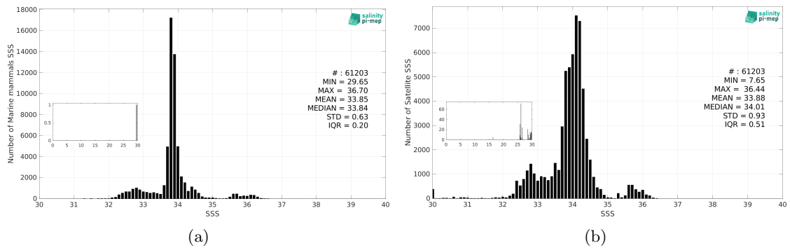
Figure 3: Histograms of SSS from Marine mammals (a) and Aquarius SSS L3 OR v5 - Monthly (NASA-GSFC) (b) considering all match-up pairs per bins of 0.1 over the Global Ocean Pi-MEP region and for the full satellite product period.
