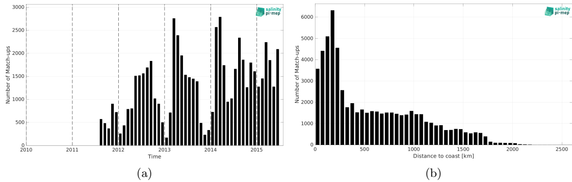
Figure 2: Number of match-ups between Marine mammals and Aquarius SSS L3 OR v5 - Monthly (NASA-GSFC) SSS as a function of time (a) and as function of the distance to coast (b) over the Global Ocean Pi-MEP region and for the full satellite product period.
