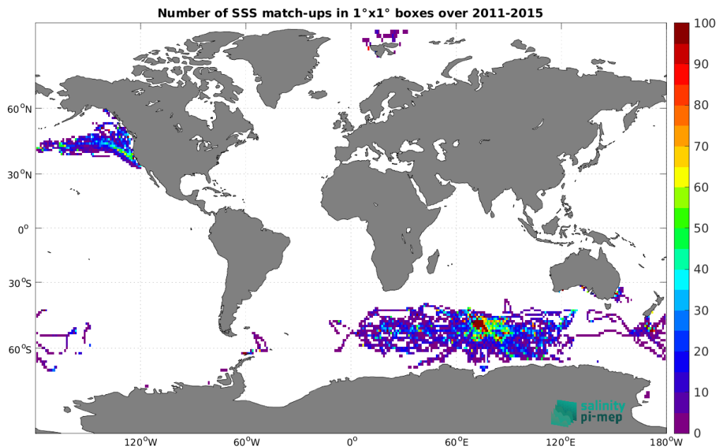
Figure 5: Number of SSS match-ups between Marine mammals SSS and the Aquarius SSS L3 OR v5 - Monthly (NASA-GSFC) SSS product for the Global Ocean Pi-MEP region over 1^\circ \times 1^\circ boxes and for the full satellite product period.
