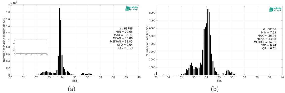
Figure 2: Histograms of SSS from Marine mammals (a) and Aquarius SSS L3 OR v5 - Monthly (NASA-GSFC) (b) considering all match-up pairs per bins of 0.1 over the Global Ocean Pi-MEP region and for the full satellite product period.
