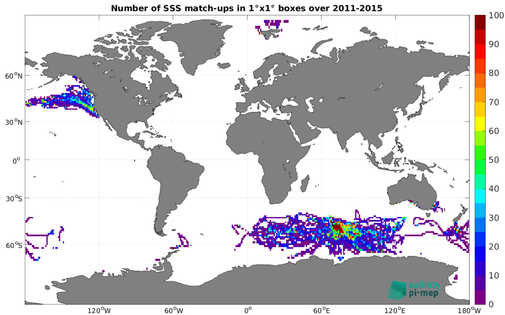
Figure 4: Number of SSS match-ups between Marine mammals SSS and the Aquarius SSS L3 OR v5 - Monthly (NASA-GSFC) SSS product for the Global Ocean Pi-MEP region over 1^\circ \times 1^\circ boxes and for the full satellite product period.
