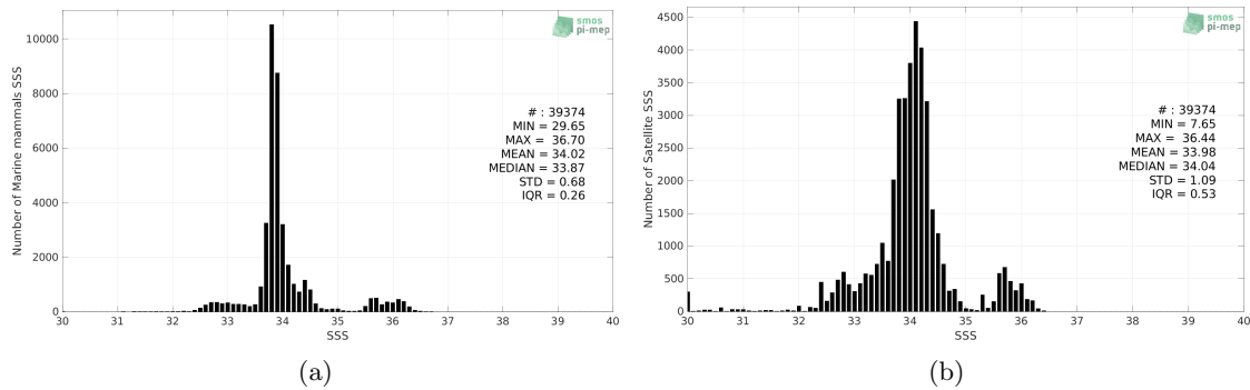
Figure 2: Histograms of SSS from Marine mammals (a) and Aquarius SSS L3 OR v5 - Monthly (NASA-GSFC) (b) considering all match-up pairs per bins of 0.1 over the Global Ocean Pi-MEP region and for the full satellite product period.
