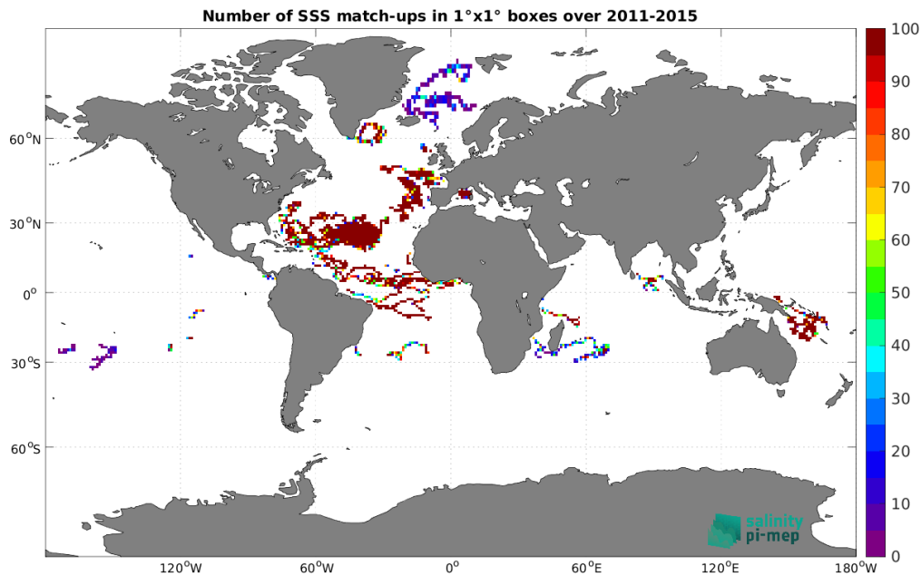
Figure 3: Number of SSS match-ups between Surface drifters SSS and the Aquarius SSS L3 OR v5 - Monthly (NASA-GSFC) SSS product for the Global Ocean Pi-MEP region over 1°×1° boxes and for the full satellite product period.
