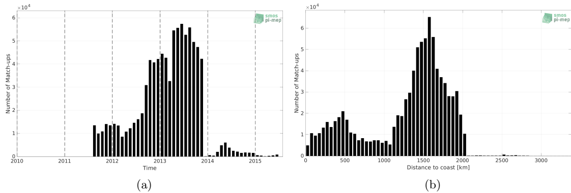
Figure 1: Number of match-ups between Surface drifters and Aquarius SSS L3 OR v5 - Monthly (NASA-GSFC) SSS as a function of time (a) and as function of the distance to coast (b) over the Global Ocean Pi-MEP region and for the full satellite product period.
