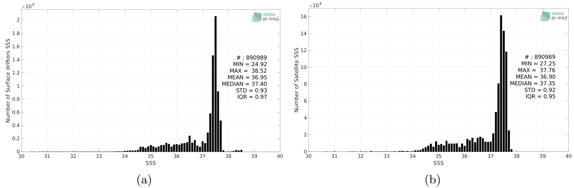
Figure 2: Histograms of SSS from Surface drifters (a) and Aquarius SSS L3 OR v5 - Monthly (NASA-GSFC) (b) considering all match-up pairs per bins of 0.1 over the Global Ocean Pi-MEP region and for the full satellite product period.
