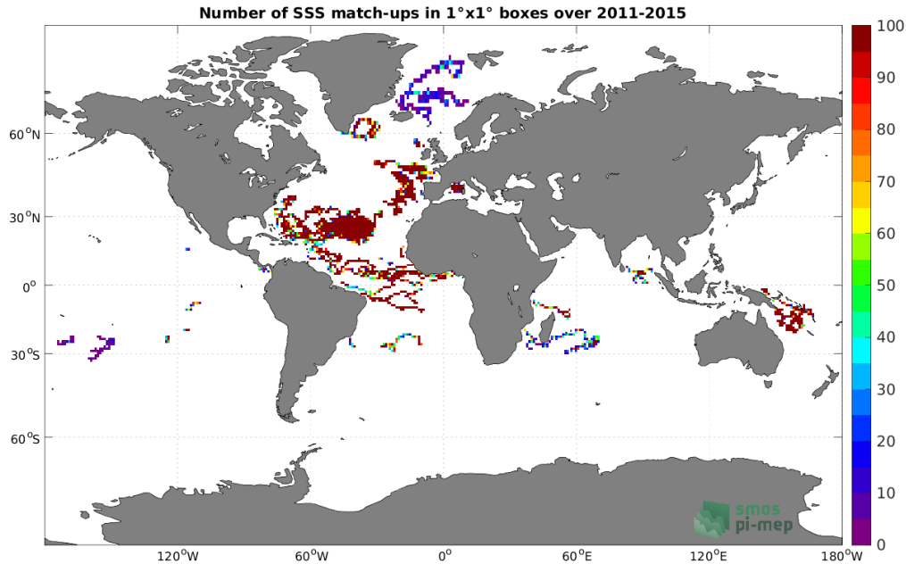
Figure 3: Number of SSS match-ups between Surface drifters SSS and the Aquarius SSS L3 OR v5 - Monthly (NASA-GSFC) SSS product for the Global Ocean Pi-MEP region over 1^\circ \times 1^\circ boxes and for the full satellite product period.
