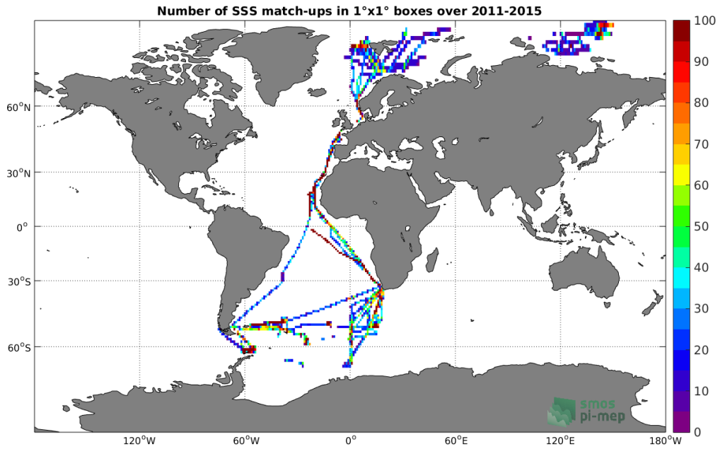
Figure 4: Number of SSS match-ups between TSG-POLARSTERN SSS and the Aquarius-L3-OR-V5-MONTHLY-RAIN-MASK-1DEG SSS product for the Global Ocean Pi-MEP region over 1°x1° boxes and for the full satellite product period.
