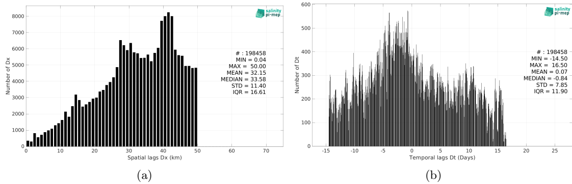
Figure 6: Histograms of the spatial (a) and temporal (b) lags between the location/time of the TSG (NCEI-0170743) measurement and the date of the corresponding Aquarius SSS L3 OR v5 - Monthly - Rain mask (NASA-GSFC) SSS pixel.
