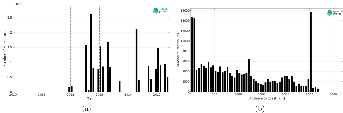
Figure 2: Number of match-ups between TSG (NCEI-0170743) and Aquarius SSS L3 OR v5 - Monthly - Rain mask (NASA-GSFC) SSS as a function of time (a) and as function of the distance to coast (b) over the Global Ocean Pi-MEP region and for the full satellite product period.
