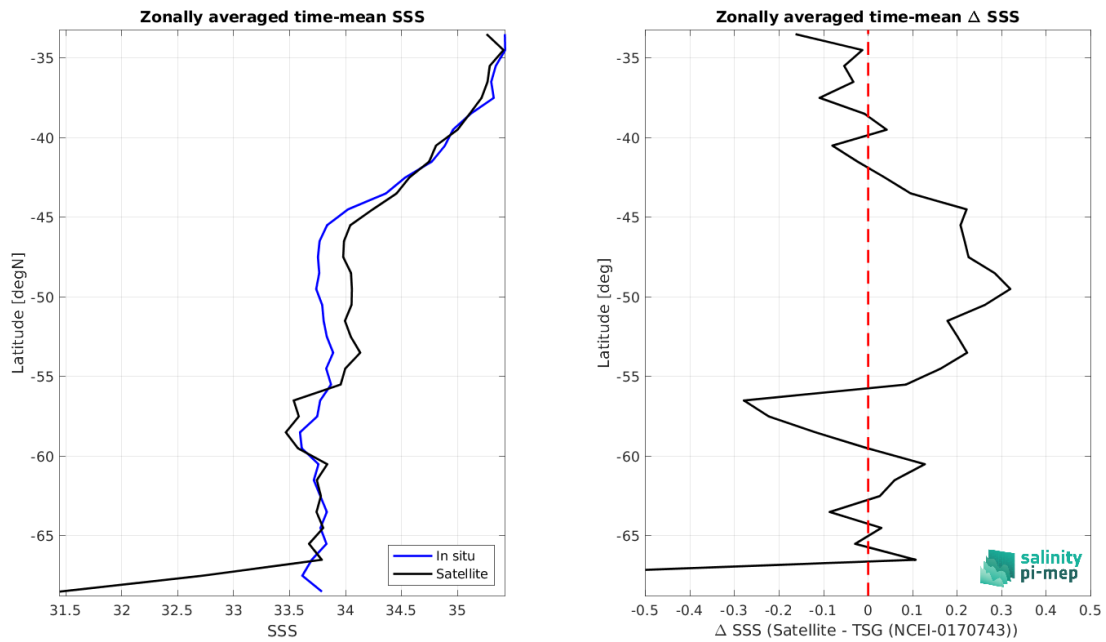
Figure 9: Left panel: Zonal mean SSS from Aquarius SSS L3 OR v5 - Monthly - Rain mask (NASA-GSFC) satellite product (black) and from TSG (NCEI-0170743) (blue). Right panel: Zonal mean of \Delta SSS (Satellite - TSG (NCEI-0170743)) for all the collected Pi-MEP match-up pairs estimated over the full satellite product period.
