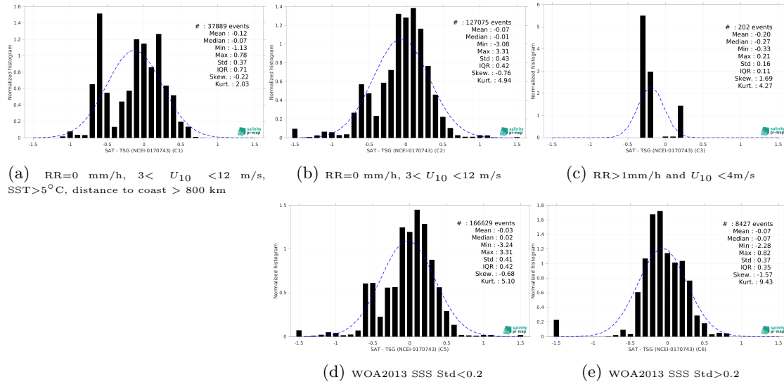
Figure 15: Normalized histogram of \Delta\text{SSS} (Aquarius SSS L3 OR v5 - Monthly - Rain mask (NASA-GSFC) - TSG (NCEI-0170743)) for 5 different subdatasets corresponding to: RR=0 mm/h, 3 < U_{10} < 12 m/s, SST > 5^{\circ}\text{C} , distance to coast > 800 km (a), RR=0 mm/h, 3 < U_{10} < 12 m/s (b), RR > 1\text{mm/h} and U_{10} < 4\text{m/s} (c), WOA2013 SSS Std < 0.2 (d), WOA2013 SSS Std > 0.2 (e).
