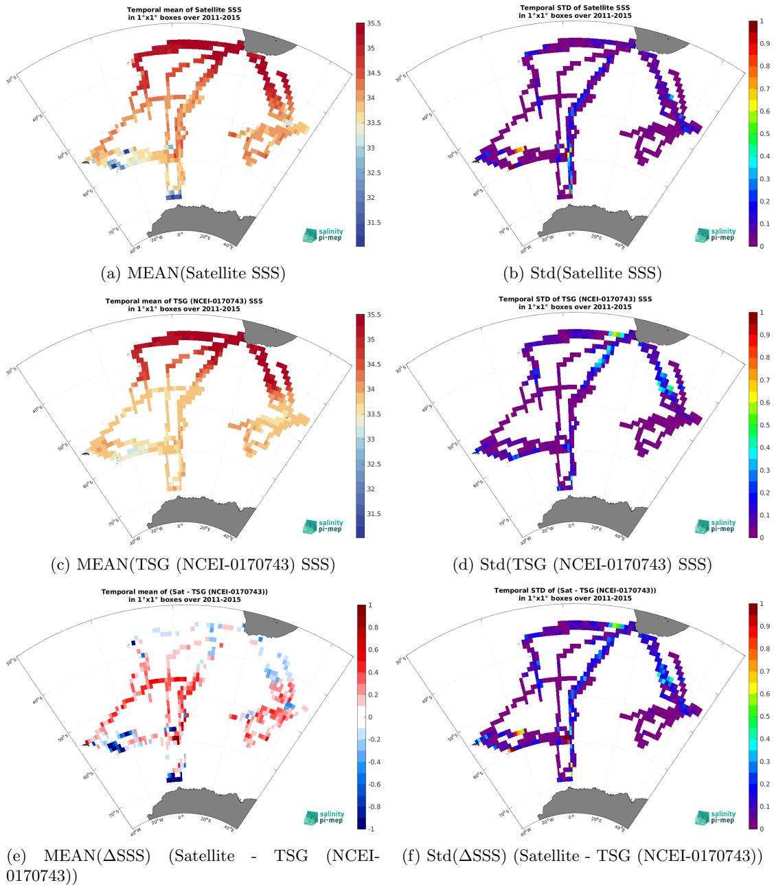
Figure 7: Temporal mean (left) and Std (right) of SSS from Aquarius SSS L3 OR v5 - Monthly - Rain mask (NASA-GSFC) (top), TSG (NCEI-0170743) (middle), and of \Delta SSS (Satellite - TSG (NCEI-0170743)). Only match-up pairs are used to generate these maps.
