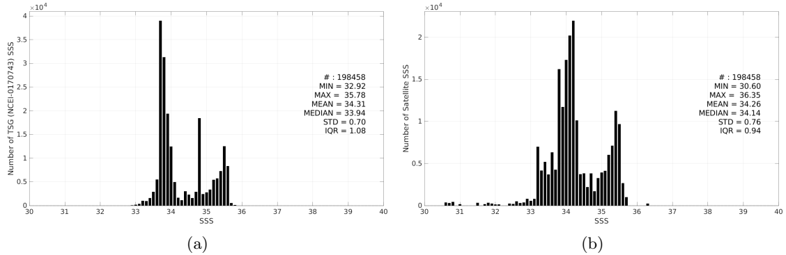
Figure 3: Histograms of SSS from TSG (NCEI-0170743) (a) and Aquarius SSS L3 OR v5 - Monthly - Rain mask (NASA-GSFC) (b) considering all match-up pairs per bins of 0.1 over the Global Ocean Pi-MEP region and for the full satellite product period.
