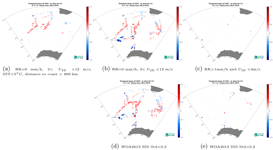
Figure 14: Temporal mean gridded over spatial boxes of size 1^\circ \times 1^\circ of \Delta SSS (Aquarius SSS L3 OR v5 - Monthly - Rain mask (NASA-GSFC) - TSG (NCEI-0170743)) for 5 different subdatasets corresponding to:RR=0 mm/h, 3 < U_{10} < 12 m/s, SST >5^\circ\text{C} , distance to coast > 800 km (a), RR=0 mm/h, 3 < U_{10} < 12 m/s (b), RR >1 mm/h and U_{10} < 4 m/s (c), WOA2013 SSS Std <0.2 (d), WOA2013 SSS Std >0.2 (e).
