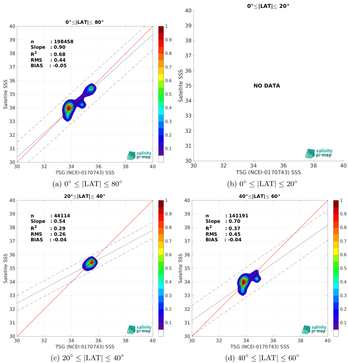
Figure 10: Contour maps of the concentration of Aquarius SSS L3 OR v5 - Monthly - Rain mask (NASA-GSFC) SSS (y-axis) versus TSG (NCEI-0170743) SSS (x-axis) at match-up pairs for different latitude bands. For each plot, the red line shows x=y . The black thin and dashed lines indicate a linear fit through the data cloud and the \pm 95\% confidence levels, respectively. The number match-up pairs n , the slope and R^2 coefficient of the linear fit, the root mean square (RMS) and the mean bias between satellite and in situ data are indicated for each latitude band in each plots.
