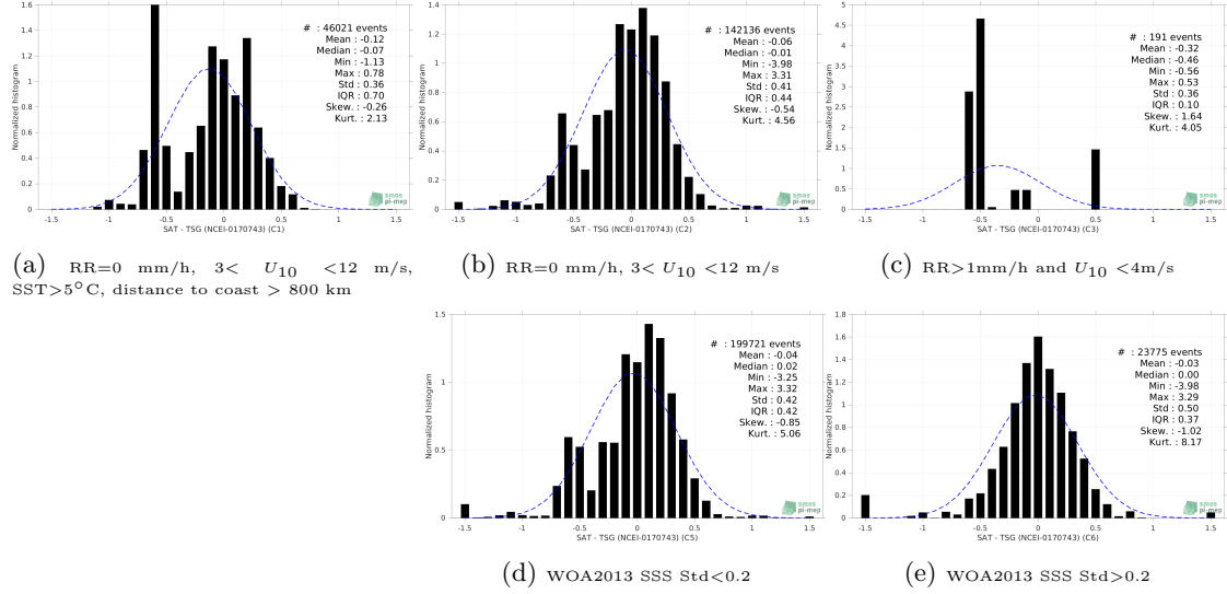
Figure 13: Normalized histogram of \Delta\text{SSS} (Aquarius SSS L3 OR v5 - Monthly - Rain mask (NASA-GSFC) - TSG (NCEI-0170743)) for 5 different subdatasets corresponding to: RR=0 mm/h, 3 < U_{10} < 12 m/s, SST>5°C, distance to coast > 800 km (a), RR=0 mm/h, 3 < U_{10} < 12 m/s (b), RR>1mm/h and U_{10} < 4 m/s (c), WOA2013 SSS Std<0.2 (d), WOA2013 SSS Std>0.2 (e).
