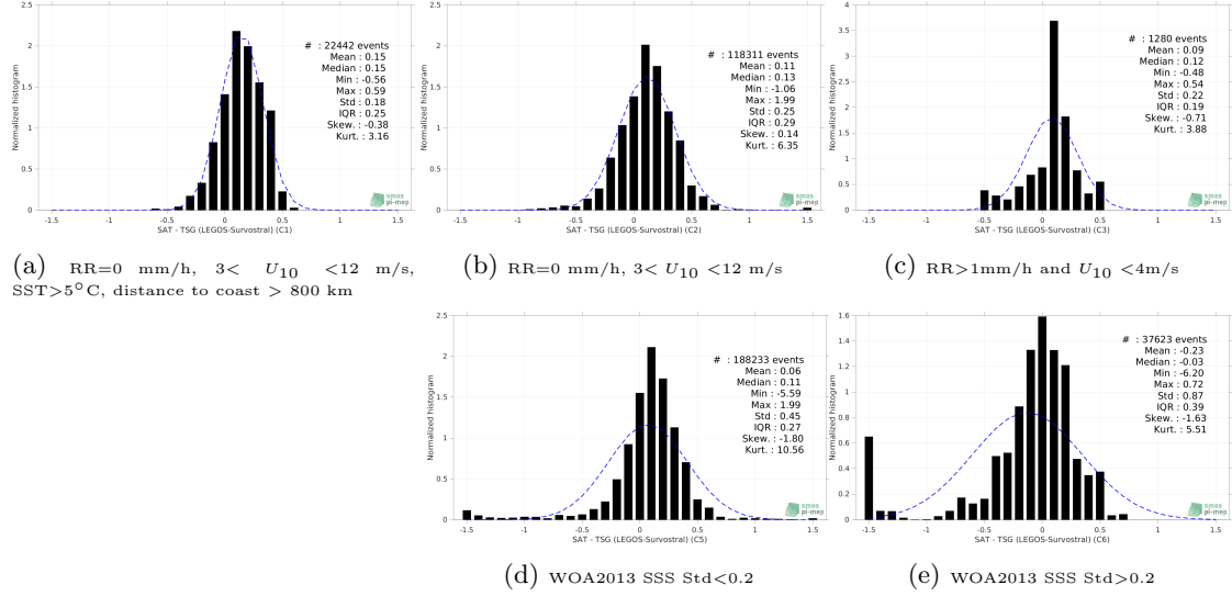
Figure 13: Normalized histogram of \Delta SSS (Aquarius SSS L3 OR v5 - Monthly - Rain mask (NASA-GSFC) - TSG (LEGOS-Survostral)) for 5 different subdatasets corresponding to: RR=0 mm/h, 3 < U_{10} < 12 m/s, SST > 5°C, distance to coast > 800 km (a), RR=0 mm/h, 3 < U_{10} < 12 m/s (b), RR > 1mm/h and U_{10} < 4 m/s (c), WOA2013 SSS Std < 0.2 (d), WOA2013 SSS Std > 0.2 (e).
