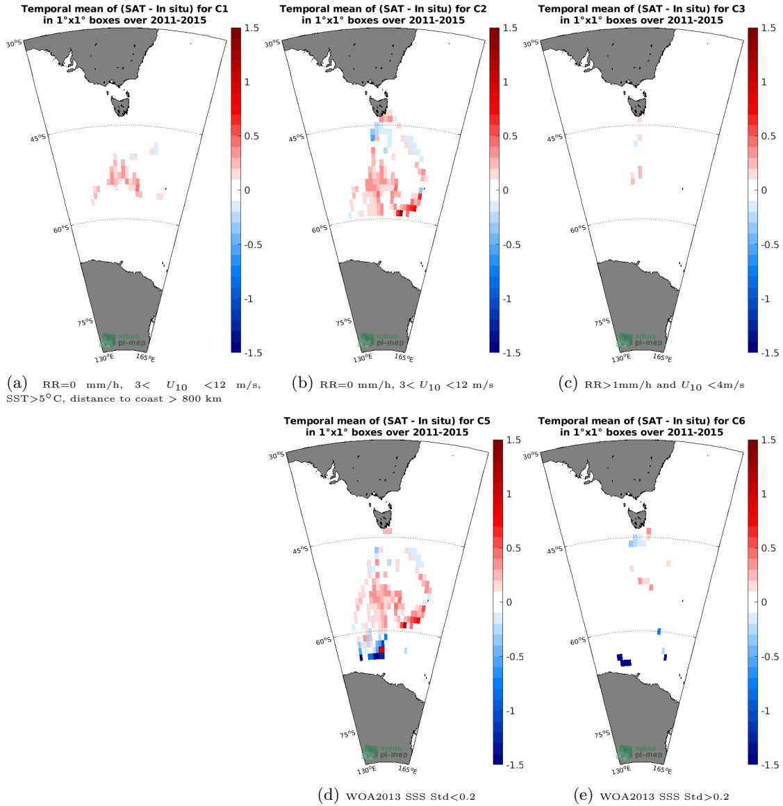
Figure 12: Temporal mean gridded over spatial boxes of size 1°x1° of \Delta SSS (Aquarius SSS L3 OR v5 - Monthly - Rain mask (NASA-GSFC) - TSG (LEGOS-Survostral)) for 5 different subdatasets corresponding to:RR=0 mm/h, 3 < U_{10} < 12 m/s, SST>5°C, distance to coast > 800 km (a), RR=0 mm/h, 3 < U_{10} < 12 m/s (b), RR>1mm/h and U_{10} < 4 m/s (c), WOA2013 SSS Std<0.2 (d), WOA2013 SSS Std>0.2 (e).
