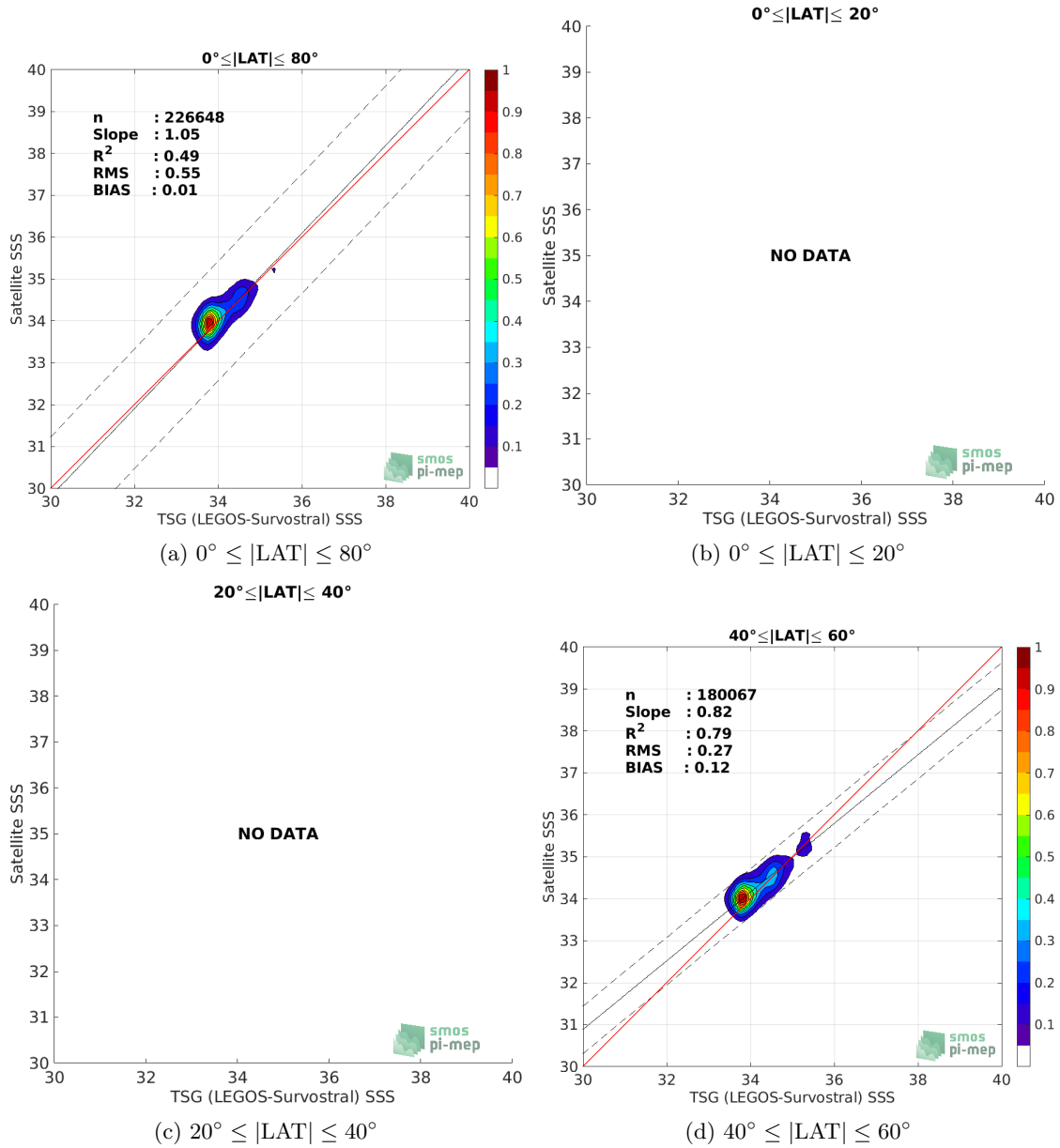
Figure 9: Contour maps of the concentration of Aquarius SSS L3 OR v5 - Monthly - Rain mask (NASA-GSFC) SSS ( y -axis) versus TSG (LEGOS-Survostral) SSS ( x -axis) at match-up pairs for different latitude bands. For each plot, the red line shows x=y . The black thin and dashed lines indicate a linear fit through the data cloud and the \pm 95\% confidence levels, respectively. The number match-up pairs n , the slope and R^2 coefficient of the linear fit, the root mean square (RMS) and the mean bias between satellite and in situ data are indicated for each latitude band in each plots.
