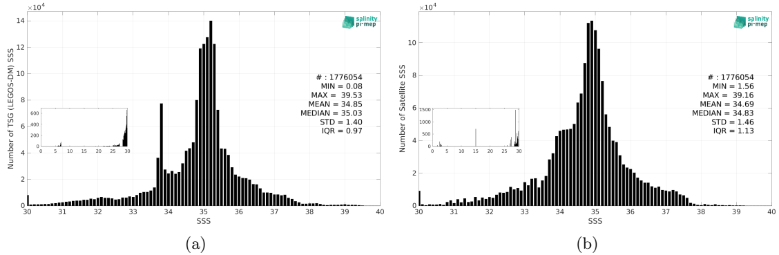
Figure 3: Histograms of SSS from TSG (LEGOS-DM) (a) and Aquarius SSS L3 OR v5 - Monthly - Rain mask (NASA-GSFC) (b) considering all match-up pairs per bins of 0.1 over the Global Ocean Pi-MEP region and for the full satellite product period.
