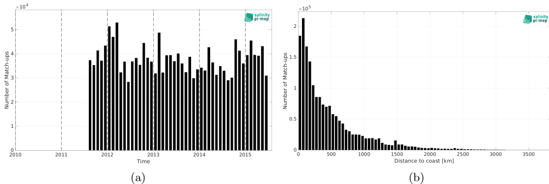
Figure 2: Number of match-ups between TSG (LEGOS-DM) and Aquarius SSS L3 OR v5 - Monthly - Rain mask (NASA-GSFC) SSS as a function of time (a) and as function of the distance to coast (b) over the Global Ocean Pi-MEP region and for the full satellite product period.
