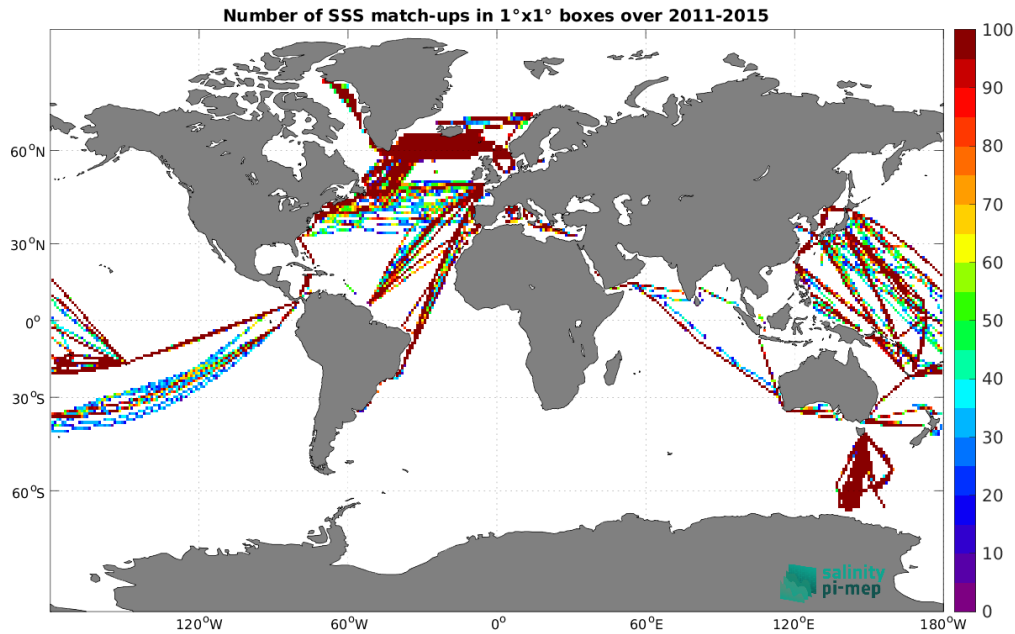
Figure 5: Number of SSS match-ups between TSG (LEGOS-DM) SSS and the Aquarius SSS L3 OR v5 - Monthly - Rain mask (NASA-GSFC) SSS product for the Global Ocean Pi-MEP region over 1^\circ \times 1^\circ boxes and for the full satellite product period.
