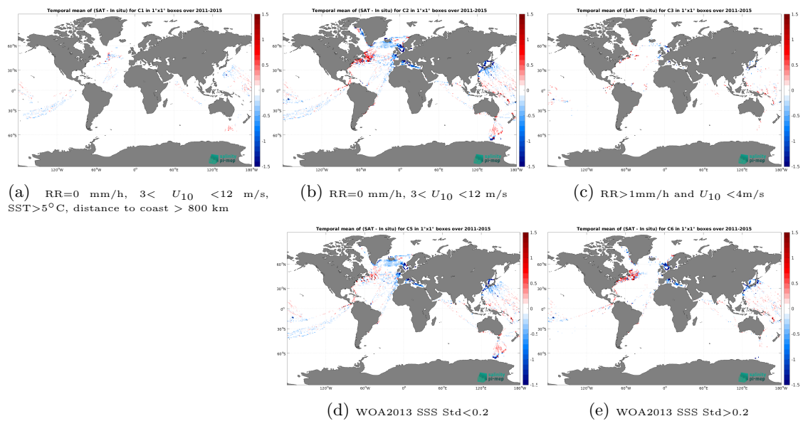
Figure 14: Temporal mean gridded over spatial boxes of size 1^\circ \times 1^\circ of \Delta\text{SSS} (Aquarius SSS L3 OR v5 - Monthly - Rain mask (NASA-GSFC) - TSG (LEGOS-DM)) for 5 different subdatasets corresponding to: RR=0 mm/h, 3 < U_{10} < 12 m/s, SST > 5^\circ\text{C} , distance to coast > 800 km (a), RR=0 mm/h, 3 < U_{10} < 12 m/s (b), RR > 1 mm/h and U_{10} < 4 m/s (c), WOA2013 SSS Std < 0.2 (d), WOA2013 SSS Std > 0.2 (e).
