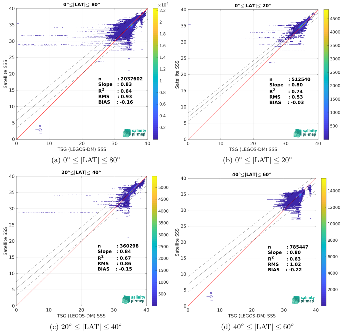
Figure 9: Contour maps of the concentration of Aquarius SSS L3 OR v5 - Monthly - Rain mask (NASA-GSFC) SSS (y-axis) versus TSG (LEGOS-DM) SSS (x-axis) at match-up pairs for different latitude bands. For each plot, the red line shows x=y . The black thin and dashed lines indicate a linear fit through the data cloud and the \pm 95\% confidence levels, respectively. The number match-up pairs n , the slope and R^2 coefficient of the linear fit, the root mean square (RMS) and the mean bias between satellite and in situ data are indicated for each latitude band in each plots.
