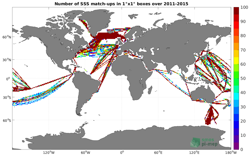
Figure 4: Number of SSS match-ups between TSG (LEGOS-DM) SSS and the Aquarius SSS L3 OR v5 - Monthly - Rain mask (NASA-GSFC) SSS product for the Global Ocean Pi-MEP region over 1^\circ \times 1^\circ boxes and for the full satellite product period.
