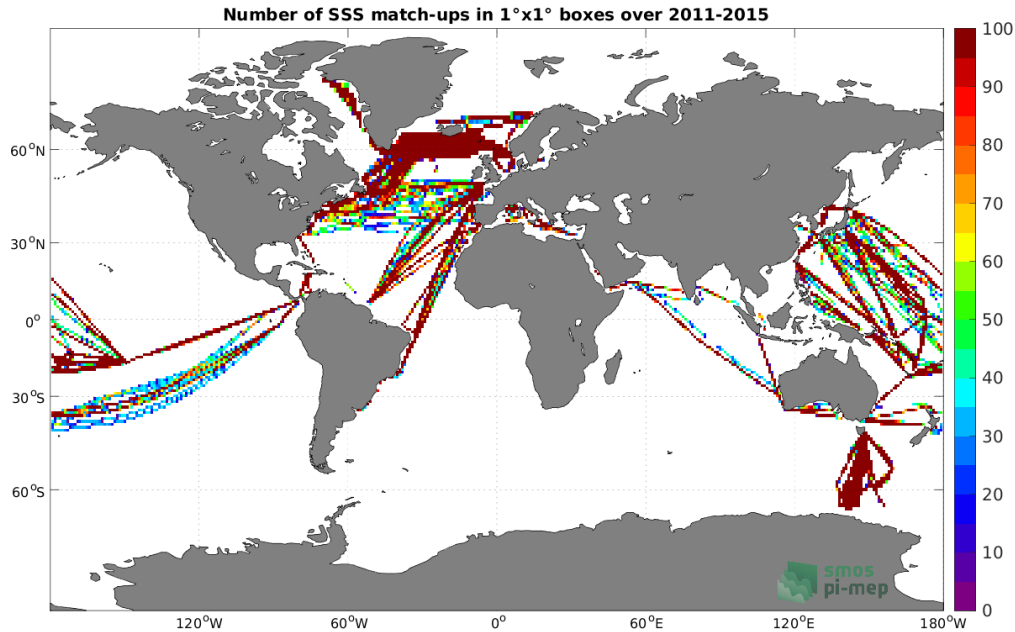
Figure 4: Number of SSS match-ups between TSG (LEGOS-DM) SSS and the Aquarius SSS L3 OR v5 - Monthly - Rain mask (NASA-GSFC) SSS product for the Global Ocean Pi-MEP region over 1°×1° boxes and for the full satellite product period.
