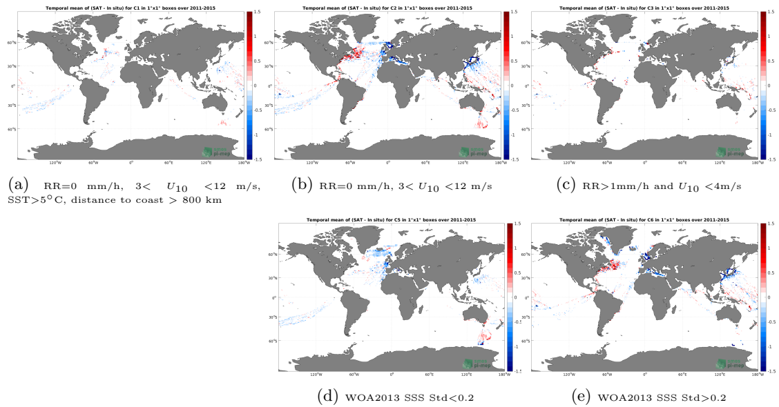
Figure 12: Temporal mean gridded over spatial boxes of size 1^\circ \times 1^\circ of \Delta SSS (Aquarius SSS L3 OR v5 - Monthly - Rain mask (NASA-GSFC) - TSG (LEGOS-DM)) for 5 different subdatasets corresponding to:RR=0 mm/h, 3 < U_{10} < 12 m/s, SST >5^\circ C, distance to coast > 800 km (a), RR=0 mm/h, 3 < U_{10} < 12 m/s (b), RR >1 mm/h and U_{10} < 4 m/s (c), WOA2013 SSS Std <0.2 (d), WOA2013 SSS Std >0.2 (e).
