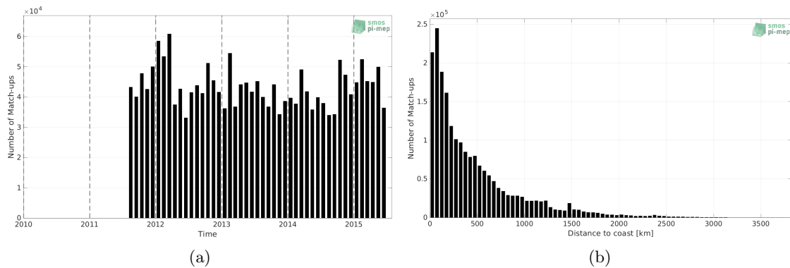
Figure 1: Number of match-ups between TSG (LEGOS-DM) and Aquarius SSS L3 OR v5 - Monthly - Rain mask (NASA-GSFC) SSS as a function of time (a) and as function of the distance to coast (b) over the Global Ocean Pi-MEP region and for the full satellite product period.
