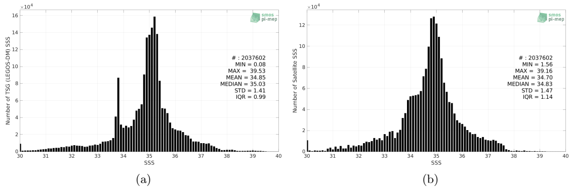
Figure 2: Histograms of SSS from TSG (LEGOS-DM) (a) and Aquarius SSS L3 OR v5 - Monthly - Rain mask (NASA-GSFC) (b) considering all match-up pairs per bins of 0.1 over the Global Ocean Pi-MEP region and for the full satellite product period.
