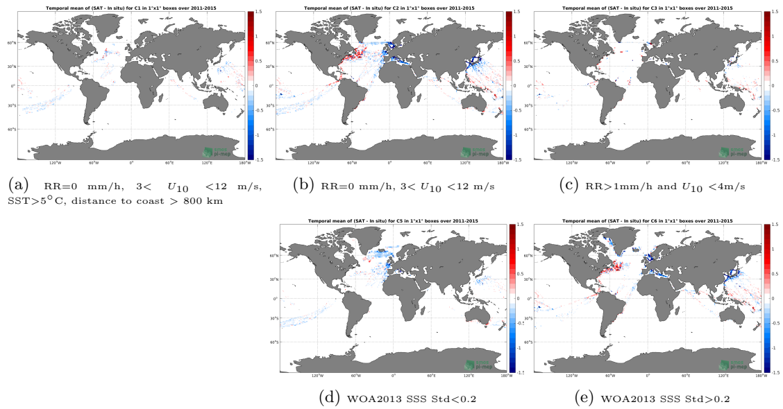
Figure 12: Temporal mean gridded over spatial boxes of size 1^\circ \times 1^\circ of \Delta SSS (Aquarius-L3-OR-V5-MONTHLY-RAIN-MASK-1DEG - TSG-LEGOS-DM) for 5 different subdatasets corresponding to: RR=0 mm/h, 3 < U_{10} < 12 m/s, SST > 5^\circ C, distance to coast > 800 km (a), RR=0 mm/h, 3 < U_{10} < 12 m/s (b), RR > 1 mm/h and U_{10} < 4 m/s (c), WOA2013 SSS Std < 0.2 (d), WOA2013 SSS Std > 0.2 (e).
