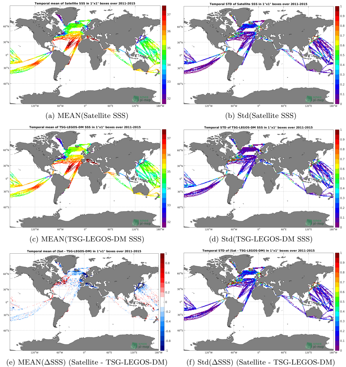
Figure 6: Temporal mean (left) and Std (right) of SSS from Aquarius-L3-OR-V5-MONTHLY-RAIN-MASK-1DEG (top), TSG-LEGOS-DM (middle), and of \Delta SSS (Satellite - TSG-LEGOS-DM). Only match-up pairs are used to generate these maps.
