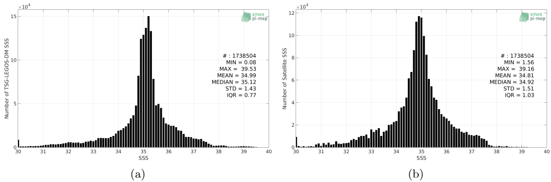
Figure 2: Histograms of SSS from TSG-LEGOS-DM (a) and Aquarius-L3-OR-V5-MONTHLY-RAIN-MASK-1DEG (b) considering all match-up pairs per bins of 0.1 over the Global Ocean Pi-MEP region and for the full satellite product period.
