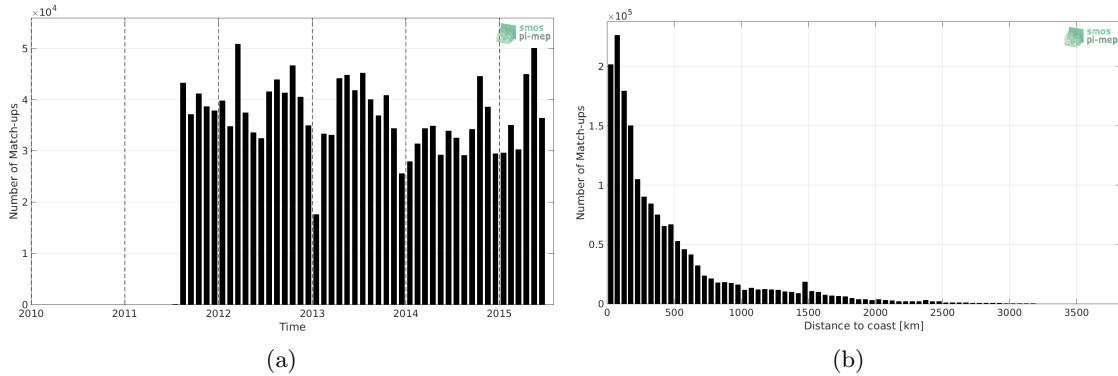
Figure 1: Number of match-ups between TSG-LEGOS-DM and Aquarius-L3-OR-V5-MONTHLY-RAIN-MASK-1DEG SSS as a function of time (a) and as function of the distance to coast (b) over the Global Ocean Pi-MEP region and for the full satellite product period.
