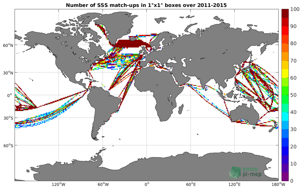
Figure 4: Number of SSS match-ups between TSG-LEGOS-DM SSS and the Aquarius-L3-OR-V5-MONTHLY-RAIN-MASK-1DEG SSS product for the Global Ocean Pi-MEP region over 1^\circ \times 1^\circ boxes and for the full satellite product period.
