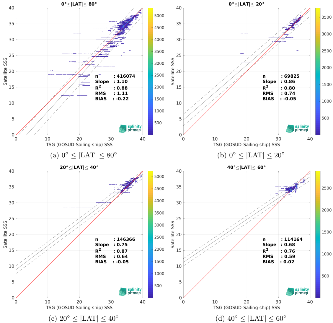
Figure 10: Contour maps of the concentration of Aquarius SSS L3 OR v5 - Monthly - Rain mask (NASA-GSFC) SSS (y-axis) versus TSG (GOSUD-Sailing-ship) SSS (x-axis) at match-up pairs for different latitude bands. For each plot, the red line shows x=y . The black thin and dashed lines indicate a linear fit through the data cloud and the \pm 95\% confidence levels, respectively. The number match-up pairs n , the slope and R^2 coefficient of the linear fit, the root mean square (RMS) and the mean bias between satellite and in situ data are indicated for each latitude band in each plots.
