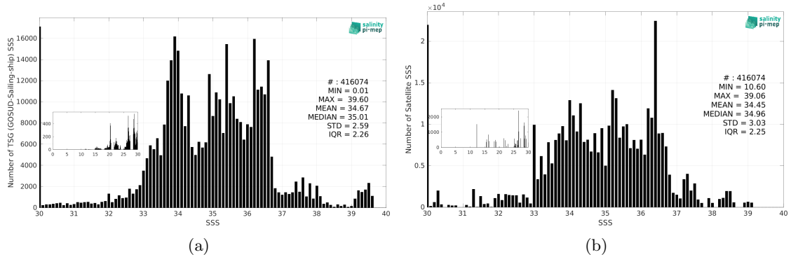
Figure 3: Histograms of SSS from TSG (GOSUD-Sailing-ship) (a) and Aquarius SSS L3 OR v5 - Monthly - Rain mask (NASA-GSFC) (b) considering all match-up pairs per bins of 0.1 over the Global Ocean Pi-MEP region and for the full satellite product period.
