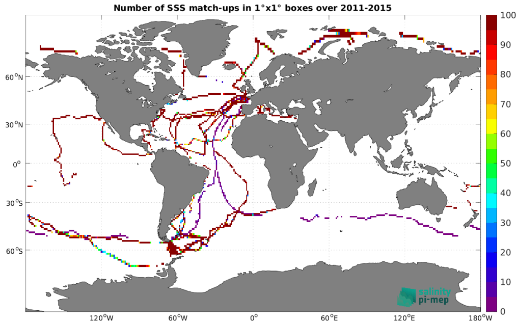
Figure 4: Number of SSS match-ups between TSG (GOSUD-Sailing-ship) SSS and the Aquarius SSS L3 OR v5 - Monthly - Rain mask (NASA-GSFC) SSS product for the Global Ocean Pi-MEP region over 1^\circ \times 1^\circ boxes and for the full satellite product period.
