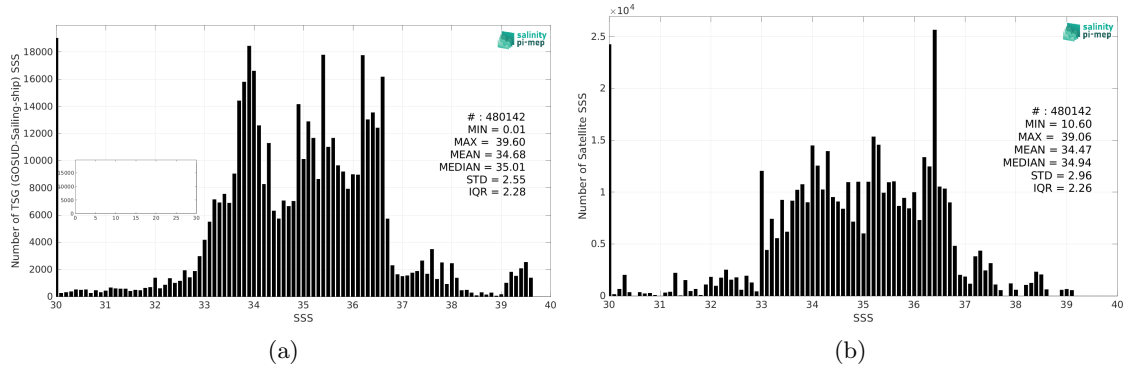
Figure 2: Histograms of SSS from TSG (GOSUD-Sailing-ship) (a) and Aquarius SSS L3 OR v5 - Monthly - Rain mask (NASA-GSFC) (b) considering all match-up pairs per bins of 0.1 over the Global Ocean Pi-MEP region and for the full satellite product period.
