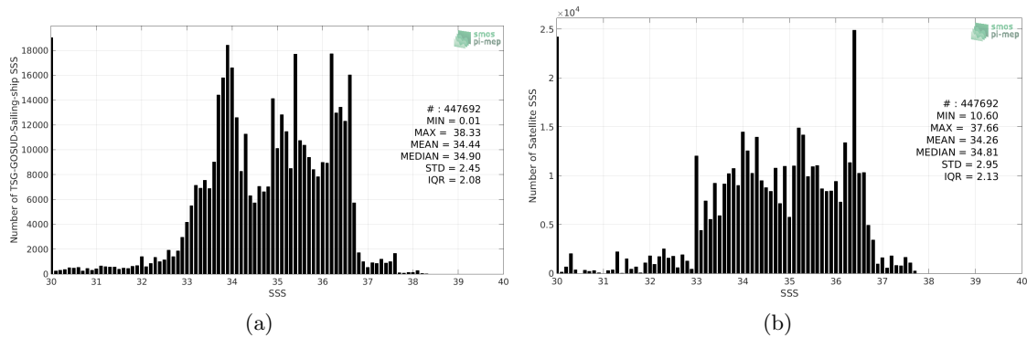
Figure 2: Histograms of SSS from TSG-GOSUD-Sailing-ship (a) and Aquarius-L3-OR-V5-MONTHLY-RAIN-MASK-1DEG (b) considering all match-up pairs per bins of 0.1 over the Global Ocean Pi-MEP region and for the full satellite product period.
