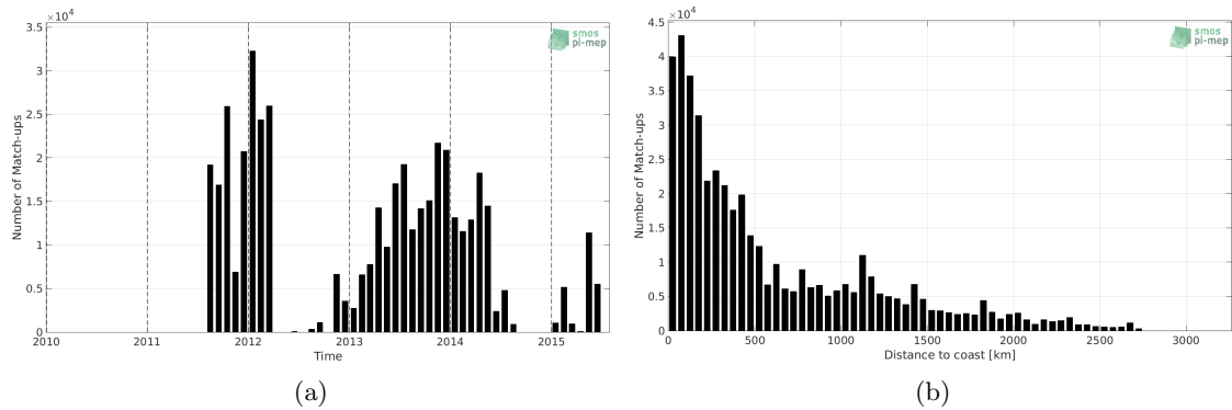
Figure 1: Number of match-ups between TSG-GOSUD-Sailing-ship and Aquarius-L3-OR-V5-MONTHLY-RAIN-MASK-1DEG SSS as a function of time (a) and as function of the distance to coast (b) over the Global Ocean Pi-MEP region and for the full satellite product period.
