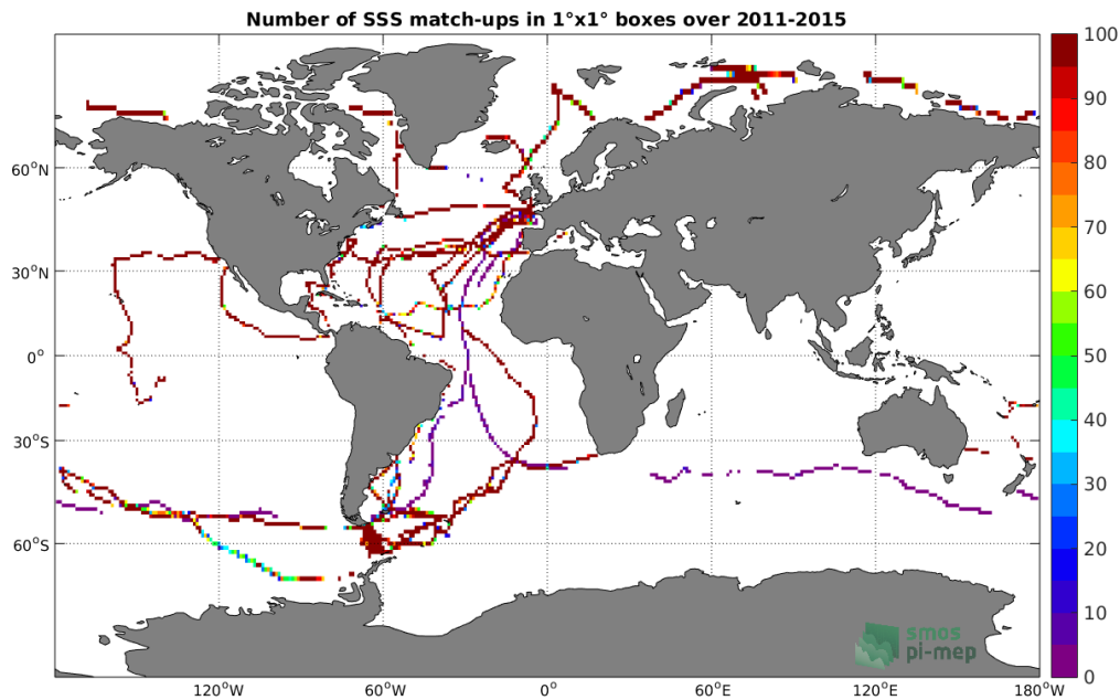
Figure 4: Number of SSS match-ups between TSG-GOSUD-Sailing-ship SSS and the Aquarius-L3-OR-V5-MONTHLY-RAIN-MASK-1DEG SSS product for the Global Ocean Pi-MEP region over 1^\circ \times 1^\circ boxes and for the full satellite product period.
