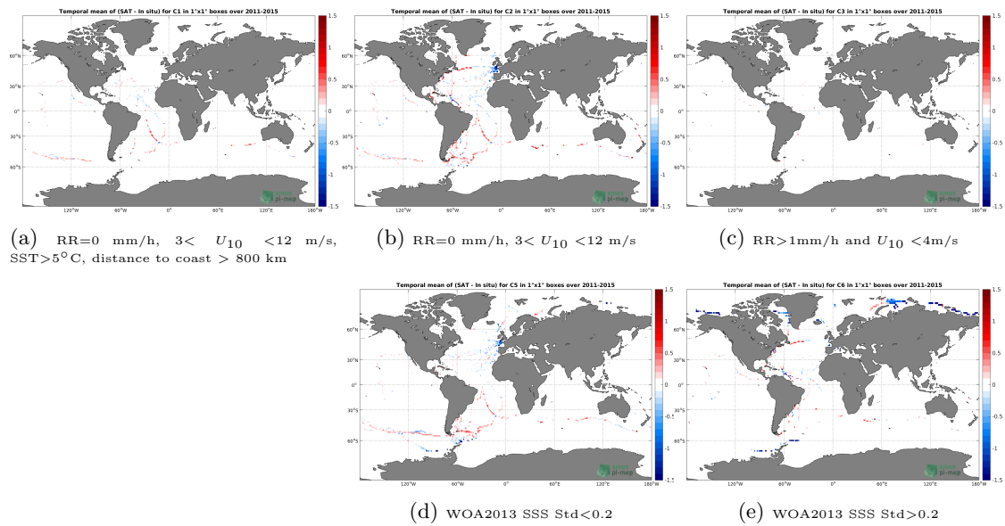
Figure 12: Temporal mean gridded over spatial boxes of size 1^\circ \times 1^\circ of \Delta SSS (Aquarius-L3-OR-V5-MONTHLY-RAIN-MASK-1DEG - TSG-GOSUD-Sailing-ship) for 5 different subdatasets corresponding to:RR=0 mm/h, 3 < U_{10} < 12 m/s, SST >5^\circ C, distance to coast > 800 km (a), RR=0 mm/h, 3 < U_{10} < 12 m/s (b), RR >1 mm/h and U_{10} < 4 m/s (c), WOA2013 SSS Std <0.2 (d), WOA2013 SSS Std >0.2 (e).
