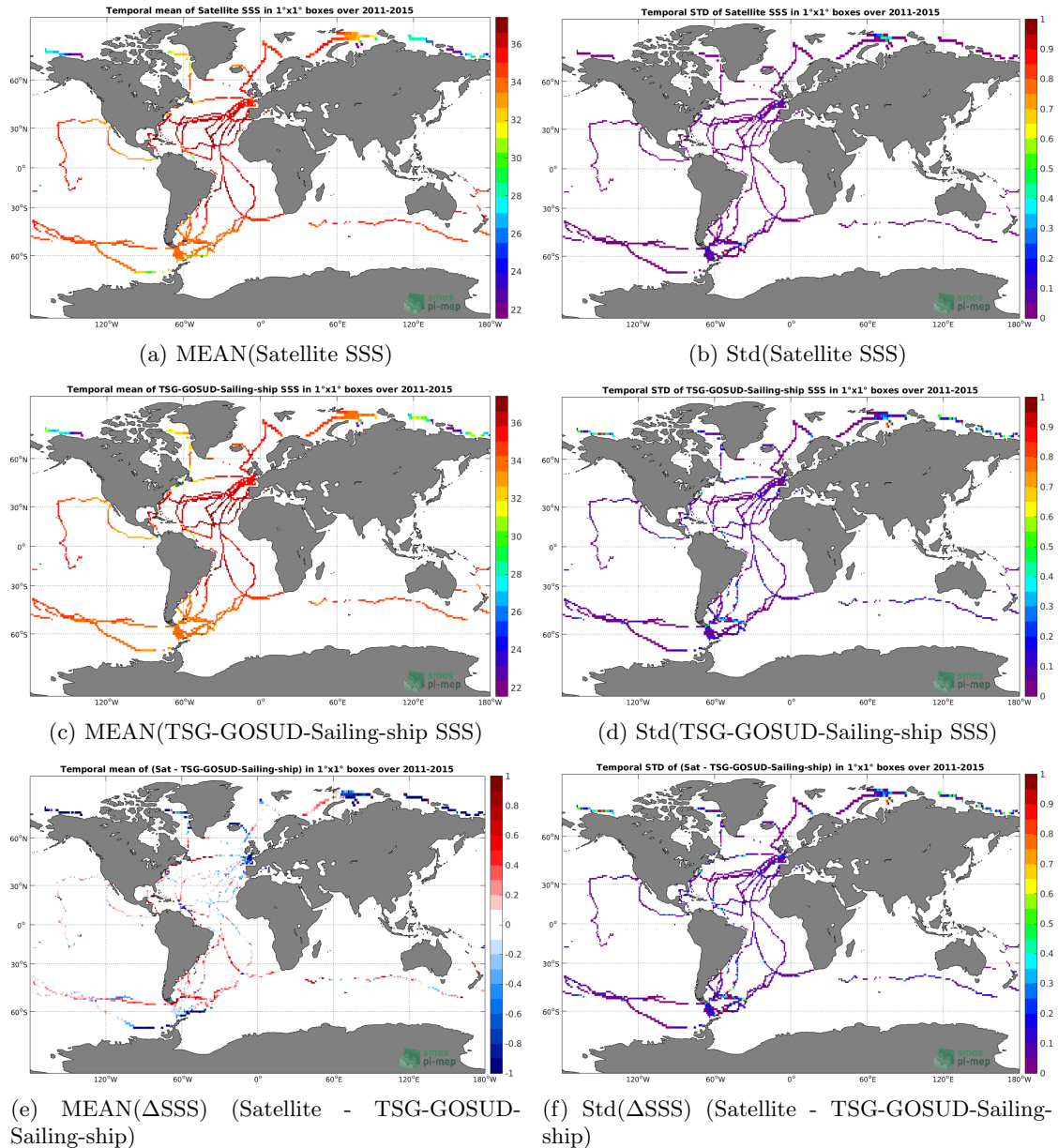
Figure 6: Temporal mean (left) and Std (right) of SSS from Aquarius-L3-OR-V5-MONTHLY-RAIN-MASK-1DEG (top), TSG-GOSUD-Sailing-ship (middle), and of \Delta SSS (Satellite - TSG-GOSUD-Sailing-ship). Only match-up pairs are used to generate these maps.
