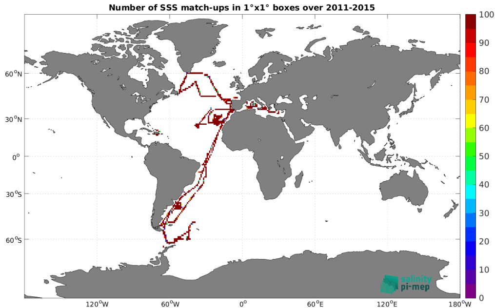
Figure 5: Number of SSS match-ups between TSG (CSIC-UTM) SSS and the Aquarius SSS L3 OR v5 - Monthly - Rain mask (NASA-GSFC) SSS product for the Global Ocean Pi-MEP region over 1^\circ \times 1^\circ boxes and for the full satellite product period.
