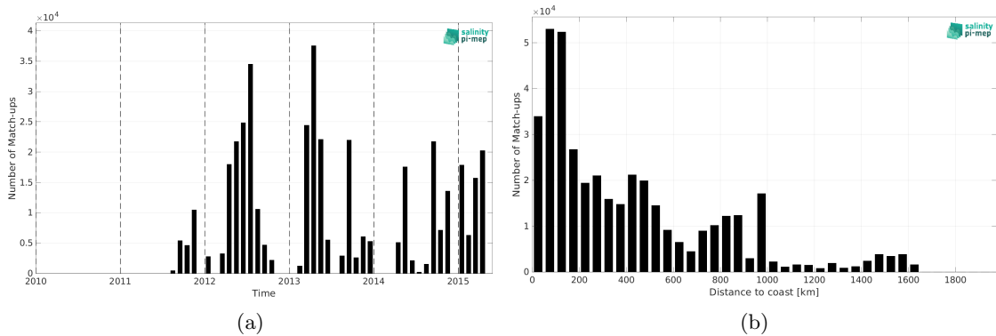
Figure 2: Number of match-ups between TSG (CSIC-UTM) and Aquarius SSS L3 OR v5 - Monthly - Rain mask (NASA-GSFC) SSS as a function of time (a) and as function of the distance to coast (b) over the Global Ocean Pi-MEP region and for the full satellite product period.
