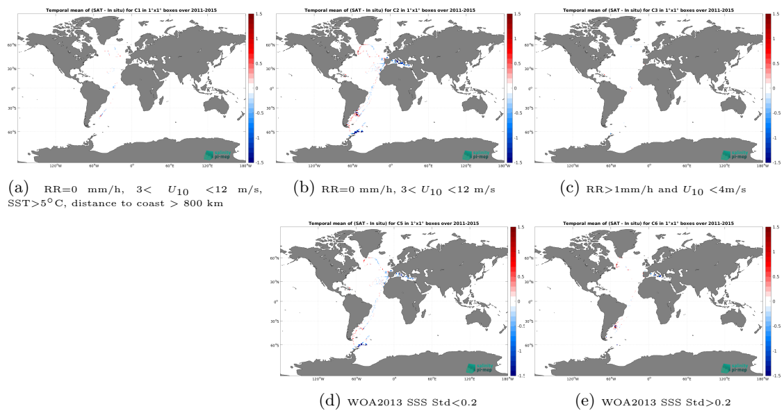
Figure 14: Temporal mean gridded over spatial boxes of size 1^\circ \times 1^\circ of \Delta\text{SSS} (Aquarius SSS L3 OR v5 - Monthly - Rain mask (NASA-GSFC) - TSG (CSIC-UTM)) for 5 different subdatasets corresponding to:RR=0 mm/h, 3 < U_{10} < 12 m/s, SST > 5^\circ\text{C} , distance to coast > 800 km (a), RR=0 mm/h, 3 < U_{10} < 12 m/s (b), RR > 1 mm/h and U_{10} < 4 m/s (c), WOA2013 SSS Std < 0.2 (d), WOA2013 SSS Std > 0.2 (e).
