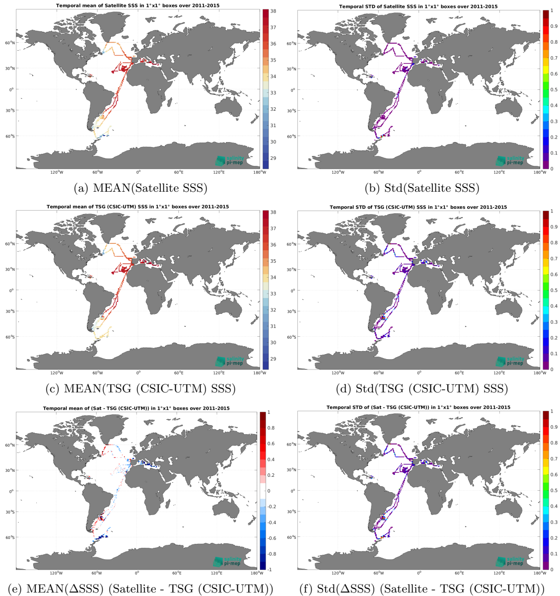
Figure 7: Temporal mean (left) and Std (right) of SSS from Aquarius SSS L3 OR v5 - Monthly - Rain mask (NASA-GSFC) (top), TSG (CSIC-UTM) (middle), and of \Delta SSS (Satellite - TSG (CSIC-UTM)). Only match-up pairs are used to generate these maps.
