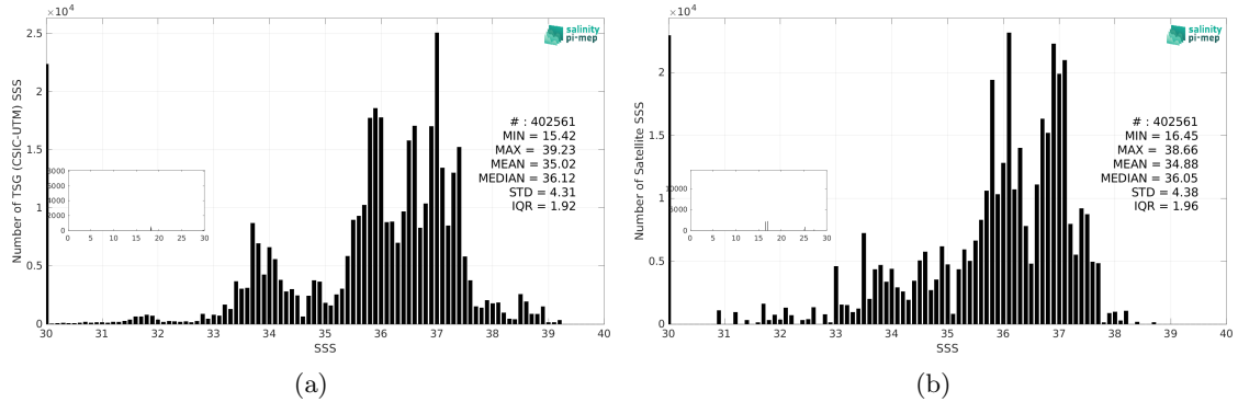
Figure 3: Histograms of SSS from TSG (CSIC-UTM) (a) and Aquarius SSS L3 OR v5 - Monthly - Rain mask (NASA-GSFC) (b) considering all match-up pairs per bins of 0.1 over the Global Ocean Pi-MEP region and for the full satellite product period.
