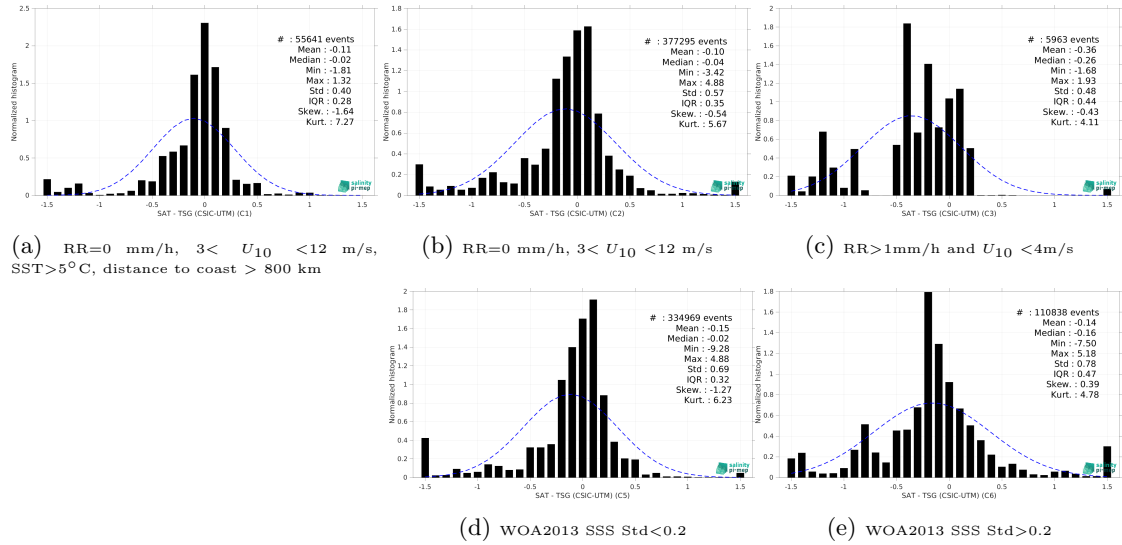
Figure 13: Normalized histogram of \Delta\text{SSS} (Aquarius SSS L3 OR v5 - Monthly - Rain mask (NASA-GSFC) - TSG (CSIC-UTM)) for 5 different subdatasets corresponding to: RR=0 mm/h, 3 < U_{10} < 12 m/s, SST > 5^\circ\text{C} , distance to coast > 800 km (a), RR=0 mm/h, 3 < U_{10} < 12 m/s (b), RR > 1 mm/h and U_{10} < 4 m/s (c), WOA2013 SSS Std < 0.2 (d), WOA2013 SSS Std > 0.2 (e).
