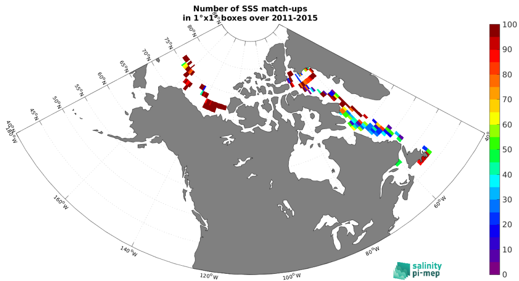
Figure 5: Number of SSS match-ups between TSG (Amundsen) SSS and the Aquarius SSS L3 OR v5 - Monthly - Rain mask (NASA-GSFC) SSS product for the Global Ocean Pi-MEP region over 1^\circ \times 1^\circ boxes and for the full satellite product period.
