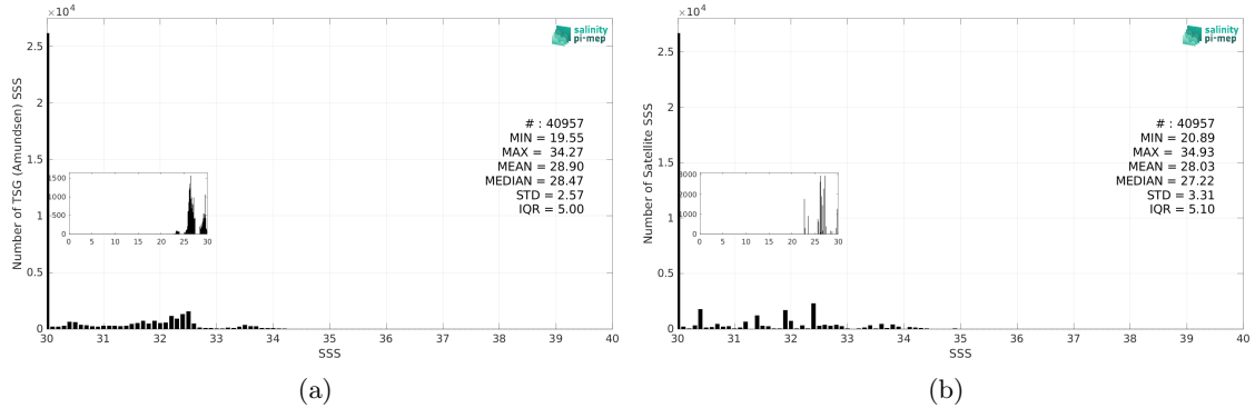
Figure 3: Histograms of SSS from TSG (Amundsen) (a) and Aquarius SSS L3 OR v5 - Monthly - Rain mask (NASA-GSFC) (b) considering all match-up pairs per bins of 0.1 over the Global Ocean Pi-MEP region and for the full satellite product period.
