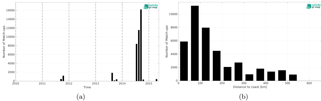
Figure 2: Number of match-ups between TSG (Amundsen) and Aquarius SSS L3 OR v5 - Monthly - Rain mask (NASA-GSFC) SSS as a function of time (a) and as function of the distance to coast (b) over the Global Ocean Pi-MEP region and for the full satellite product period.
