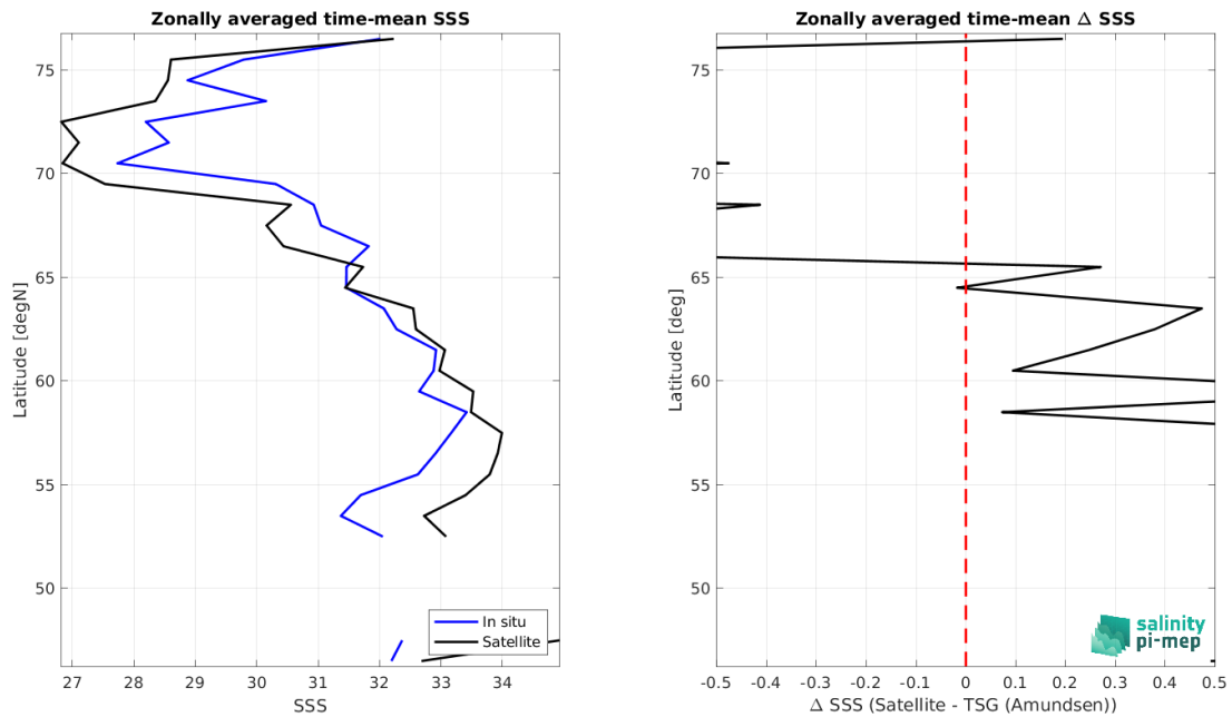
Figure 8: Left panel: Zonal mean SSS from Aquarius SSS L3 OR v5 - Monthly - Rain mask (NASA-GSFC) satellite product (black) and from TSG (Amundsen) (blue). Right panel: Zonal mean of \Delta SSS (Satellite - TSG (Amundsen)) for all the collected Pi-MEP match-up pairs estimated over the full satellite product period.
