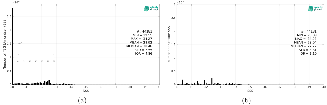
Figure 2: Histograms of SSS from TSG (Amundsen) (a) and Aquarius SSS L3 OR v5 - Monthly - Rain mask (NASA-GSFC) (b) considering all match-up pairs per bins of 0.1 over the Global Ocean Pi-MEP region and for the full satellite product period.
