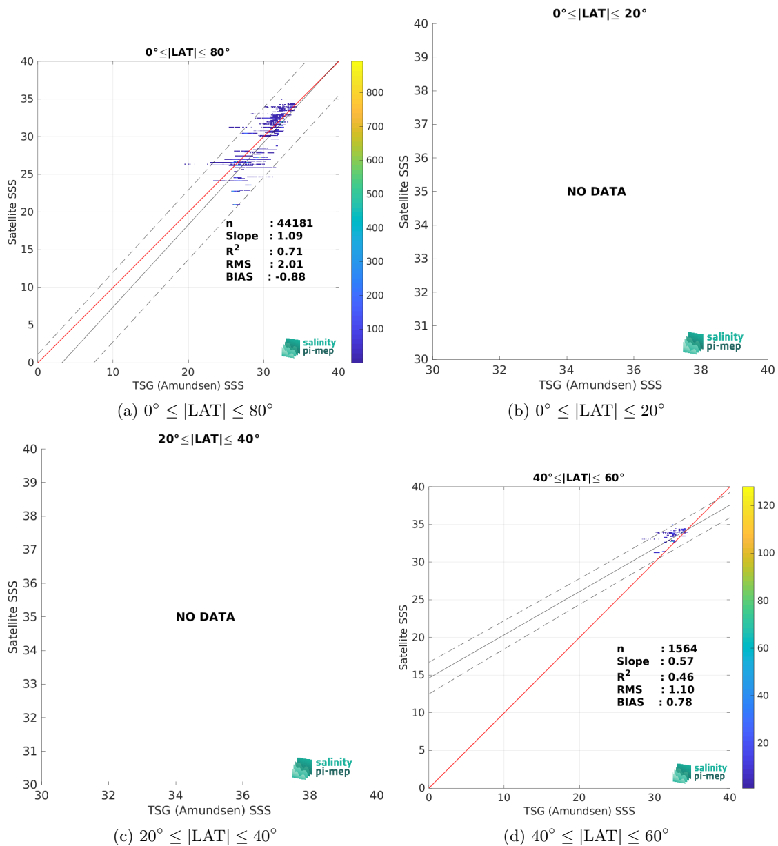
Figure 9: Contour maps of the concentration of Aquarius SSS L3 OR v5 - Monthly - Rain mask (NASA-GSFC) SSS (y-axis) versus TSG (Amundsen) SSS (x-axis) at match-up pairs for different latitude bands. For each plot, the red line shows x=y . The black thin and dashed lines indicate a linear fit through the data cloud and the \pm 95\% confidence levels, respectively. The number match-up pairs n , the slope and R^2 coefficient of the linear fit, the root mean square (RMS) and the mean bias between satellite and in situ data are indicated for each latitude band in each plots.
