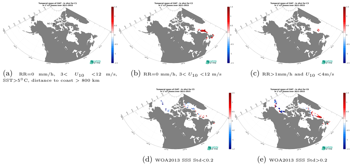
Figure 12: Temporal mean gridded over spatial boxes of size 1^{\circ}\times 1^{\circ} of \Delta\text{SSS} (Aquarius SSS L3 OR v5 - Monthly - Rain mask (NASA-GSFC) - TSG (Amundsen)) for 5 different subdatasets corresponding to:RR=0 mm/h, 3 < U_{10} < 12 m/s, SST >5^{\circ}\text{C} , distance to coast > 800 km (a), RR=0 mm/h, 3 < U_{10} < 12 m/s (b), RR >1 mm/h and U_{10} < 4 m/s (c), WOA2013 SSS Std <0.2 (d), WOA2013 SSS Std >0.2 (e).
