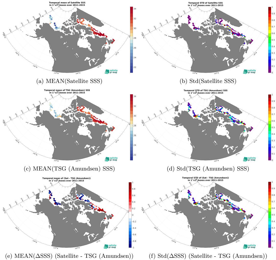
Figure 6: Temporal mean (left) and Std (right) of SSS from Aquarius SSS L3 OR v5 - Monthly - Rain mask (NASA-GSFC) (top), TSG (Amundsen) (middle), and of \Delta SSS (Satellite - TSG (Amundsen)). Only match-up pairs are used to generate these maps.
