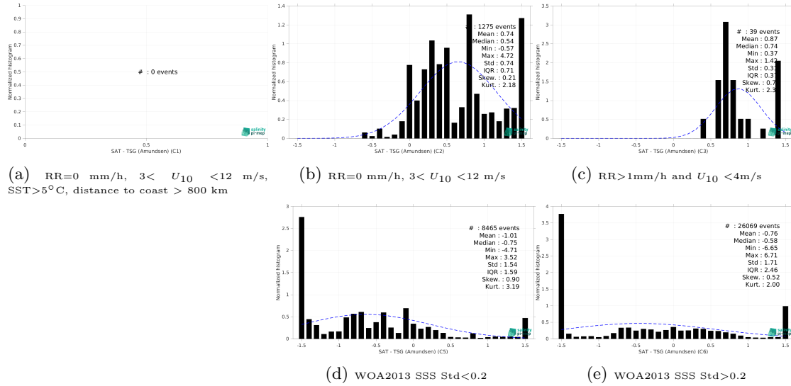
Figure 13: Normalized histogram of \Delta SSS (Aquarius SSS L3 OR v5 - Monthly - Rain mask (NASA-GSFC) - TSG (Amundsen)) for 5 different subdatasets corresponding to: RR=0 mm/h, 3 < U_{10} < 12 m/s, SST > 5°C, distance to coast > 800 km (a), RR=0 mm/h, 3 < U_{10} < 12 m/s (b), RR > 1mm/h and U_{10} < 4 m/s (c), WOA2013 SSS Std < 0.2 (d), WOA2013 SSS Std > 0.2 (e).
