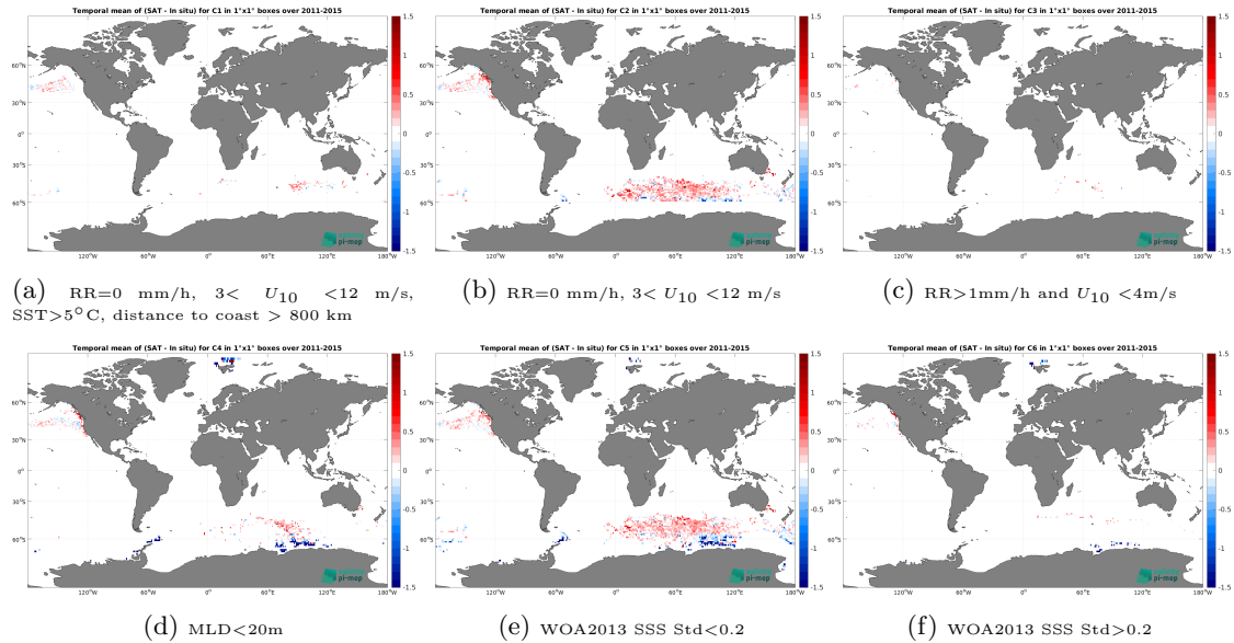
Figure 12: Temporal mean gridded over spatial boxes of size 1^{\circ}\times 1^{\circ} of \Delta\text{SSS} (Aquarius SSS L3 OR v5 - Monthly - Rain mask (NASA-GSFC) - Marine mammals) for 6 different subdatasets corresponding to:RR=0 mm/h, 3 < U_{10} < 12 m/s, SST > 5^{\circ}\text{C} , distance to coast > 800 km (a), RR=0 mm/h, 3 < U_{10} < 12 m/s (b), RR > 1\text{mm/h} and U_{10} < 4\text{m/s} (c),MLD < 20\text{m} (d),WOA2013 SSS Std < 0.2 (e),WOA2013 SSS Std > 0.2 (f).
