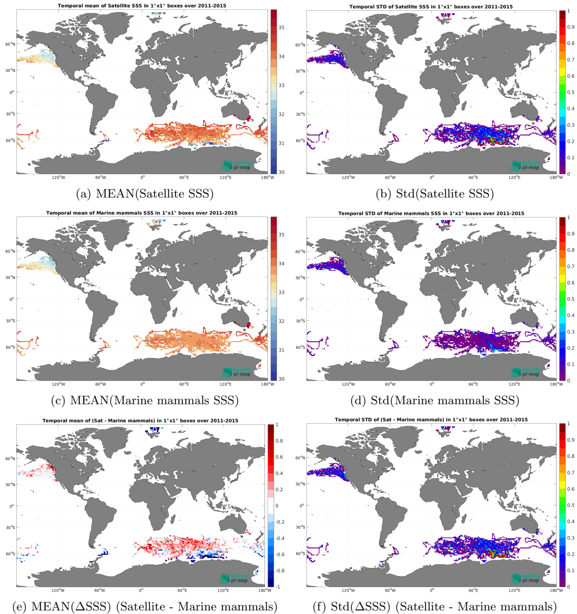
Figure 6: Temporal mean (left) and Std (right) of SSS from Aquarius SSS L3 OR v5 - Monthly - Rain mask (NASA-GSFC) (top), Marine mammals (middle), and of \Delta SSS (Satellite - Marine mammals). Only match-up pairs are used to generate these maps.
