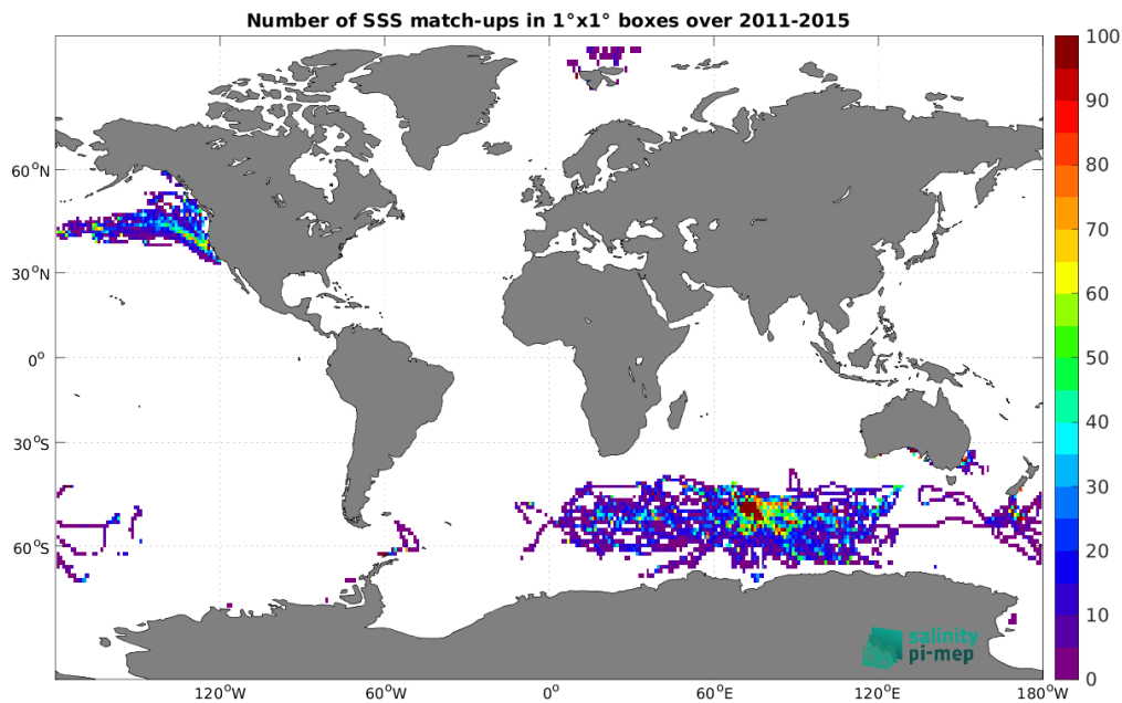
Figure 4: Number of SSS match-ups between Marine mammals SSS and the Aquarius SSS L3 OR v5 - Monthly - Rain mask (NASA-GSFC) SSS product for the Global Ocean Pi-MEP region over 1^\circ \times 1^\circ boxes and for the full satellite product period.
