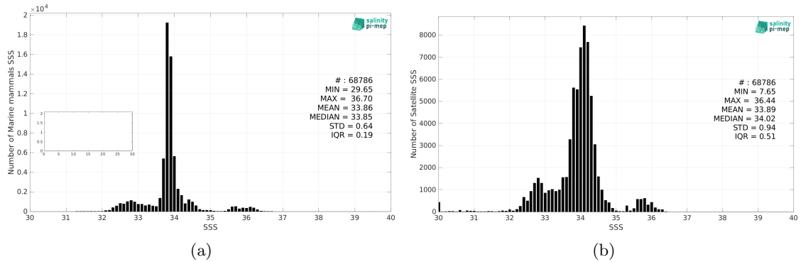
Figure 2: Histograms of SSS from Marine mammals (a) and Aquarius SSS L3 OR v5 - Monthly - Rain mask (NASA-GSFC) (b) considering all match-up pairs per bins of 0.1 over the Global Ocean Pi-MEP region and for the full satellite product period.
