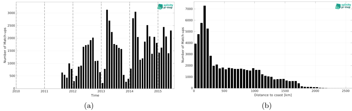
Figure 1: Number of match-ups between Marine mammals and Aquarius SSS L3 OR v5 - Monthly - Rain mask (NASA-GSFC) SSS as a function of time (a) and as function of the distance to coast (b) over the Global Ocean Pi-MEP region and for the full satellite product period.
