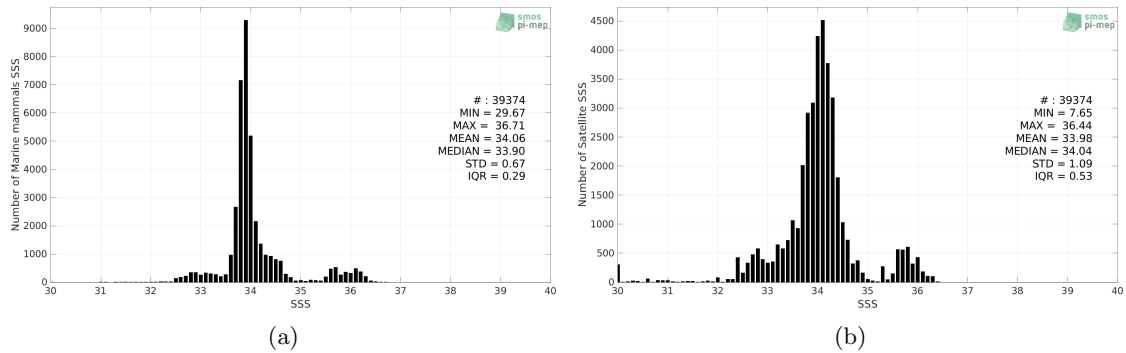
Figure 2: Histograms of SSS from Marine mammals (a) and Aquarius SSS L3 OR v5 - Monthly - Rain mask (NASA-GSFC) (b) considering all match-up pairs per bins of 0.1 over the Global Ocean Pi-MEP region and for the full satellite product period.
