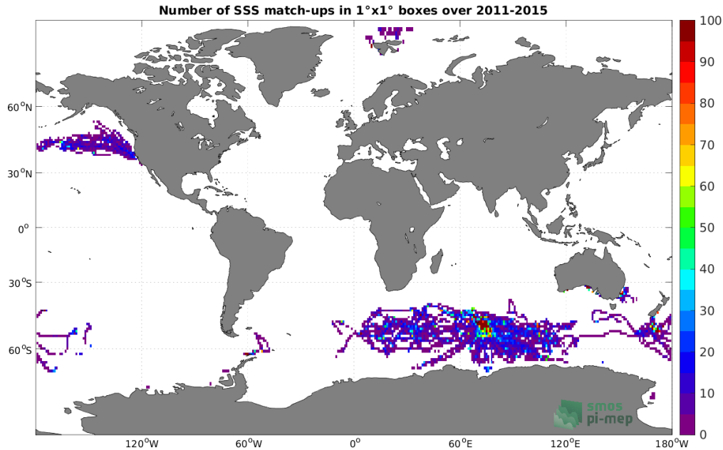
Figure 4: Number of SSS match-ups between Marine mammals SSS and the Aquarius SSS L3 OR v5 - Monthly - Rain mask (NASA-GSFC) SSS product for the Global Ocean Pi-MEP region over 1^{\circ} \times 1^{\circ} boxes and for the full satellite product period.
