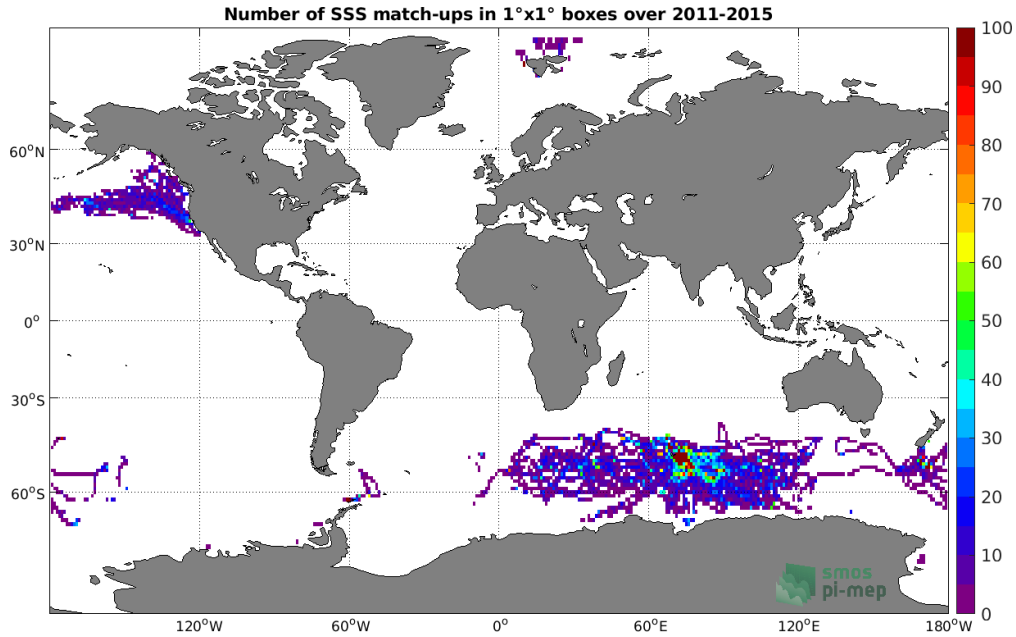
Figure 4: Number of SSS match-ups between Marine mammals SSS and the Aquarius SSS L3 OR v5 - Monthly - Rain mask (NASA-GSFC) SSS product for the Global Ocean Pi-MEP region over 1°×1° boxes and for the full satellite product period.
