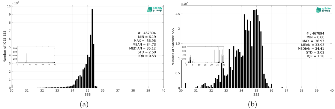
Figure 3: Histograms of SSS from ICES (a) and Aquarius SSS L3 OR v5 - Monthly - Rain mask (NASA-GSFC) (b) considering all match-up pairs per bins of 0.1 over the Global Ocean Pi-MEP region and for the full satellite product period.
