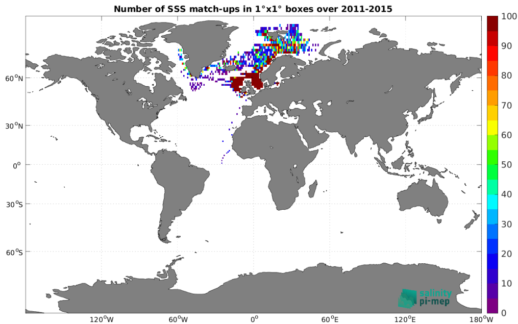
Figure 5: Number of SSS match-ups between ICES SSS and the Aquarius SSS L3 OR v5 - Monthly - Rain mask (NASA-GSFC) SSS product for the Global Ocean Pi-MEP region over 1^\circ \times 1^\circ boxes and for the full satellite product period.
