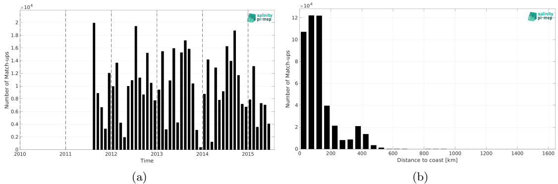
Figure 2: Number of match-ups between ICES and Aquarius SSS L3 OR v5 - Monthly - Rain mask (NASA-GSFC) SSS as a function of time (a) and as function of the distance to coast (b) over the Global Ocean Pi-MEP region and for the full satellite product period.
