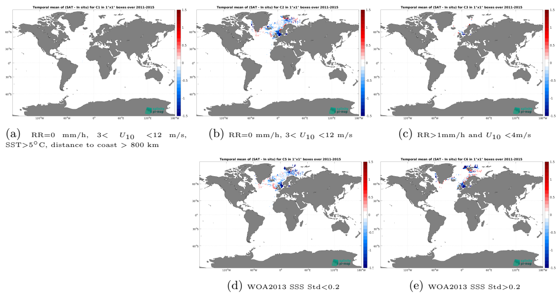
Figure 14: Temporal mean gridded over spatial boxes of size 1^\circ \times 1^\circ of \Delta SSS (Aquarius SSS L3 OR v5 - Monthly - Rain mask (NASA-GSFC) - ICES) for 5 different subdatasets corresponding to: RR=0 mm/h, 3 < U_{10} < 12 m/s, SST > 5^\circ\text{C} , distance to coast > 800 km (a), RR=0 mm/h, 3 < U_{10} < 12 m/s (b), RR > 1 mm/h and U_{10} < 4 m/s (c), WOA2013 SSS Std < 0.2 (d), WOA2013 SSS Std > 0.2 (e).
