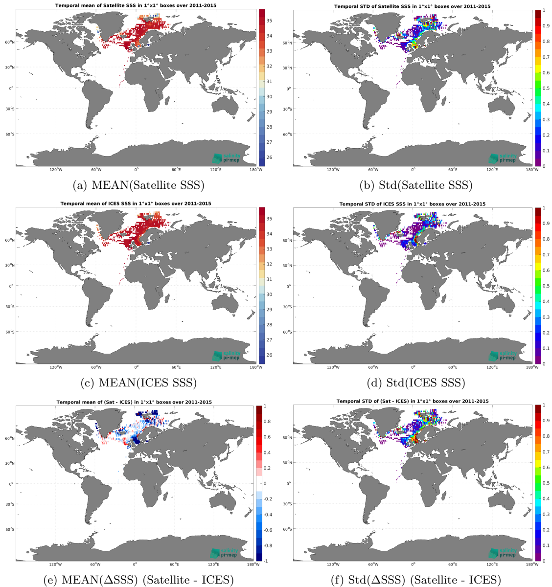
Figure 7: Temporal mean (left) and Std (right) of SSS from Aquarius SSS L3 OR v5 - Monthly - Rain mask (NASA-GSFC) (top), ICES (middle), and of \Delta SSS (Satellite - ICES). Only match-up pairs are used to generate these maps.
