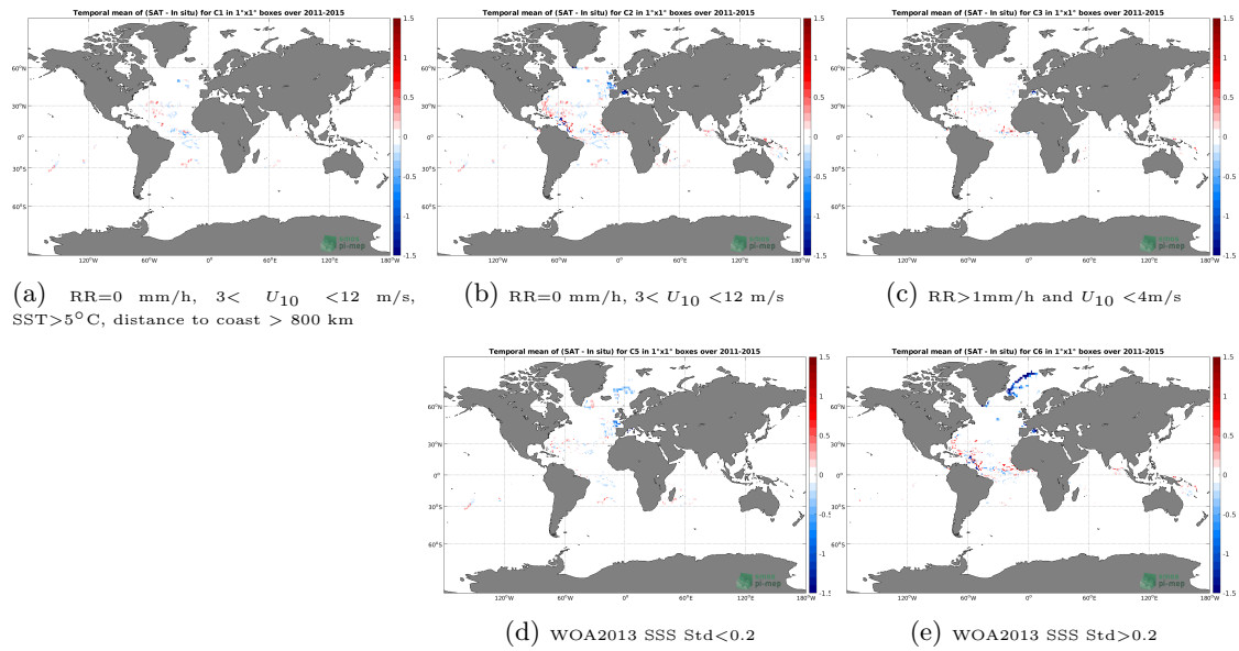
Figure 11: Temporal mean gridded over spatial boxes of size 1^\circ \times 1^\circ of \Delta SSS (Aquarius SSS L3 OR v5 - Monthly - Rain mask (NASA-GSFC) - Surface drifters) for 5 different subdatasets corresponding to:RR=0 mm/h, 3 < U_{10} < 12 m/s, SST >5^\circ\text{C} , distance to coast > 800 km (a), RR=0 mm/h, 3 < U_{10} < 12 m/s (b), RR >1 mm/h and U_{10} < 4 m/s (c), WOA2013 SSS Std <0.2 (d), WOA2013 SSS Std >0.2 (e).
