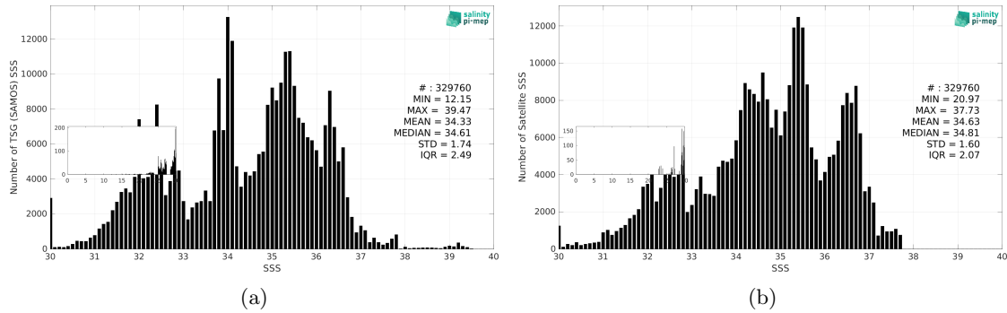
Figure 3: Histograms of SSS from TSG (SAMOS) (a) and Aquarius SSS L3 CAP v5 - 7-Day running (JPL) (b) considering all match-up pairs per bins of 0.1 over the Global Ocean Pi-MEP region and for the full satellite product period.
