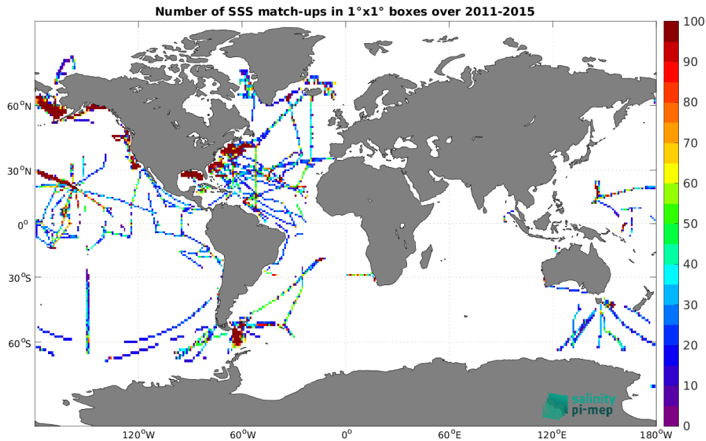
Figure 5: Number of SSS match-ups between TSG (SAMOS) SSS and the Aquarius SSS L3 CAP v5 - 7-Day running (JPL) SSS product for the Global Ocean Pi-MEP region over 1^\circ \times 1^\circ boxes and for the full satellite product period.
