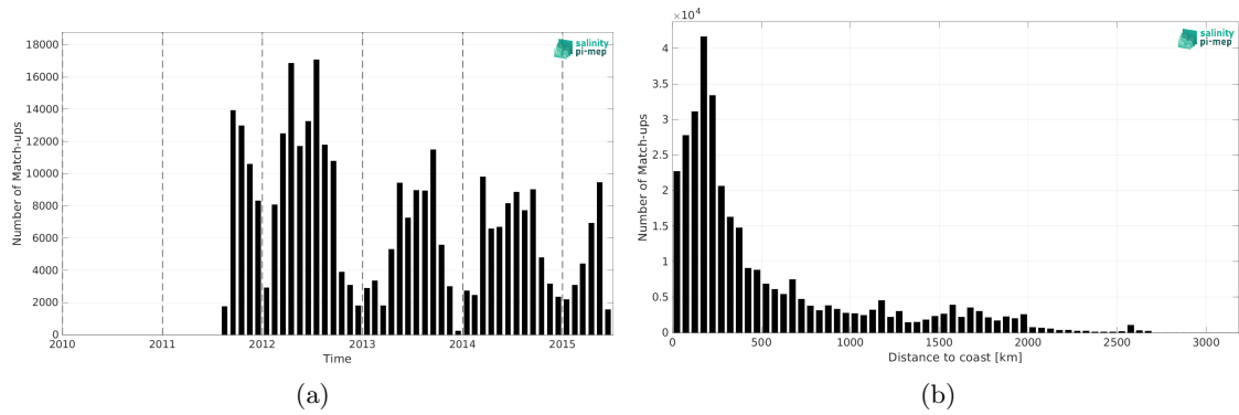
Figure 2: Number of match-ups between TSG (SAMOS) and Aquarius SSS L3 CAP v5 - 7-Day running (JPL) SSS as a function of time (a) and as function of the distance to coast (b) over the Global Ocean Pi-MEP region and for the full satellite product period.
