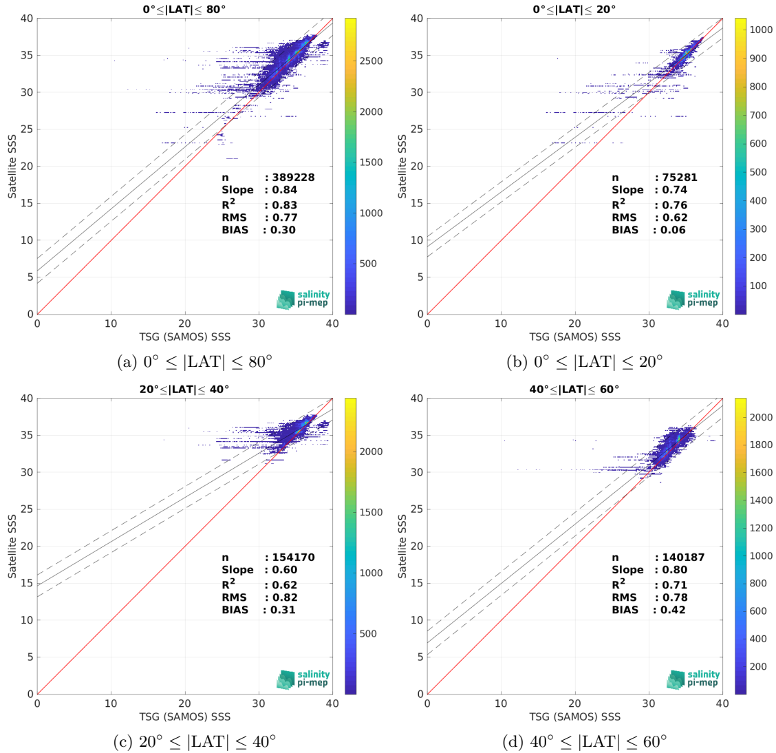
Figure 9: Contour maps of the concentration of Aquarius SSS L3 CAP v5 - 7-Day running (JPL) SSS (y-axis) versus TSG (SAMOS) SSS (x-axis) at match-up pairs for different latitude bands. For each plot, the red line shows x=y . The black thin and dashed lines indicate a linear fit through the data cloud and the \pm 95\% confidence levels, respectively. The number match-up pairs n , the slope and R^2 coefficient of the linear fit, the root mean square (RMS) and the mean bias between satellite and in situ data are indicated for each latitude band in each plots.
