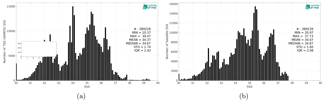
Figure 2: Histograms of SSS from TSG (SAMOS) (a) and Aquarius SSS L3 CAP v5 - 7-Day running (JPL) (b) considering all match-up pairs per bins of 0.1 over the Global Ocean Pi-MEP region and for the full satellite product period.
