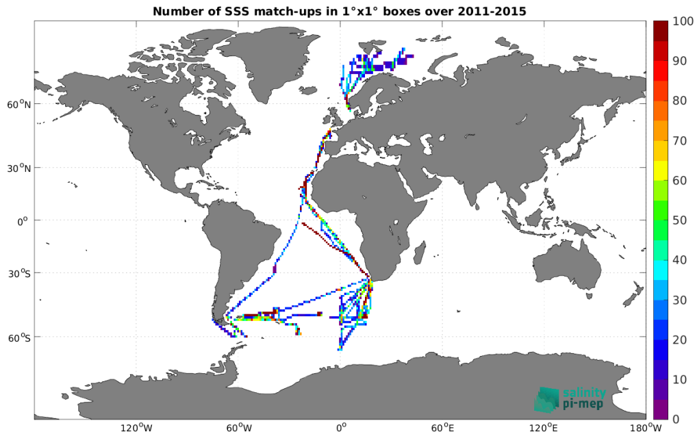
Figure 5: Number of SSS match-ups between TSG (Polarstern) SSS and the Aquarius SSS L3 CAP v5 - 7-Day running (JPL) SSS product for the Global Ocean Pi-MEP region over 1^\circ \times 1^\circ boxes and for the full satellite product period.
