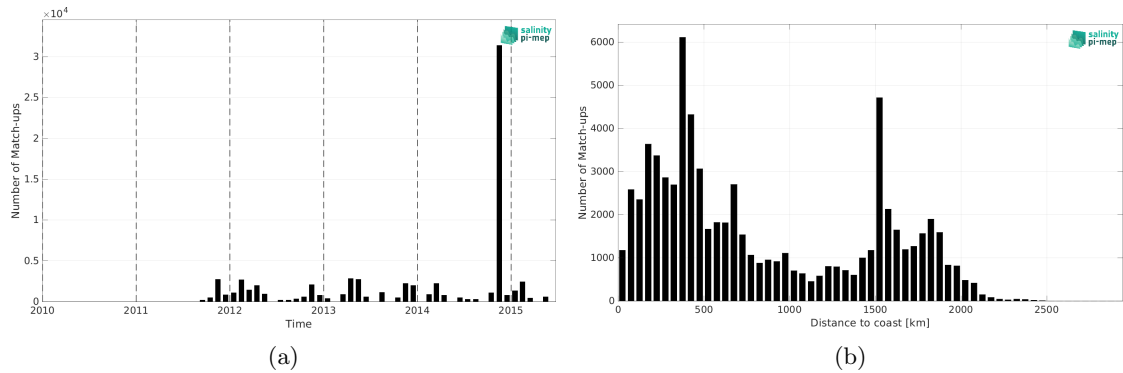
Figure 2: Number of match-ups between TSG (Polarstern) and Aquarius SSS L3 CAP v5 - 7-Day running (JPL) SSS as a function of time (a) and as function of the distance to coast (b) over the Global Ocean Pi-MEP region and for the full satellite product period.
