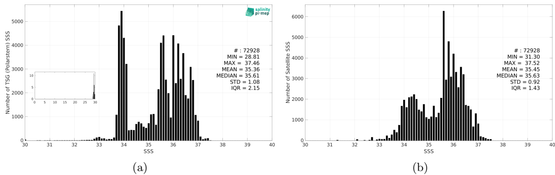
Figure 3: Histograms of SSS from TSG (Polarstern) (a) and Aquarius SSS L3 CAP v5 - 7-Day running (JPL) (b) considering all match-up pairs per bins of 0.1 over the Global Ocean Pi-MEP region and for the full satellite product period.
