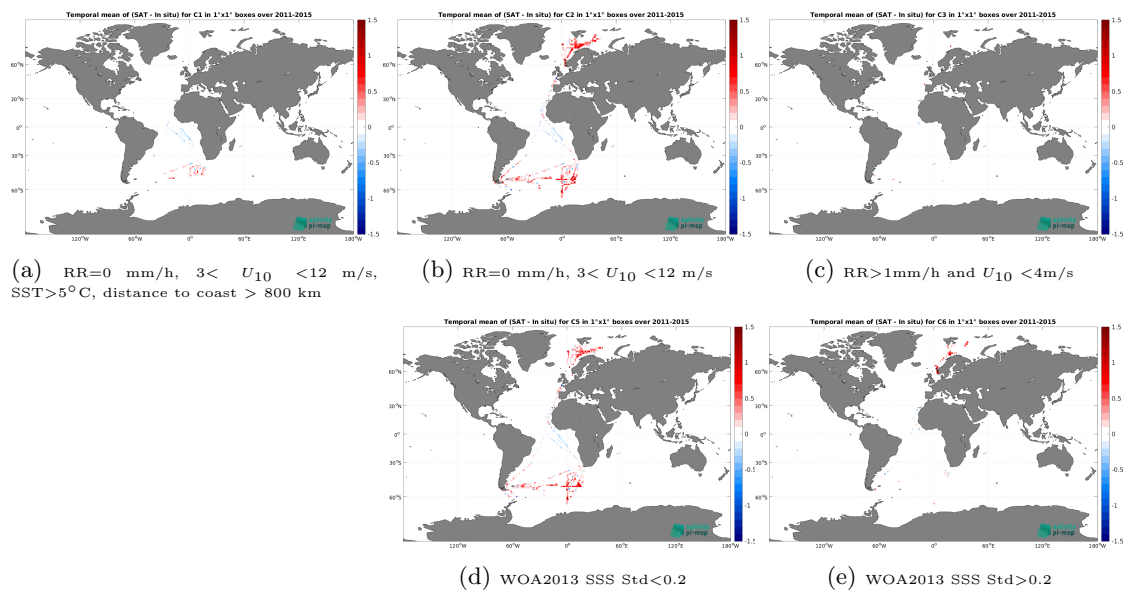
Figure 14: Temporal mean gridded over spatial boxes of size 1^\circ \times 1^\circ of \Delta SSS (Aquarius SSS L3 CAP v5 - 7-Day running (JPL) - TSG (Polarstern)) for 5 different subdatasets corresponding to: RR=0 mm/h, 3 < U_{10} < 12 m/s, SST > 5^\circ\text{C} , distance to coast > 800 km (a), RR=0 mm/h, 3 < U_{10} < 12 m/s (b), RR > 1 mm/h and U_{10} < 4 m/s (c), WOA2013 SSS Std < 0.2 (d), WOA2013 SSS Std > 0.2 (e).
