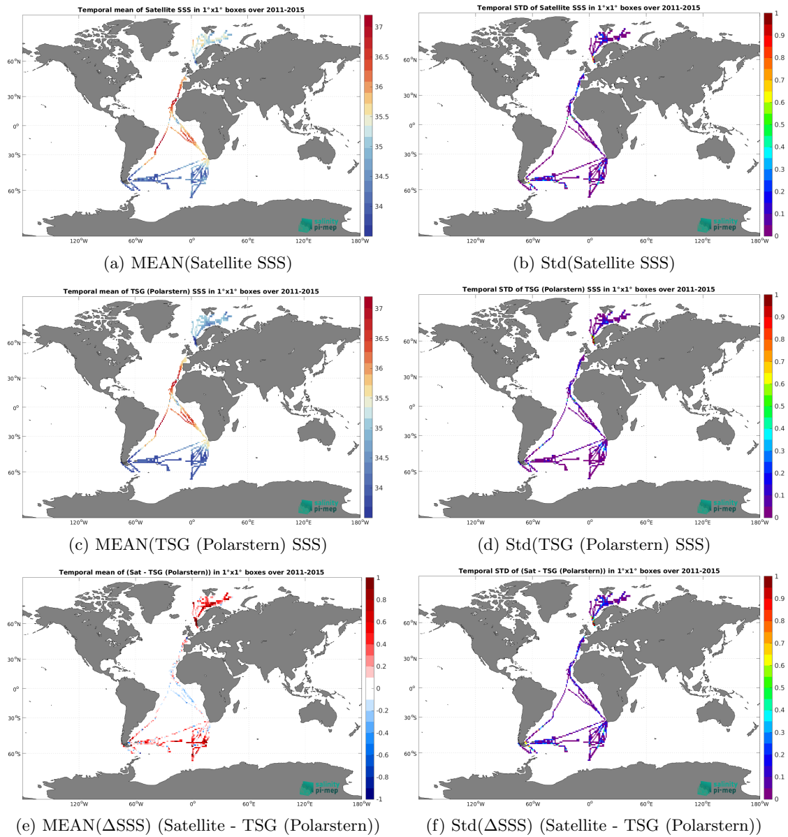
Figure 7: Temporal mean (left) and Std (right) of SSS from Aquarius SSS L3 CAP v5 - 7-Day running (JPL) (top), TSG (Polarstern) (middle), and of \Delta SSS (Satellite - TSG (Polarstern)). Only match-up pairs are used to generate these maps.
