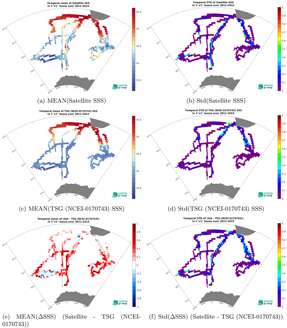
Figure 7: Temporal mean (left) and Std (right) of SSS from Aquarius SSS L3 CAP v5 - 7-Day running (JPL) (top), TSG (NCEI-0170743) (middle), and of \Delta SSS (Satellite - TSG (NCEI-0170743)). Only match-up pairs are used to generate these maps.
