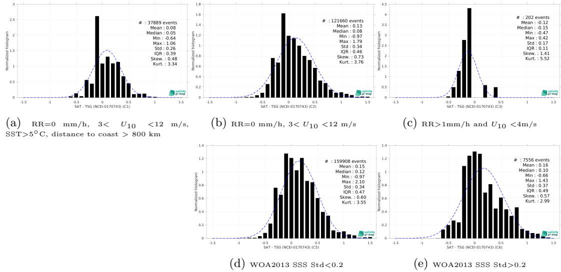
Figure 15: Normalized histogram of \Delta SSS (Aquarius SSS L3 CAP v5 - 7-Day running (JPL) - TSG (NCEI-0170743)) for 5 different subdatasets corresponding to: RR=0 mm/h, 3 < U_{10} < 12 m/s, SST > 5°C, distance to coast > 800 km (a), RR=0 mm/h, 3 < U_{10} < 12 m/s (b), RR > 1mm/h and U_{10} < 4 m/s (c), WOA2013 SSS Std < 0.2 (d), WOA2013 SSS Std > 0.2 (e).
