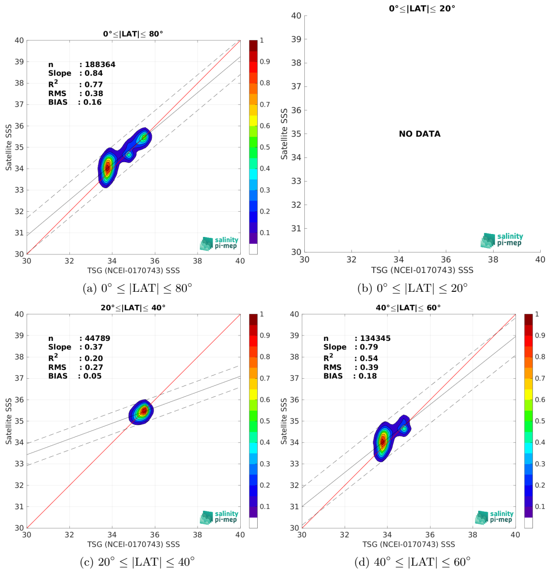
Figure 10: Contour maps of the concentration of Aquarius SSS L3 CAP v5 - 7-Day running (JPL) SSS (y-axis) versus TSG (NCEI-0170743) SSS (x-axis) at match-up pairs for different latitude bands. For each plot, the red line shows x=y . The black thin and dashed lines indicate a linear fit through the data cloud and the \pm 95\% confidence levels, respectively. The number match-up pairs n , the slope and R^2 coefficient of the linear fit, the root mean square (RMS) and the mean bias between satellite and in situ data are indicated for each latitude band in each plots.
