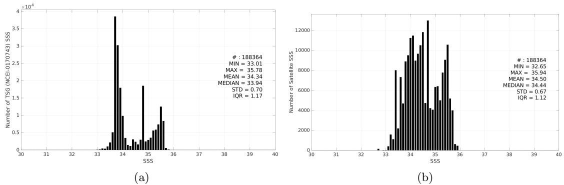
Figure 3: Histograms of SSS from TSG (NCEI-0170743) (a) and Aquarius SSS L3 CAP v5 - 7-Day running (JPL) (b) considering all match-up pairs per bins of 0.1 over the Global Ocean Pi-MEP region and for the full satellite product period.
