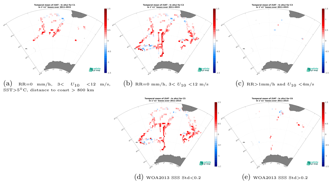
Figure 14: Temporal mean gridded over spatial boxes of size 1^\circ \times 1^\circ of \Delta SSS (Aquarius SSS L3 CAP v5 - 7-Day running (JPL) - TSG (NCEI-0170743)) for 5 different subdatasets corresponding to: RR=0 mm/h, 3 < U_{10} < 12 m/s, SST > 5^\circ\text{C} , distance to coast > 800 km (a), RR=0 mm/h, 3 < U_{10} < 12 m/s (b), RR > 1 mm/h and U_{10} < 4 m/s (c), WOA2013 SSS Std < 0.2 (d), WOA2013 SSS Std > 0.2 (e).
