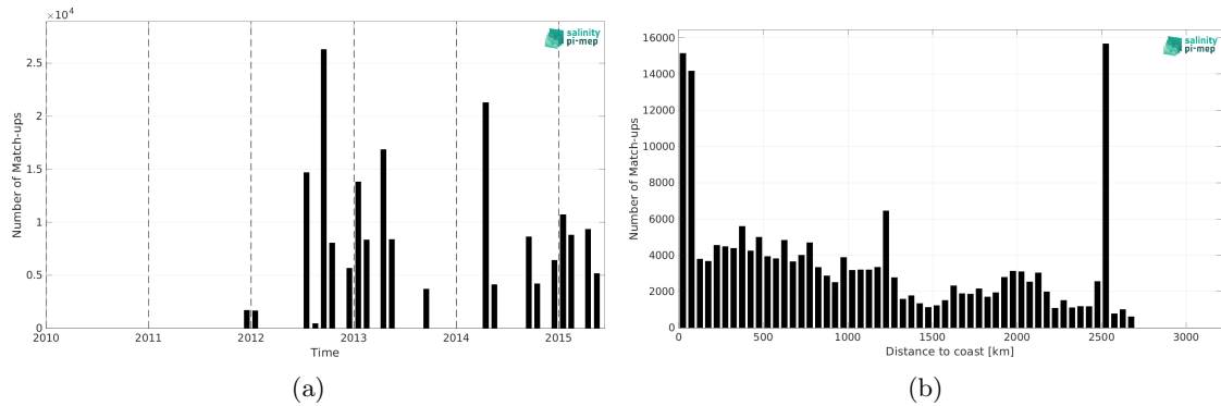
Figure 2: Number of match-ups between TSG (NCEI-0170743) and Aquarius SSS L3 CAP v5 - 7-Day running (JPL) SSS as a function of time (a) and as function of the distance to coast (b) over the Global Ocean Pi-MEP region and for the full satellite product period.
