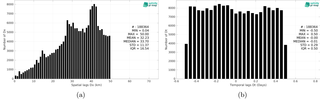
Figure 6: Histograms of the spatial (a) and temporal (b) lags between the location/time of the TSG (NCEI-0170743) measurement and the date of the corresponding Aquarius SSS L3 CAP v5 - 7-Day running (JPL) SSS pixel.
