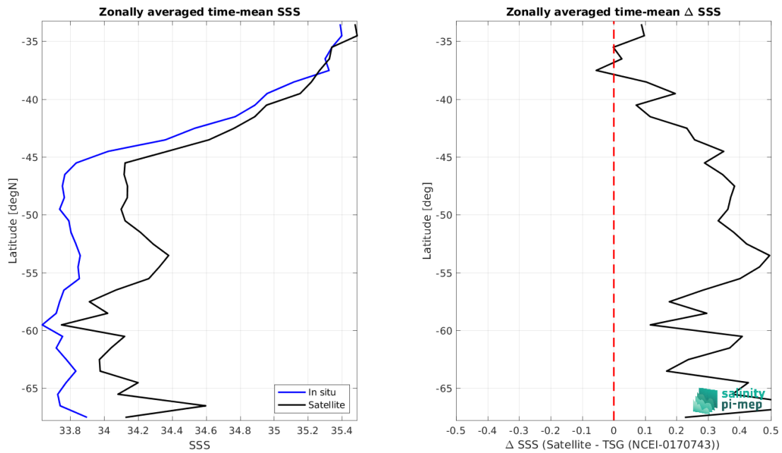
Figure 9: Left panel: Zonal mean SSS from Aquarius SSS L3 CAP v5 - 7-Day running (JPL) satellite product (black) and from TSG (NCEI-0170743) (blue). Right panel: Zonal mean of \Delta SSS (Satellite - TSG (NCEI-0170743)) for all the collected Pi-MEP match-up pairs estimated over the full satellite product period.
