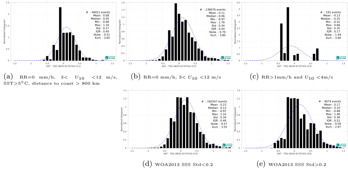
Figure 13: Normalized histogram of \Delta\text{SSS} (Aquarius SSS L3 CAP v5 - 7-Day running (JPL) - TSG (NCEI-0170743)) for 5 different subdatasets corresponding to: RR=0 mm/h, 3 < U_{10} < 12 m/s, SST>5°C, distance to coast > 800 km (a), RR=0 mm/h, 3 < U_{10} < 12 m/s (b), RR>1mm/h and U_{10} < 4 m/s (c), WOA2013 SSS Std<0.2 (d), WOA2013 SSS Std>0.2 (e).
