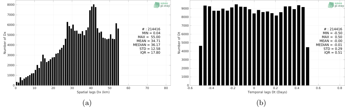
Figure 5: Histograms of the spatial (a) and temporal (b) lags between the location/time of the TSG (NCEI-0170743) measurement and the date of the corresponding Aquarius SSS L3 CAP v5 - 7-Day running (JPL) SSS pixel.
