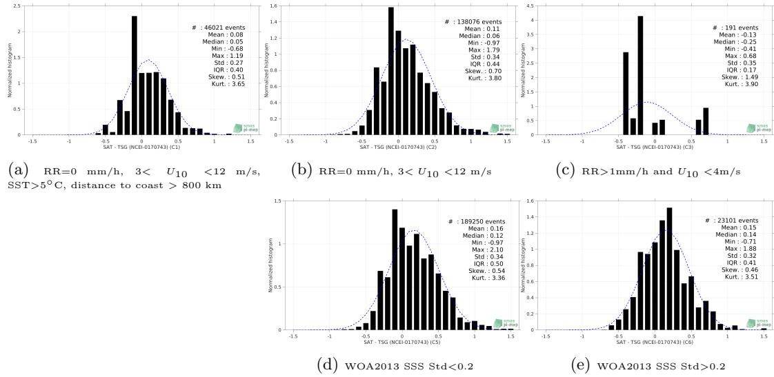
Figure 13: Normalized histogram of \Delta SSS (Aquarius SSS L3 CAP v5 - 7-Day running (JPL) - TSG (NCEI-0170743)) for 5 different subdatasets corresponding to: RR=0 mm/h, 3 < U_{10} < 12 m/s, SST>5°C, distance to coast > 800 km (a), RR=0 mm/h, 3 < U_{10} < 12 m/s (b), RR>1mm/h and U_{10} < 4 m/s (c), WOA2013 SSS Std<0.2 (d), WOA2013 SSS Std>0.2 (e).
