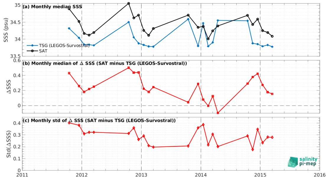
Figure 8: Time series of the monthly median SSS (top), median of \Delta SSS (Satellite - TSG (LEGOS-Survostral)) and Std of \Delta SSS (Satellite - TSG (LEGOS-Survostral)) over the Global Ocean Pi-MEP region considering all match-ups collected by the Pi-MEP.
