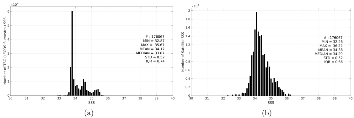
Figure 3: Histograms of SSS from TSG (LEGOS-Survostral) (a) and Aquarius SSS L3 CAP v5 - 7-Day running (JPL) (b) considering all match-up pairs per bins of 0.1 over the Global Ocean Pi-MEP region and for the full satellite product period.
