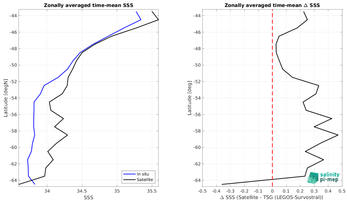
Figure 9: Left panel: Zonal mean SSS from Aquarius SSS L3 CAP v5 - 7-Day running (JPL) satellite product (black) and from TSG (LEGOS-Survostral) (blue). Right panel: Zonal mean of \Delta SSS (Satellite - TSG (LEGOS-Survostral)) for all the collected Pi-MEP match-up pairs estimated over the full satellite product period.
