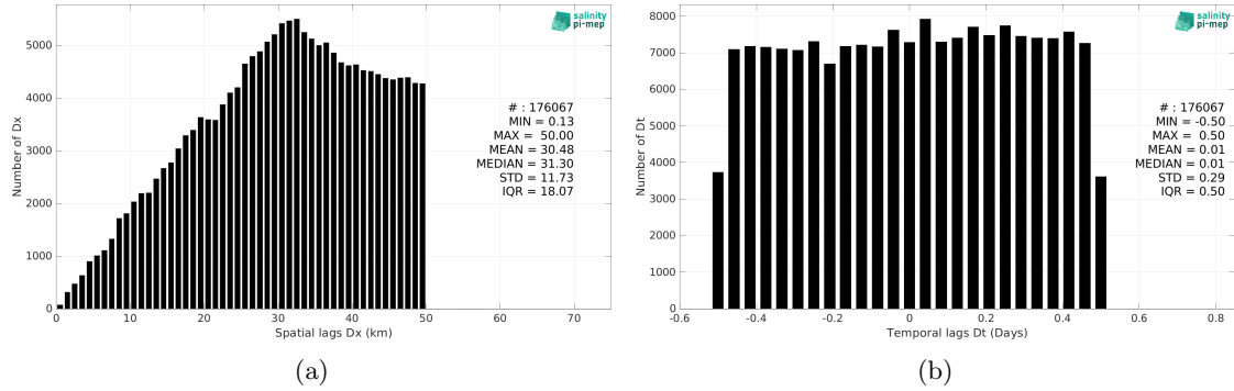
Figure 6: Histograms of the spatial (a) and temporal (b) lags between the location/time of the TSG (LEGOS-Survostral) measurement and the date of the corresponding Aquarius SSS L3 CAP v5 - 7-Day running (JPL) SSS pixel.
