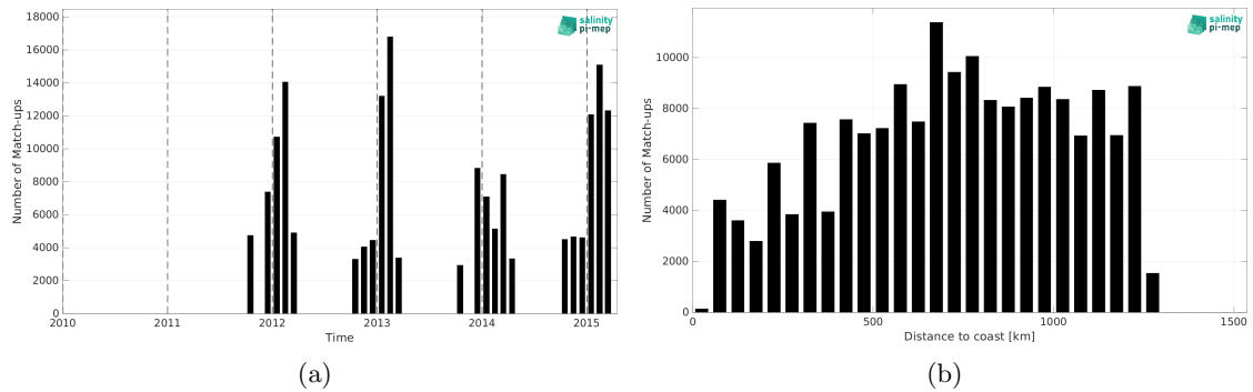
Figure 2: Number of match-ups between TSG (LEGOS-Survostral) and Aquarius SSS L3 CAP v5 - 7-Day running (JPL) SSS as a function of time (a) and as function of the distance to coast (b) over the Global Ocean Pi-MEP region and for the full satellite product period.
