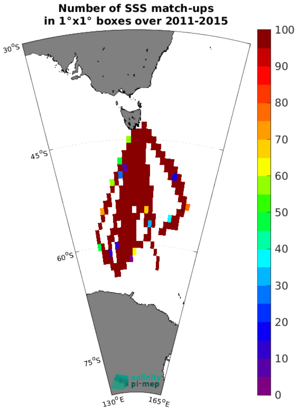
Figure 5: Number of SSS match-ups between TSG (LEGOS-Survostral) SSS and the Aquarius SSS L3 CAP v5 - 7-Day running (JPL) SSS product for the Global Ocean Pi-MEP region over 1^\circ \times 1^\circ boxes and for the full satellite product period.
