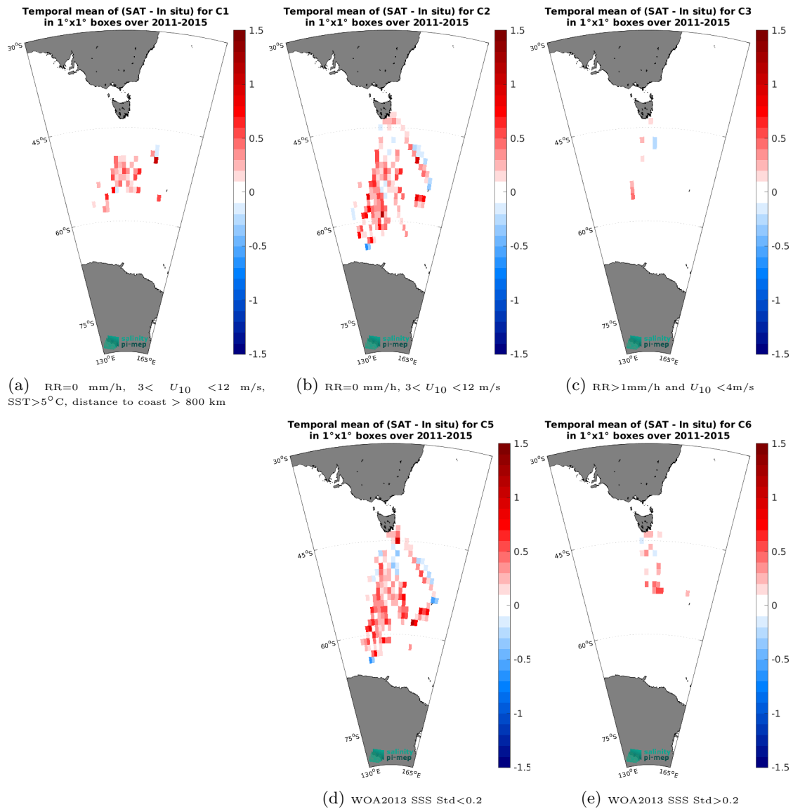
Figure 14: Temporal mean gridded over spatial boxes of size 1^\circ \times 1^\circ of \Delta SSS (Aquarius SSS L3 CAP v5 - 7-Day running (JPL) - TSG (LEGOS-Survostral)) for 5 different subdatasets corresponding to:RR=0 mm/h, 3 < U_{10} < 12 m/s, SST>5°C, distance to coast > 800 km (a), RR=0 mm/h, 3 < U_{10} < 12 m/s (b), RR>1mm/h and U_{10} < 4 m/s (c), WOA2013 SSS Std<0.2 (d), WOA2013 SSS Std>0.2 (e).
