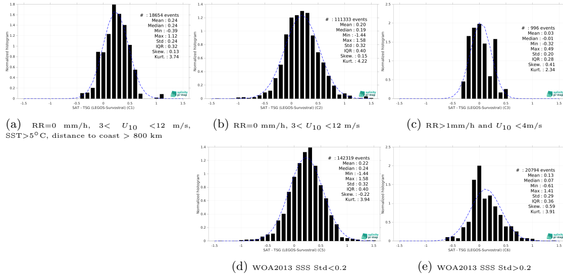
Figure 15: Normalized histogram of \Delta SSS (Aquarius SSS L3 CAP v5 - 7-Day running (JPL) - TSG (LEGOS-Survostral)) for 5 different subdatasets corresponding to: RR=0 mm/h, 3 < U_{10} < 12 m/s, SST>5°C, distance to coast > 800 km (a), RR=0 mm/h, 3 < U_{10} < 12 m/s (b), RR>1mm/h and U_{10} < 4 m/s (c), WOA2013 SSS Std<0.2 (d), WOA2013 SSS Std>0.2 (e).
