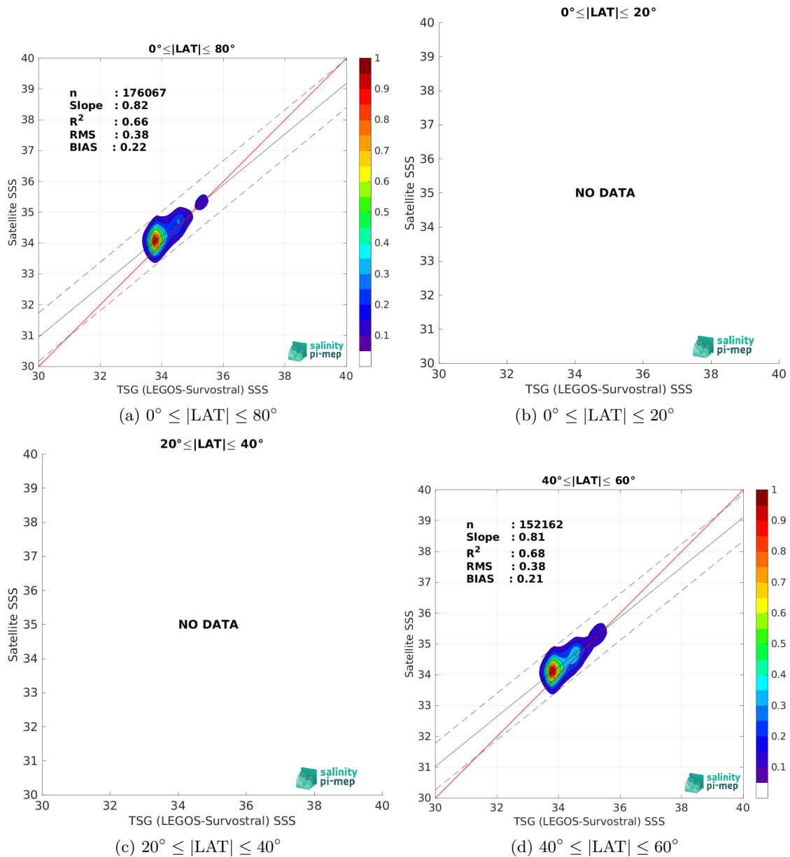
Figure 10: Contour maps of the concentration of Aquarius SSS L3 CAP v5 - 7-Day running (JPL) SSS (y-axis) versus TSG (LEGOS-Survostral) SSS (x-axis) at match-up pairs for different latitude bands. For each plot, the red line shows x=y . The black thin and dashed lines indicate a linear fit through the data cloud and the \pm 95\% confidence levels, respectively. The number match-up pairs n , the slope and R^2 coefficient of the linear fit, the root mean square (RMS) and the mean bias between satellite and in situ data are indicated for each latitude band in each plots.
