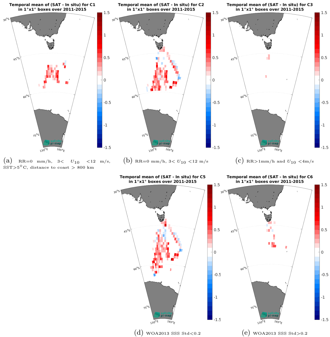
Figure 12: Temporal mean gridded over spatial boxes of size 1^\circ \times 1^\circ of \Delta SSS (Aquarius SSS L3 CAP v5 - 7-Day running (JPL) - TSG (LEGOS-Survostral)) for 5 different subdatasets corresponding to:RR=0 mm/h, 3 < U_{10} < 12 m/s, SST>5°C, distance to coast > 800 km (a), RR=0 mm/h, 3 < U_{10} < 12 m/s (b), RR>1mm/h and U_{10} < 4 m/s (c), WOA2013 SSS Std<0.2 (d), WOA2013 SSS Std>0.2 (e).
