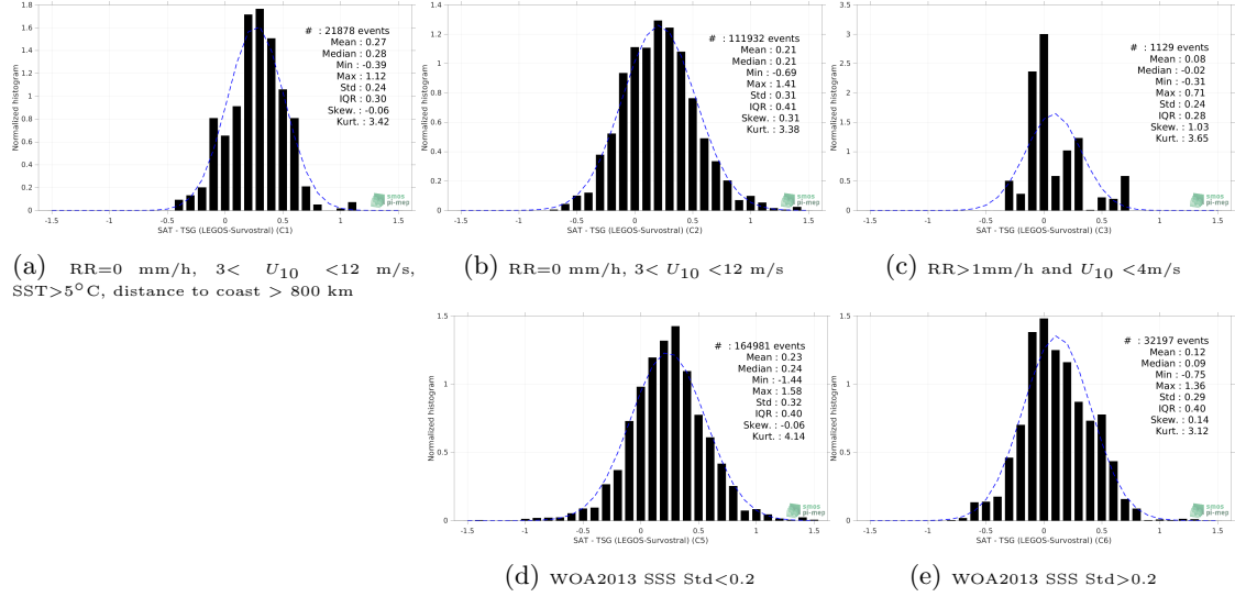
Figure 13: Normalized histogram of \Delta SSS (Aquarius SSS L3 CAP v5 - 7-Day running (JPL) - TSG (LEGOS-Survostral)) for 5 different subdatasets corresponding to: RR=0 mm/h, 3 < U_{10} < 12 m/s, SST > 5°C, distance to coast > 800 km (a), RR=0 mm/h, 3 < U_{10} < 12 m/s (b), RR > 1mm/h and U_{10} < 4 m/s (c), WOA2013 SSS Std < 0.2 (d), WOA2013 SSS Std > 0.2 (e).
