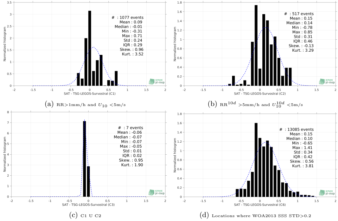
Figure 13: Normalized histogram of \Delta SSS (Aquarius-L3-JPL-V5-7DAY-RUNNING - TSG-LEGOS-Survostral) for 6 different subdatasets corresponding to: RR > 1mm/h and U_{10} < 5 m/s (a), RR^{10d} > 5 mm/h and U_{10}^{10d} < 5 m/s (b), C1 U C2 (c), Locations where WOA2013 SSS STD > 0.2 (d).
