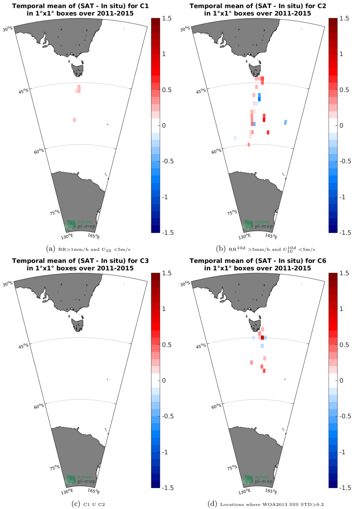
Figure 12: Temporal mean gridded over spatial boxes of size 1^\circ \times 1^\circ of \Delta SSS (Aquarius-L3-JPL-V5-7DAY-RUNNING - TSG-LEGOS-Survostral) for 4 different subdatasets corresponding to: RR > 1\text{mm/h} and U_{10} < 5\text{m/s} (a), RR^{10d} > 5\text{mm/h} and U_{10}^{10d} < 5\text{m/s} (b), C1 U C2 (c), Locations where WOA2013 SSS STD > 0.2 (d).
