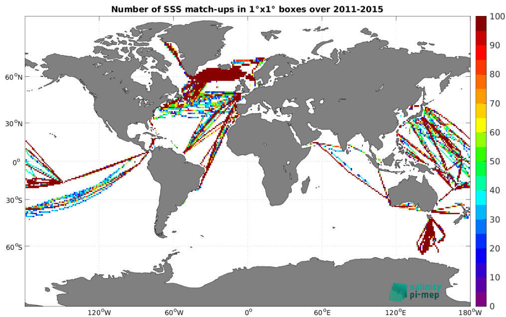
Figure 5: Number of SSS match-ups between TSG (LEGOS-DM) SSS and the Aquarius SSS L3 CAP v5 - 7-Day running (JPL) SSS product for the Global Ocean Pi-MEP region over 1^\circ \times 1^\circ boxes and for the full satellite product period.
