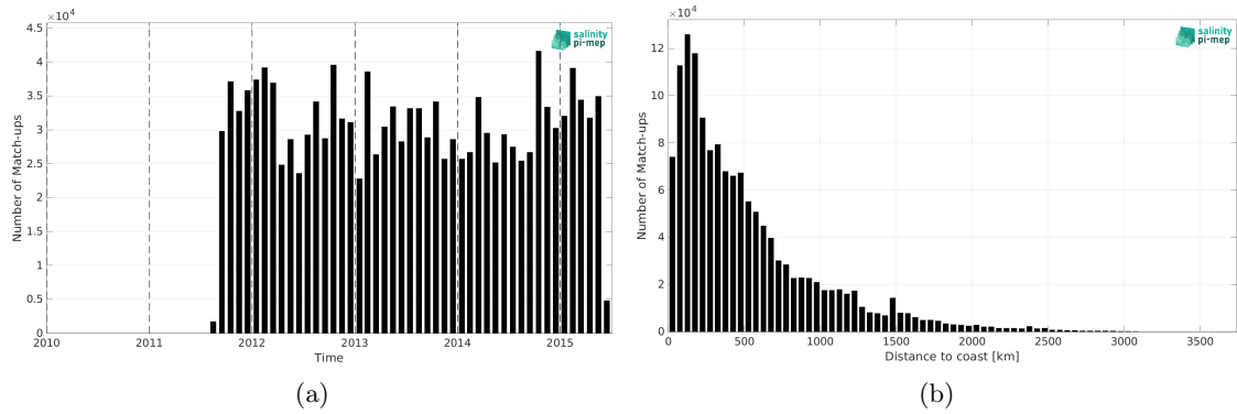
Figure 2: Number of match-ups between TSG (LEGOS-DM) and Aquarius SSS L3 CAP v5 - 7-Day running (JPL) SSS as a function of time (a) and as function of the distance to coast (b) over the Global Ocean Pi-MEP region and for the full satellite product period.
