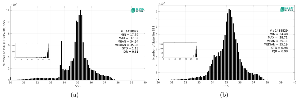
Figure 3: Histograms of SSS from TSG (LEGOS-DM) (a) and Aquarius SSS L3 CAP v5 - 7-Day running (JPL) (b) considering all match-up pairs per bins of 0.1 over the Global Ocean Pi-MEP region and for the full satellite product period.
