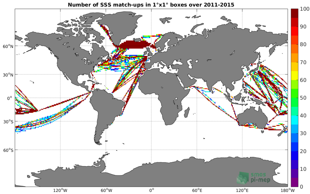
Figure 4: Number of SSS match-ups between TSG-LEGOS-DM SSS and the Aquarius-L3-JPL-V5-7DAY-RUNNING SSS product for the Global Ocean Pi-MEP region over 1°x1° boxes and for the full satellite product period.
