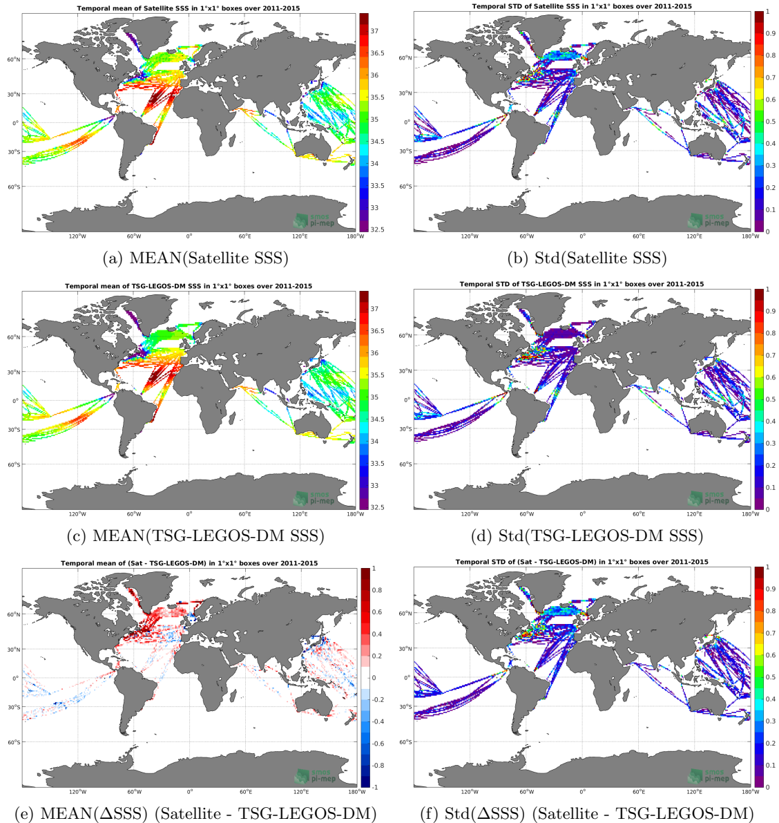
Figure 6: Temporal mean (left) and Std (right) of SSS from Aquarius-L3-JPL-V5-7DAY-RUNNING (top), TSG-LEGOS-DM (middle), and of \Delta SSS (Satellite - TSG-LEGOS-DM). Only match-up pairs are used to generate these maps.
