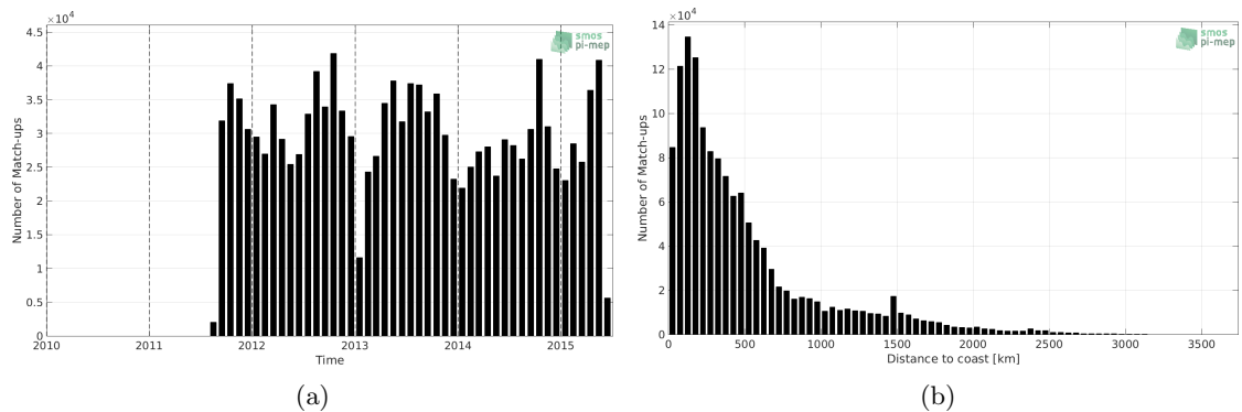
Figure 1: Number of match-ups between TSG-LEGOS-DM and Aquarius-L3-JPL-V5-7DAY-RUNNING SSS as a function of time (a) and as function of the distance to coast (b) over the Global Ocean Pi-MEP region and for the full satellite product period.
