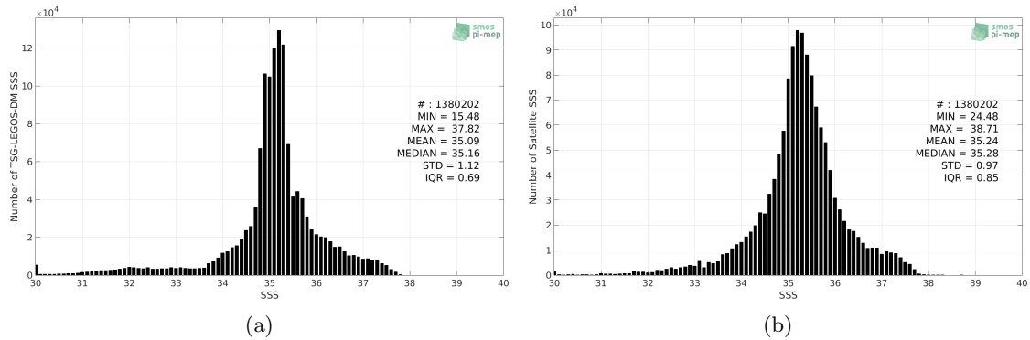
Figure 2: Histograms of SSS from TSG-LEGOS-DM (a) and Aquarius-L3-JPL-V5-7DAY-RUNNING (b) considering all match-up pairs per bins of 0.1 over the Global Ocean Pi-MEP region and for the full satellite product period.
