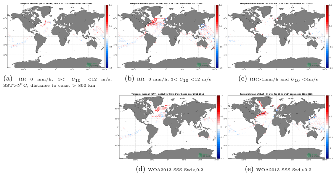
Figure 12: Temporal mean gridded over spatial boxes of size 1^\circ \times 1^\circ of \Delta SSS (Aquarius-L3-JPL-V5-7DAY-RUNNING - TSG-LEGOS-DM) for 5 different subdatasets corresponding to:RR=0 mm/h, 3 < U_{10} < 12 m/s, SST > 5^\circ\text{C} , distance to coast > 800 km (a), RR=0 mm/h, 3 < U_{10} < 12 m/s (b), RR > 1 mm/h and U_{10} < 4 m/s (c), WOA2013 SSS Std < 0.2 (d), WOA2013 SSS Std > 0.2 (e).
