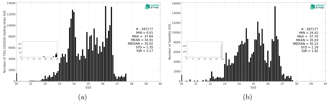
Figure 3: Histograms of SSS from TSG (GOSUD-Sailing-ship) (a) and Aquarius SSS L3 CAP v5 - 7-Day running (JPL) (b) considering all match-up pairs per bins of 0.1 over the Global Ocean Pi-MEP region and for the full satellite product period.
