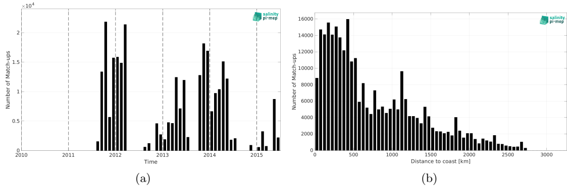
Figure 2: Number of match-ups between TSG (GOSUD-Sailing-ship) and Aquarius SSS L3 CAP v5 - 7-Day running (JPL) SSS as a function of time (a) and as function of the distance to coast (b) over the Global Ocean Pi-MEP region and for the full satellite product period.
