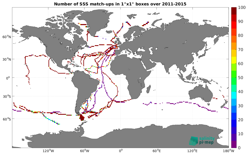
Figure 5: Number of SSS match-ups between TSG (GOSUD-Sailing-ship) SSS and the Aquarius SSS L3 CAP v5 - 7-Day running (JPL) SSS product for the Global Ocean Pi-MEP region over 1^\circ \times 1^\circ boxes and for the full satellite product period.
