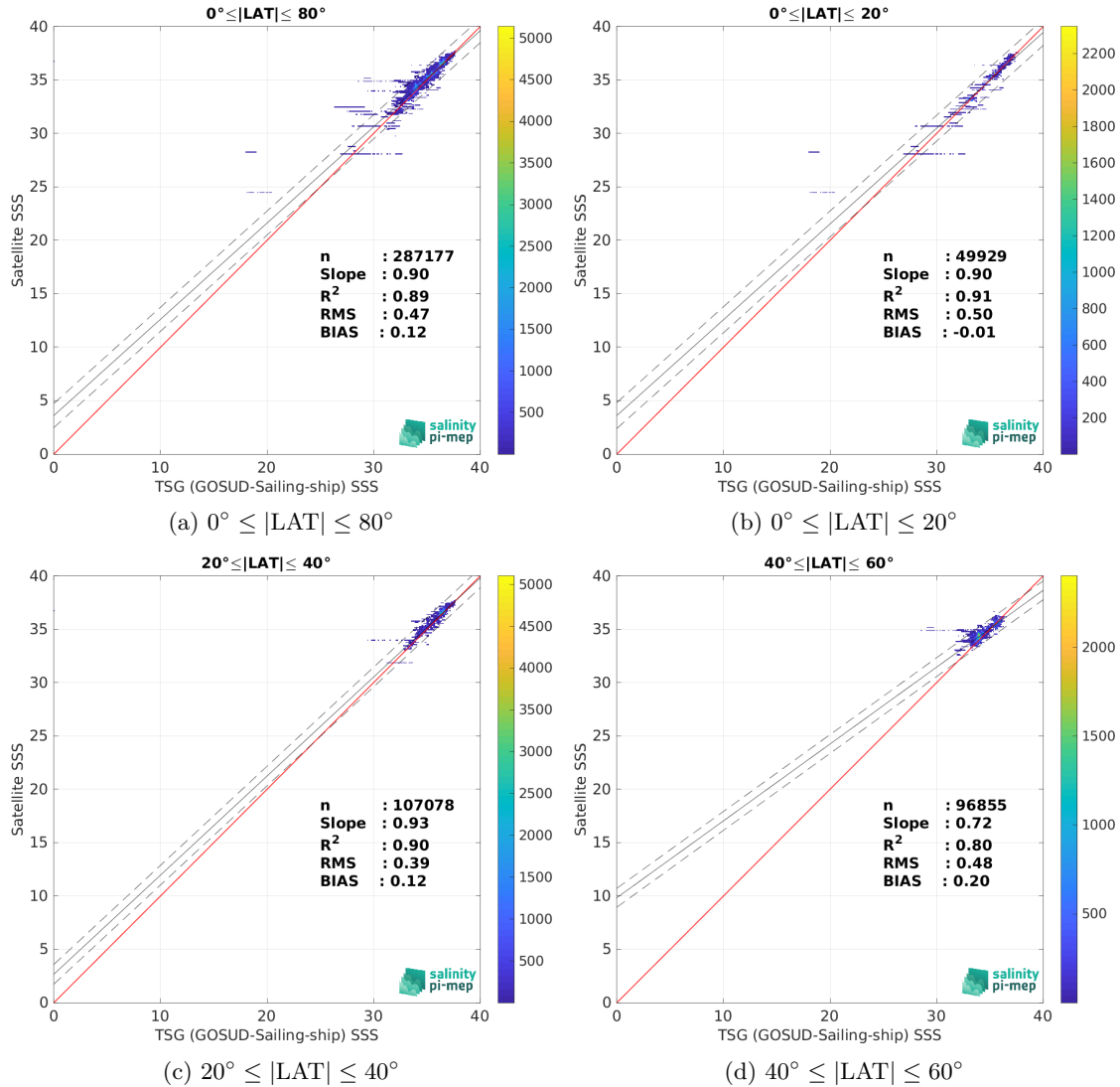
Figure 10: Contour maps of the concentration of Aquarius SSS L3 CAP v5 - 7-Day running (JPL) SSS (y-axis) versus TSG (GOSUD-Sailing-ship) SSS (x-axis) at match-up pairs for different latitude bands. For each plot, the red line shows x=y . The black thin and dashed lines indicate a linear fit through the data cloud and the \pm 95\% confidence levels, respectively. The number of match-up pairs n , the slope and R^2 coefficient of the linear fit, the root mean square (RMS) and the mean bias between satellite and in situ data are indicated for each latitude band in each plot.
