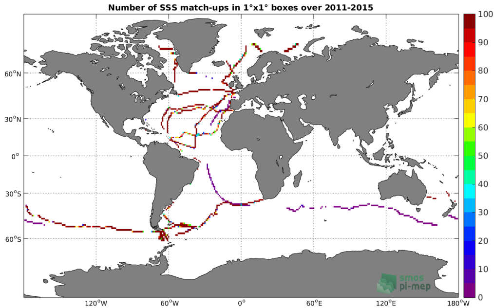
Figure 4: Number of SSS match-ups between TSG-GOSUD-Sailing-ship SSS and the Aquarius-L3-JPL-V5-7DAY-RUNNING SSS product for the Global Ocean Pi-MEP region over 1°x1° boxes and for the full satellite product period.
