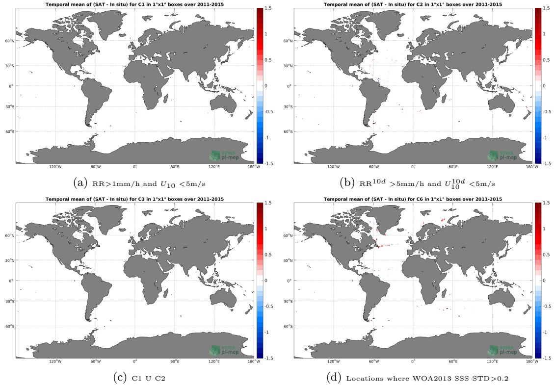
Figure 12: Temporal mean gridded over spatial boxes of size 1^\circ \times 1^\circ of \Delta SSS (Aquarius-L3-JPL-V5-7DAY-RUNNING - TSG-GOSUD-Sailing-ship) for 4 different subdatasets corresponding to: RR > 1\text{mm/h} and U_{10} < 5\text{m/s} (a), RR^{10d} > 5\text{mm/h} and U_{10}^{10d} < 5\text{m/s} (b), C1 U C2 (c), Locations where WOA2013 SSS STD > 0.2 (d).
